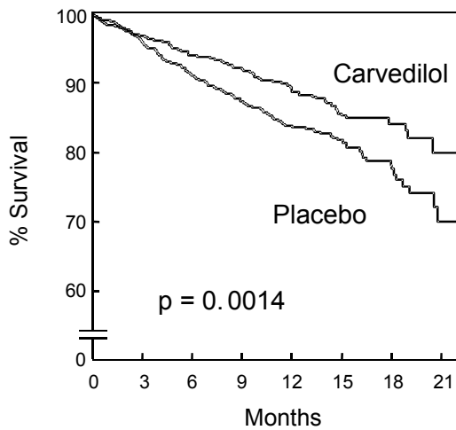
1 Figure 1. Survival Analysis for COPERNICUS (intent-to-treat)
