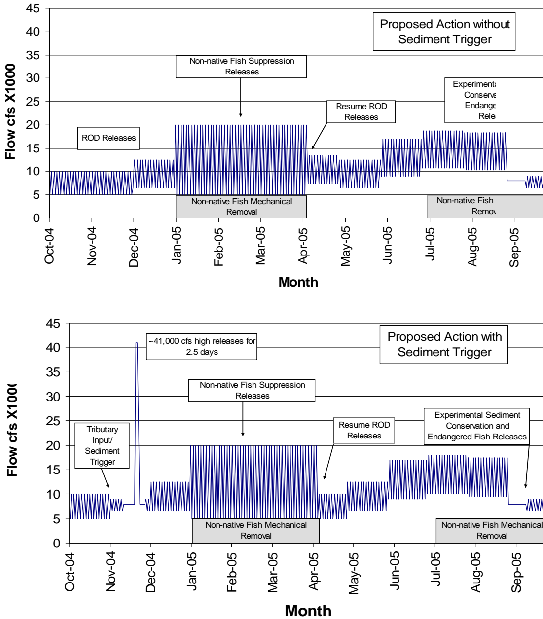
Figure 2. Proposed Action scenario without and with a sediment trigger sufficient to trigger a high experimental flow from Glen Canyon Dam.
