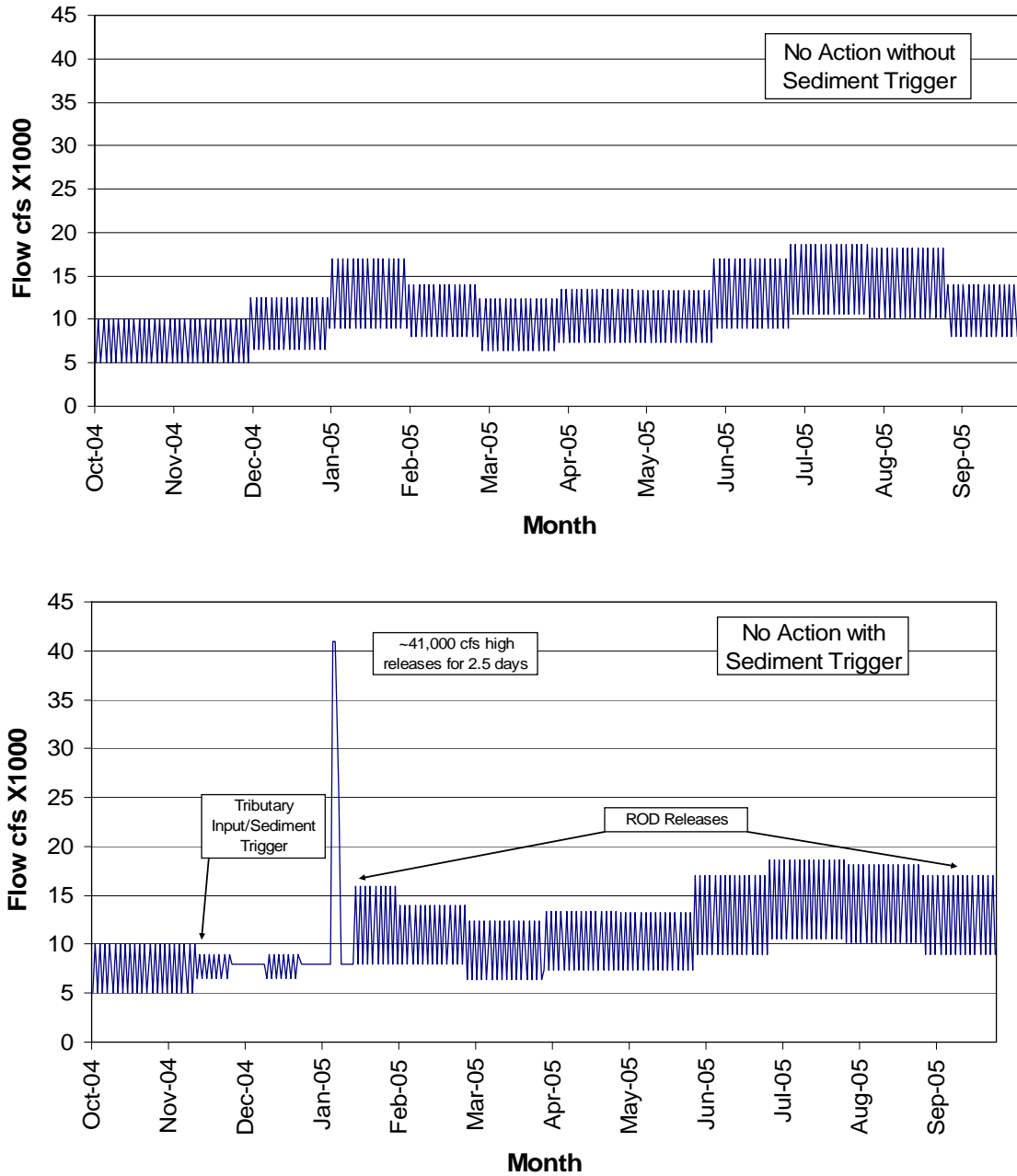
Figure 1. No Action scenario without and with a sediment trigger sufficient to trigger a high experimental flow from Glen Canyon Dam.
