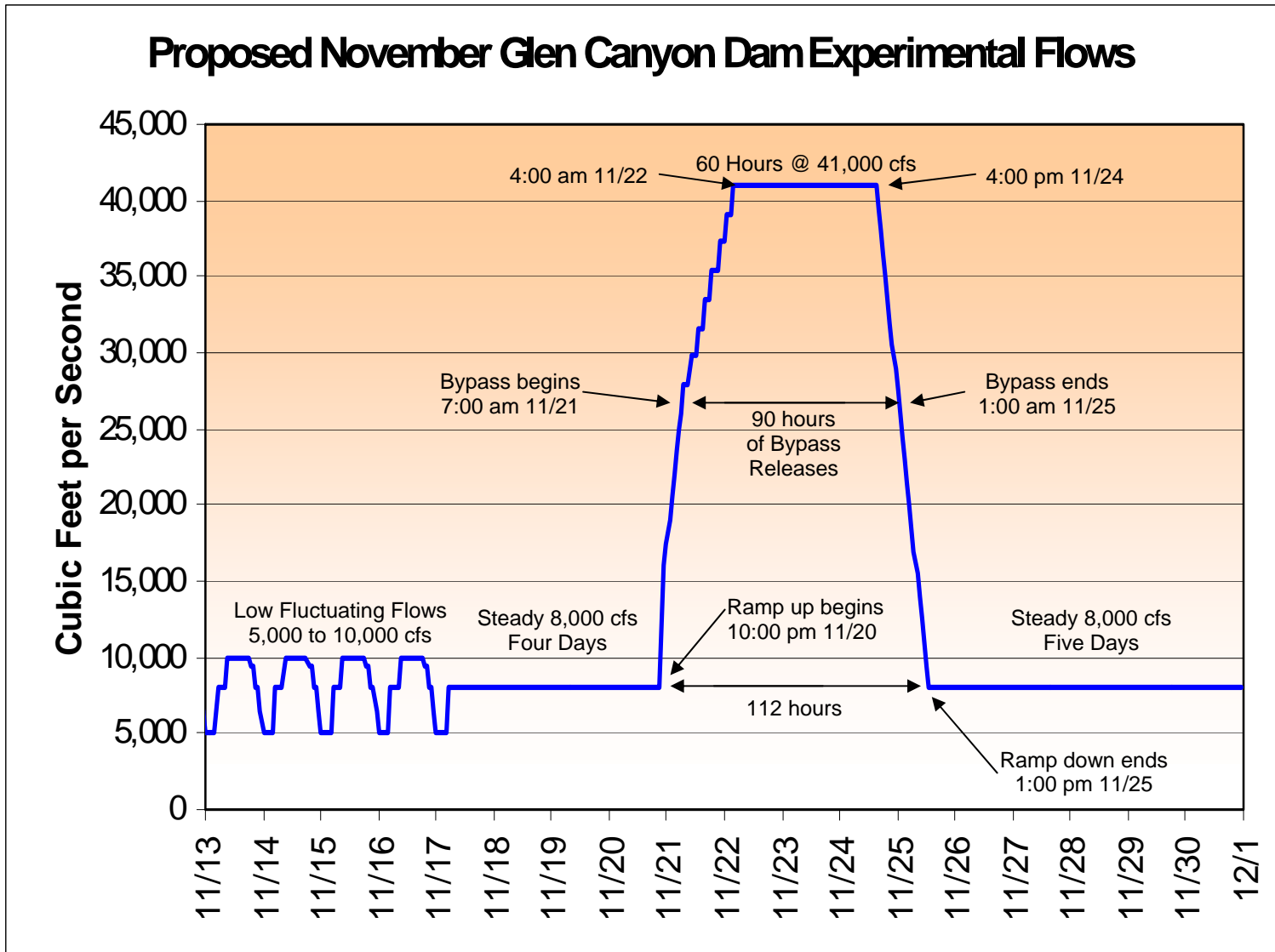
Figure 3. Detailed portrayal of the proposed high experimental flow.
