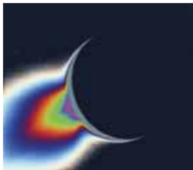
Backlit by the Sun, Saturn's moon Enceladus has a fountain-like plume of icy material that towers over the moon's south polar region. The greatly enhanced and colorized image, taken by the Cassini spacecraft during a July 2005 flyby, shows the extent of the fainter, larger-scale component of the plume. Scientists suspect that the plume is created by multiple jets arising from warm fractures in the region, indicating that the small moon is geologically active. (Image: NASA/JPL/Space Science Institute)
