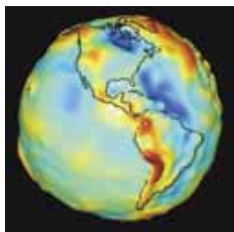
This image was created using gravity field data from the Gravity Recovery And Climate Experiment (GRACE) twin satellites, launched in 2002, which study changes to Earth's gravitational fields over both land and sea. Red indicates the strongest gravity field; blue indicates the weakest. (Image: NASA)
