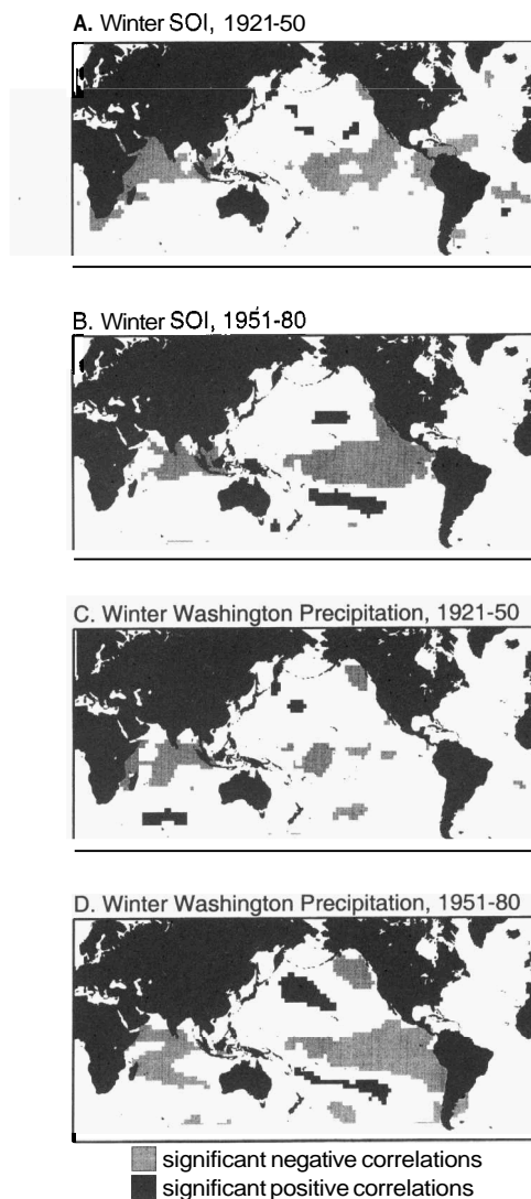
Figure 7. Correlations (significant at a 95% confidence level) between winter (October–March) SSTs (Parker et al. , 1995) and the October–March SOI for (A) 1921–1950 and (B) 1951–1980, and between winter SSTs and October–March precipitation for Washington for (C) 1921–1950 and (D) 1951–1980
