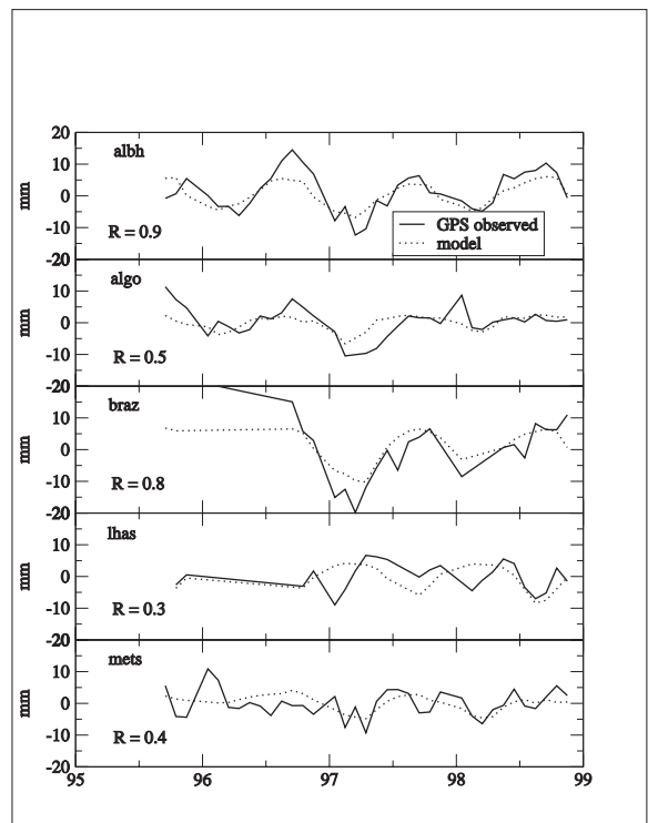
Figure 2. Modeled maximum water-storage-induced vertical displacements ( \Delta r_M , mm) at selected GPS locations (dotted lines) and monthly averages of GPS height residuals ( \Delta r_O , mm) after atmospheric pressure and nontidal and tidal annually varying loading corrections (solid lines). Victoria (albh), in Western Canada; Algonquin Park (algo), in Eastern Canada; Brasilia, Brazil (braz); Lhasa, China (lhas) on the Tibetan Plateau; and Kirkkonummi, Finland (mets). The R values represent the amplitudes of the correlations between the two signals.
