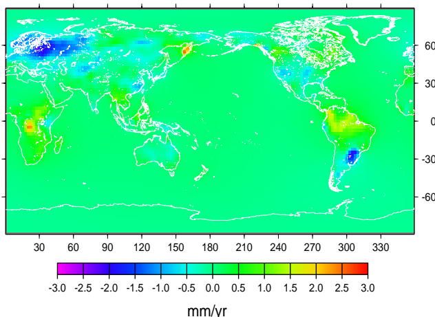
Figure 4. Global distribution of vertical displacement rates ( \text{mm/yr} ) modeled using 3 years (1996-1998) of water-storage data.
