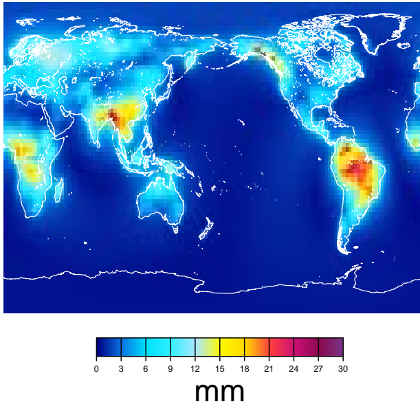
Figure 1. Maximum range in vertical crustal displacement during 1994-1998 (mm) due to changes in total continental water storage.
