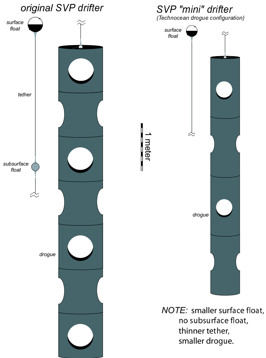
Figure 1: Schematic view of two SVP drifter types. All components are shown to scale; much of the tether length has been excluded. The drogues are centered at a depth of 15m.
