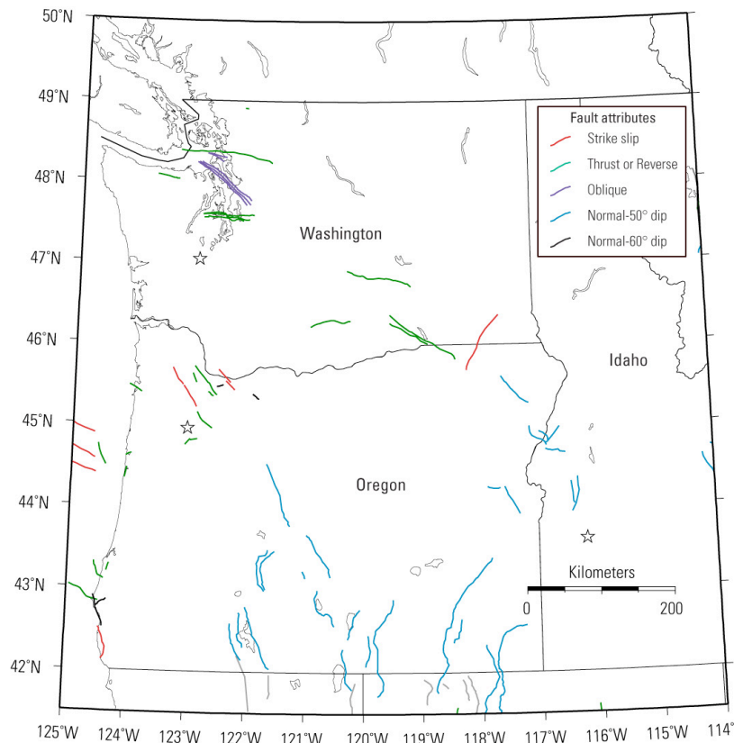
Figure H-1. Map of fault sources in the Pacific Northwest showing sense of slip by color.
