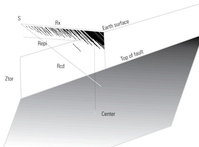
Figure D-1. Schematic diagram of virtual fault with associated distances to site S. Rcd, closest distance to fault; Rx, closest distance to top of fault projected indefinitely along strike; Rx < 0 on footwall (Rx is used in the Chiou and Youngs relation); Repi, picentral distance to center projected to Earth surface; Ztor, depth of top of rupture, and \theta is fault strike, a random variable.
