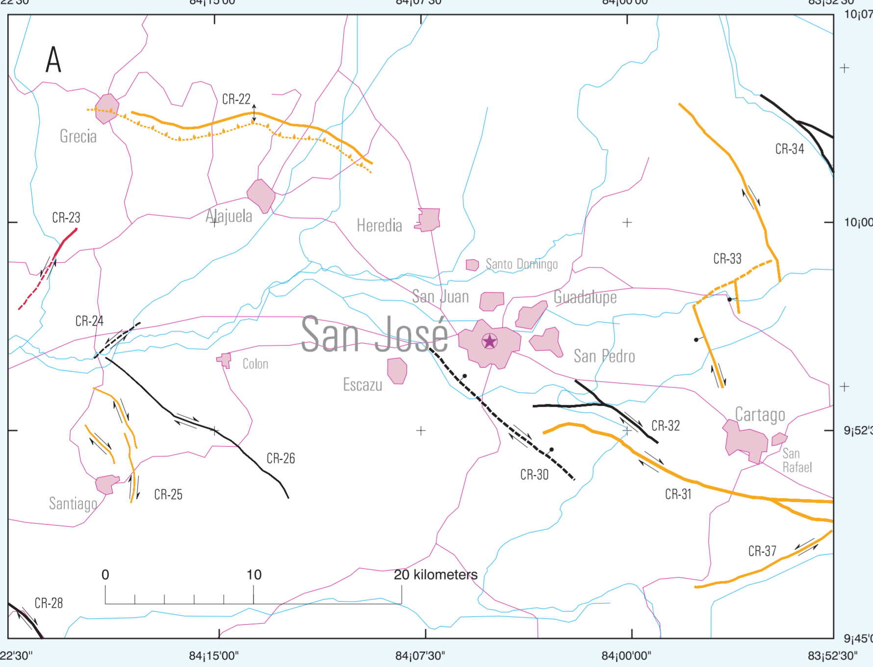
Map of Quaternary Faults and Folds of Costa Rica A project of International Lithosphere Program Task Group II-2, Major Active Faults of the World A cooperative project between the U.S. Geological Survey, the Central American School of Geology—Universidad de Costa Rica and the Costa Rican Electrical Institute, San Jose, Costa Rica Data compiled by Walter Montero, Percy Denyer, Rafael Barquero, Guillermo Alvarado, and Hugh Cowan; digital representation by Richard L. Dart; and project coordinated by Michael N. Machette (ILP Task Group II-2 Co-chairman)
