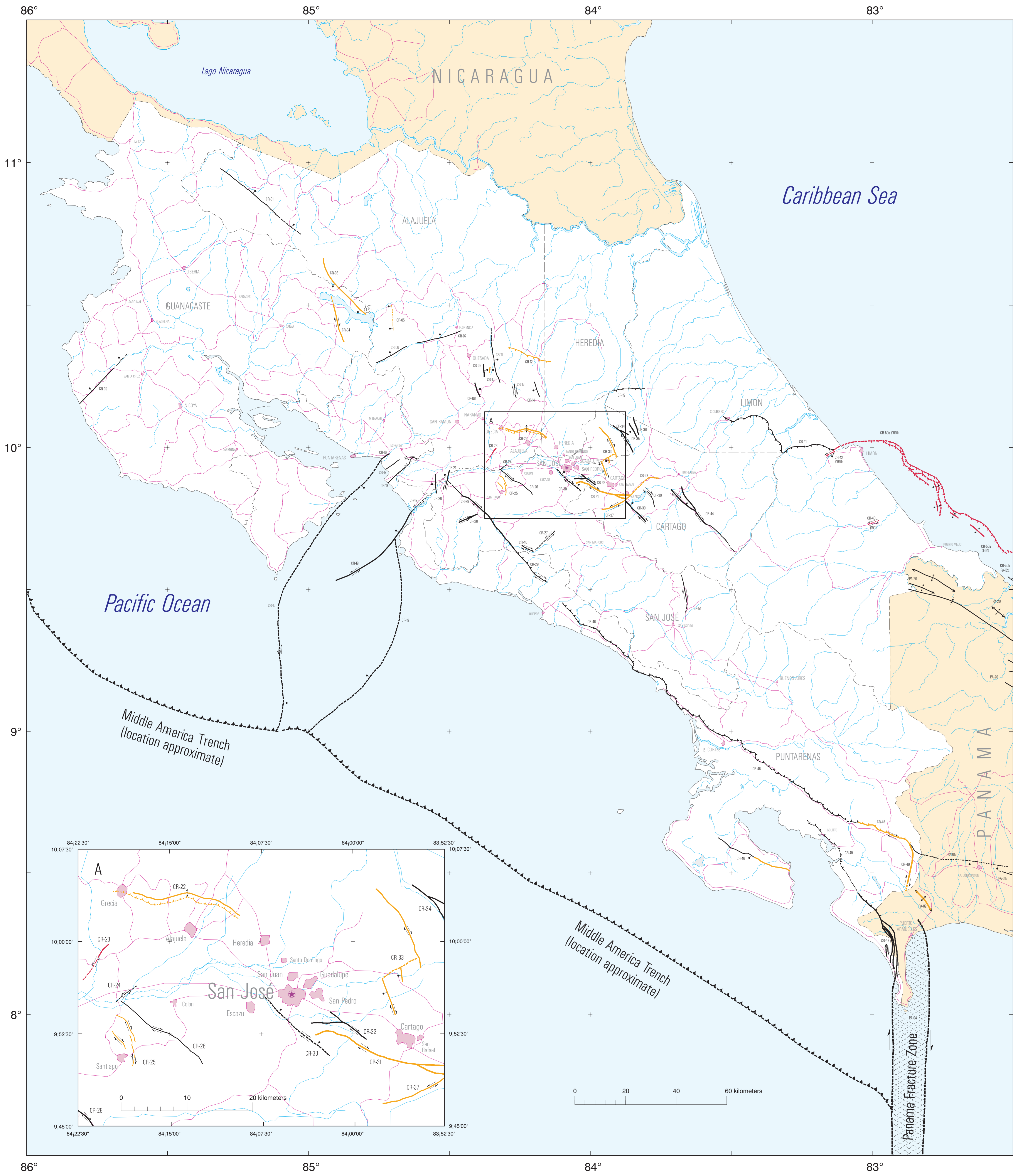
Map of Quaternary Faults and Folds of Costa Rica A project of International Lithosphere Program Task Group II-2, Major Active Faults of the World A cooperative project between the U.S. Geological Survey, the Central American School of Geology—Universidad de Costa Rica and the Costa Rican Electrical Institute, San Jose, Costa Rica Data compiled by Walter Montero, Percy Denyer, Rafael Barquero, Guillermo Alvarado, and Hugh Cowan; digital representation by Richard L. Dart; and project coordinated by Michael N. Machette (ILP Task Group II-2 Co-chairman)
