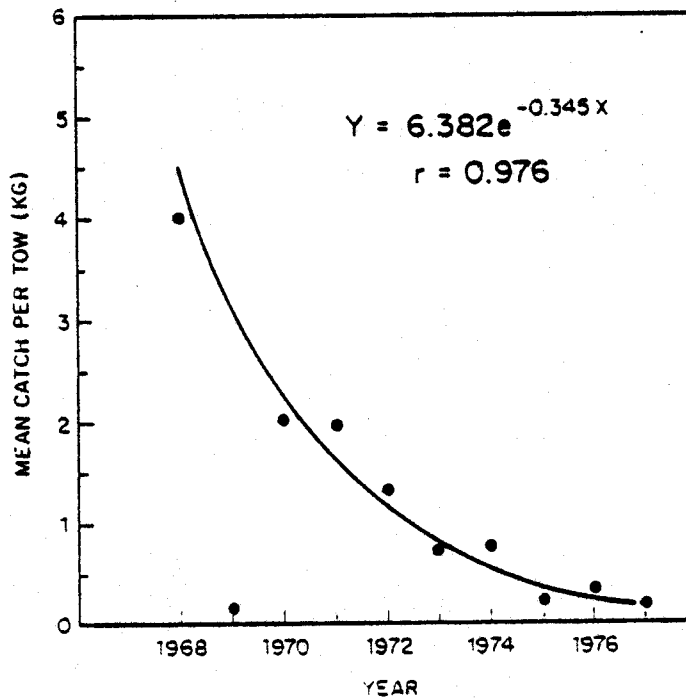
Figure 5. Exponential curve fitted to the 1968-1977 (1969 value omitted from calculation) catch-per-tow values for mackerel (retransformed) from the USA spring bottom trawl survey.
