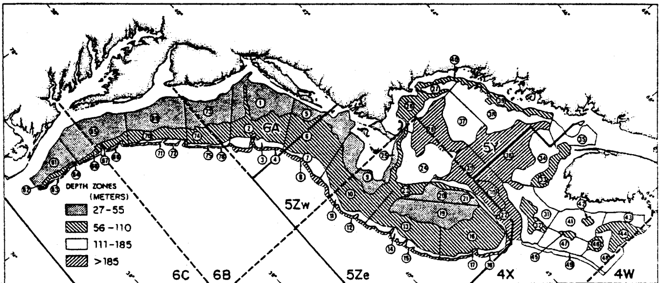
Figure 2. USA bottom trawl survey sampling strata in the Northwest Atlantic between Cape Hatteras and Nova Scotia.
