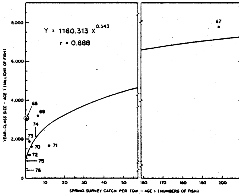
Figure 8. Power curve relationship between mackerel year-class size at age 1 from cohort analysis assuming F = 0.36 at ages 4 and older in 1977 and spring survey catch per tow at age 1 (1968 value omitted from calculation).
