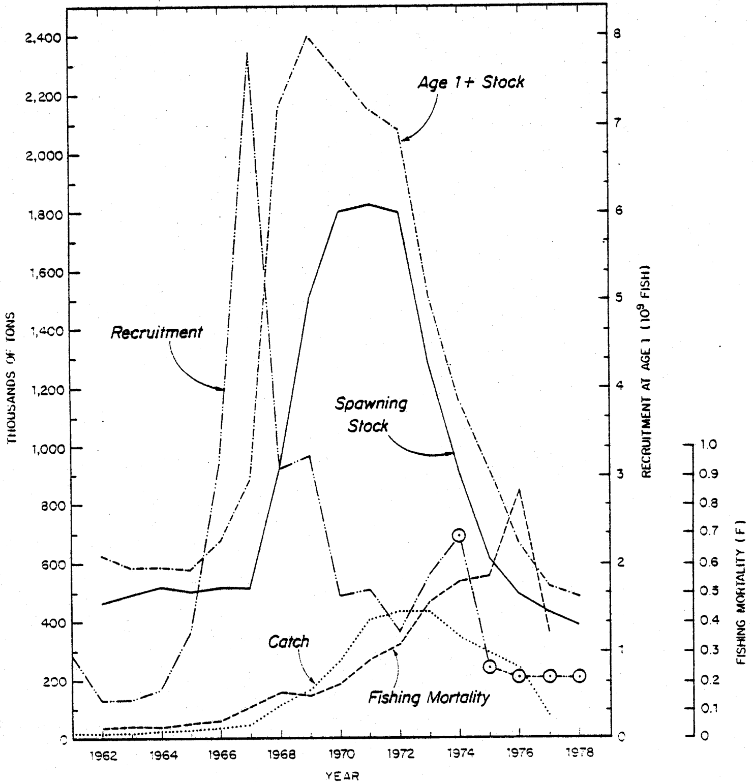
Figure 12. Mackerel stock biomass (ages 1 and older and spawners) during 1962-1978 from cohort analysis assuming F = 0.36 at ages 4 and older in 1977, abundance at age 1 of the 1961-1977 year classes (open circles represent estimated year-class sizes; others determined from cohort analysis), total international catch (commercial and recreational) during 1961-1977, and fishing mortality (mean for ages 3 and older) during 1962-1977 in ICNAF SA 3-6.
