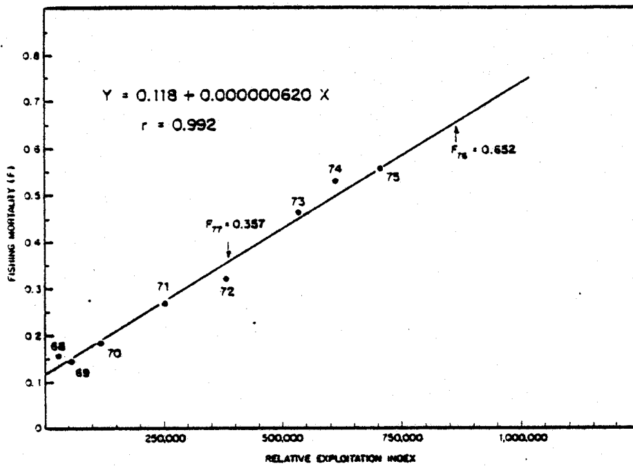
Figure 6. Relationship between fishing mortality from cohort analysis assuming F = 0.36 at ages 4 and older in 1977 and a relative exploitation index derived from USA spring survey catch per tow and total catch of mackerel.
