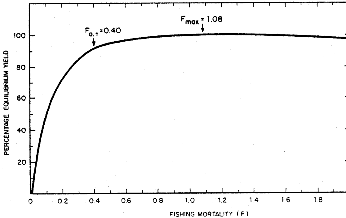
Figure 11. Curve of equilibrium yield for mackerel (see text for parameters), with yield expressed as a percentage of the maximum.
