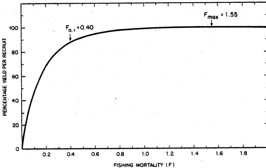
Figure 10. Beverton and Holt (1957) yield-per-recruit curve for mackerel (see text for parameters), with yield per recruit expressed as a percentage of the maximum.
