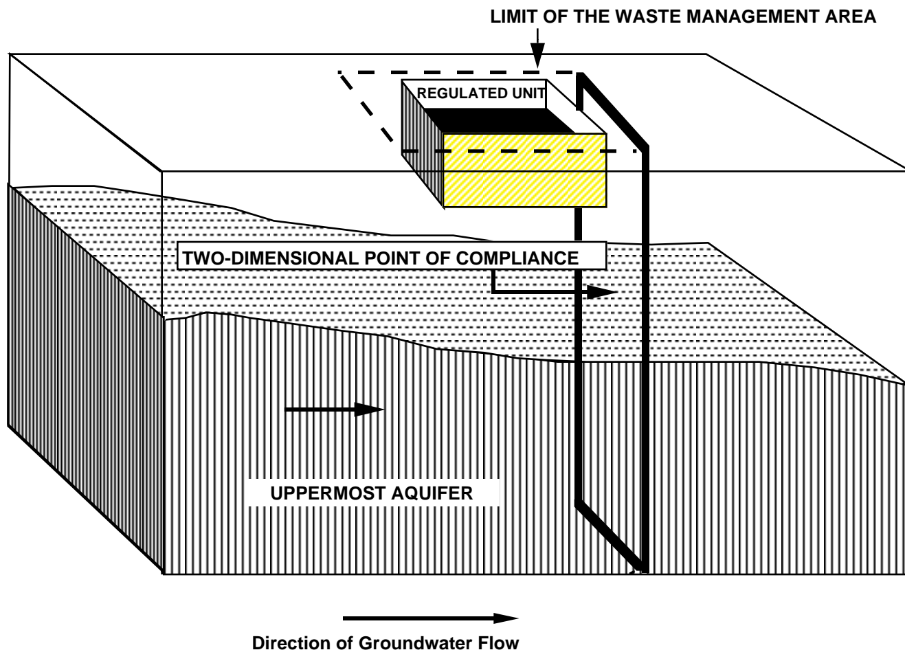
Figure 6 SCHEMATIC OF POINT OF COMPLIANCE
