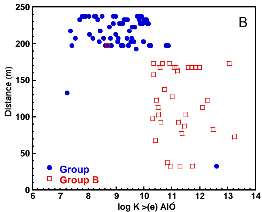
Figure 2.9 Breakthrough distance representing a C/C_0 \sim 0.5 of uranium in fluid versus (a) \log K_{>(e)AlOUO_2^+} and (b) \log K_{>(e)AlO} for a simulation time of two years. The various simulations are separated based on the two observed groups A and B.
