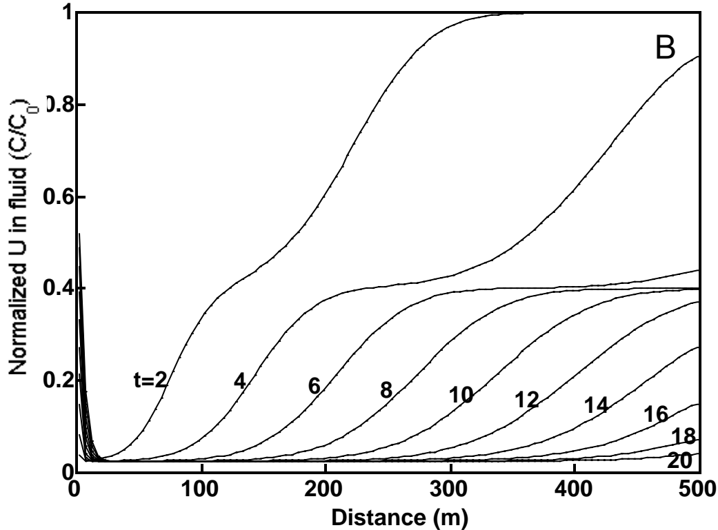
Figure 2.6 Temporal development of concentration profiles for aqueous uranium typical of (a) group A and (b) group B. Note that the log K values chosen for this Group A simulation result in a smaller fraction of uranium in solution than the baseline case illustrated in Fig. 2.2. simulations, the uranium present is more equally distributed between the solution and the smectite surface; for example, for \log K_{>(e)AlO^-} = 9.72 and \log K_{>(e)AlOUO_2^+} = -1.14 , the initial uranium concentrations are 560 mg/kg in solution and 490 mg/kg adsorbed.
