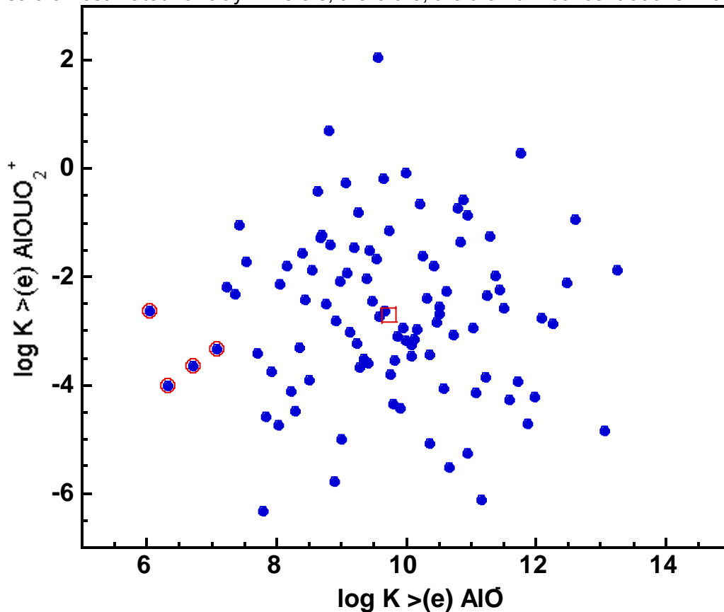
Figure 2.4 Log K variation for >(e)AlOUO_2^+ versus those of >(e)AlO^- for 100 pairs of values generated
