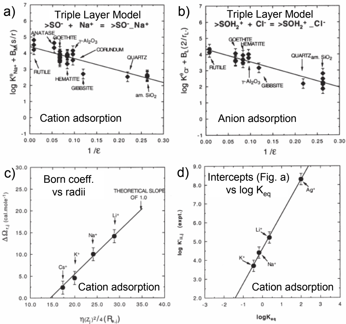
Figure 4.1 Correlations between adsorption constants and mineral properties. (a) Values of \log K_M^0 as a function of the dielectric constant \left(\frac{1}{\epsilon_s}\right) and values of the bond strength per Å \left(\frac{s}{r_M}\right) ; (b) values of \log K_L^0 as a function of the dielectric constant \left(\frac{1}{\epsilon_s}\right) and the repulsive term in Å \left(\frac{2}{r_L}\right) ; (c) values of \Delta\Omega_{r,M^+} as a function of the effective electrostatic radius \left(\frac{1}{R_{e,j}}\right) and values of r_{x,j} ; (d) linear free energy correlations for values of \log K_{i,M}^{(expt.)} with the aqueous phase equilibrium association constants \log K_{M(OH)^0} . Adapted from Sverjensky (2005) with permission from Elsevier.
