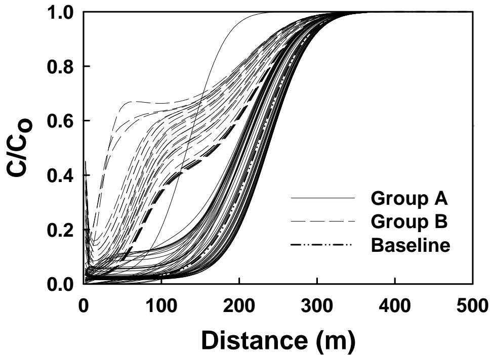
Figure 2.7 Normalized concentrations versus distance profiles of uranium in fluid versus distance, after 2 years, for 96 realizations. The profile for the baseline case (i.e., using mean log K values) is also indicated.
