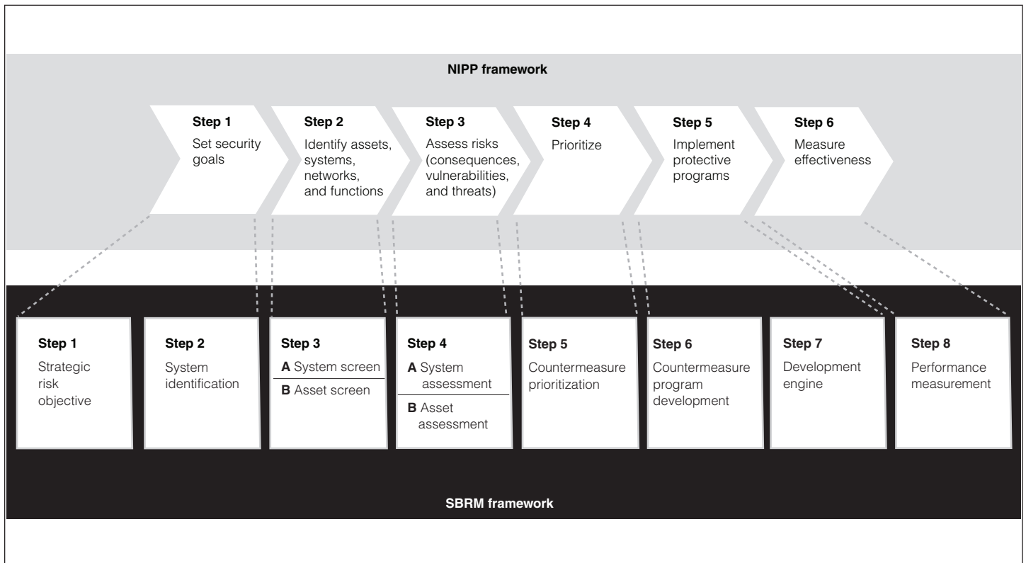
Figure 3: Alignment between the NIPP and TSA’s Systems-Based Risk Management Framework (SBRM)
