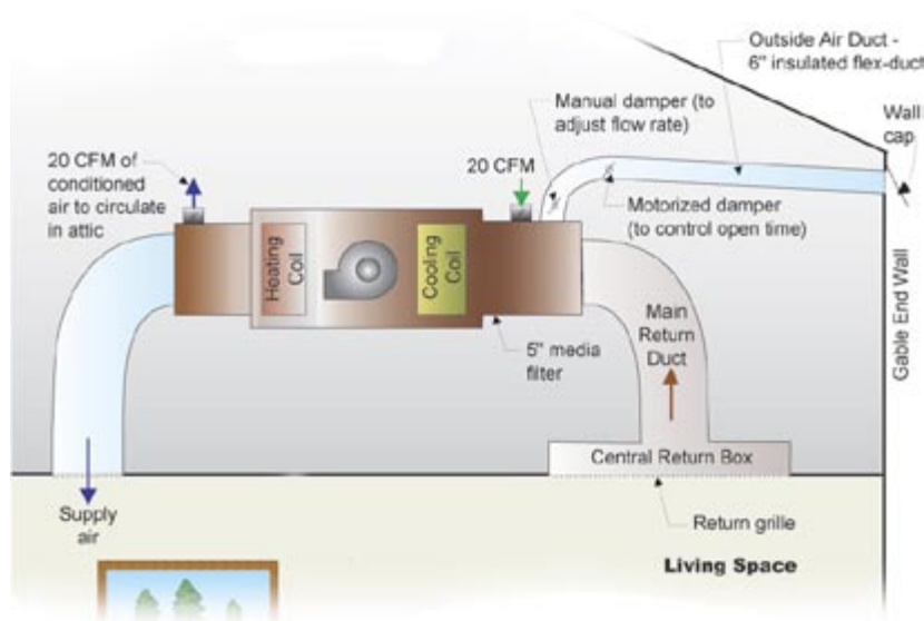
FIGURE 15: Outside Vents
