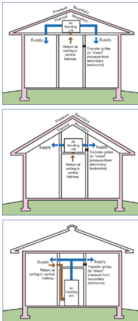
FIGURE 16: Duct Run Configurations
