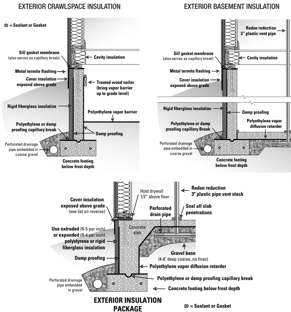
FIGURE 3: Typical Building Foundation Systems
