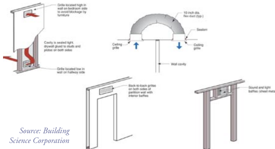
FIGURE 18: Approaches to Pressure Balancing
