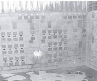
This is a view of the Black Cell Design during construction.
