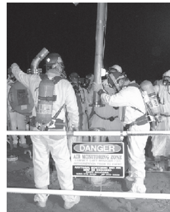
Hanford Tank Farm workers installing a breather stack extension.
