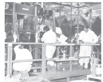
Glovebox operations at Nevada's Visual Examination and Repackaging Building.
