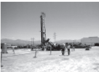
A Grout Rig will be used to Coat Blocks of Beryllium with a Wax-Based Grout to Reduce the Release of Carbon-14. The Grout will be Injected at approximately 8,200 Pounds per Square Inch at a Temperature of Nearly 400° F.
