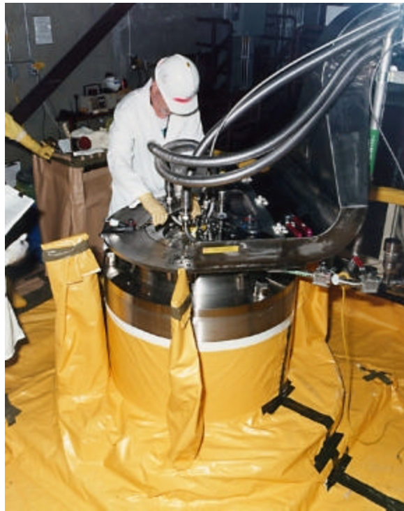
Cover Photograph: Nuclear Chemical Operators Attach Hoses to Ports in the Top of a Multi-Canister Overpack Holding 290-300 Irradiated Fuel Assemblies from Hanford's K-Basins, in the Cold Vacuum Drying Facility.
