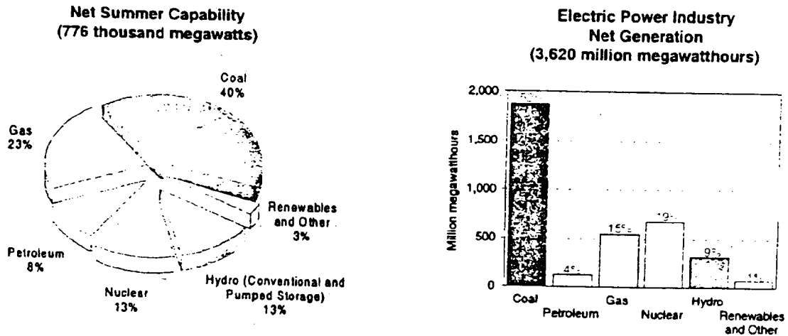
Figure 4. Electric Power Industry Capability and Generation by Energy Source, 1998
