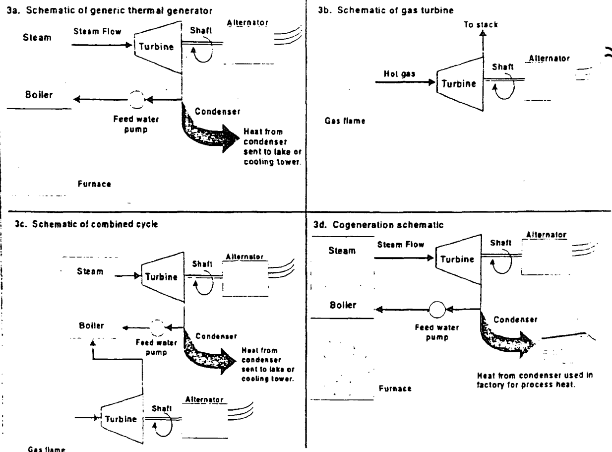
Figure 3. Prime Movers of Electricity
