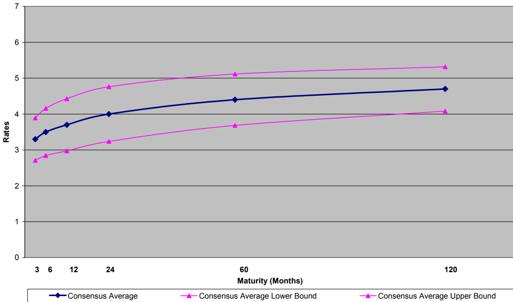
Figure 2: Estimated Yield Curve and Interval for Third Quarter 2005
