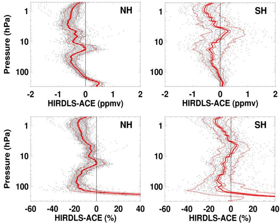
Figure 5.2.3. Shown is the ozone percent difference between HIRDLS and ACE-FTS satellite solar occultation comparisons since May 2006.
