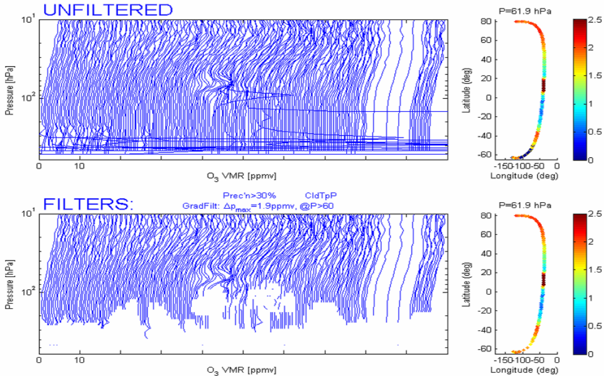
Figure 5.2.9. Shown are HIRDLS v003 ozone profiles for about \frac{1}{2} orbit on 2006-June-19. The top plot shows the raw unfiltered data and the bottom shows the filtered data using the three recommended filters.
