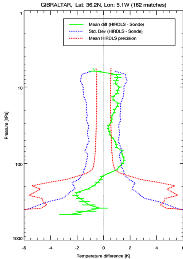
Figure 5.1.2. Statistics of HIRDLS minus sonde differences for Gibraltar. Green line shows mean differences, blue dots show \pm 1 standard deviation of the differences, while red dots show \pm 1 standard deviation predicted by retrieval algorithm.
