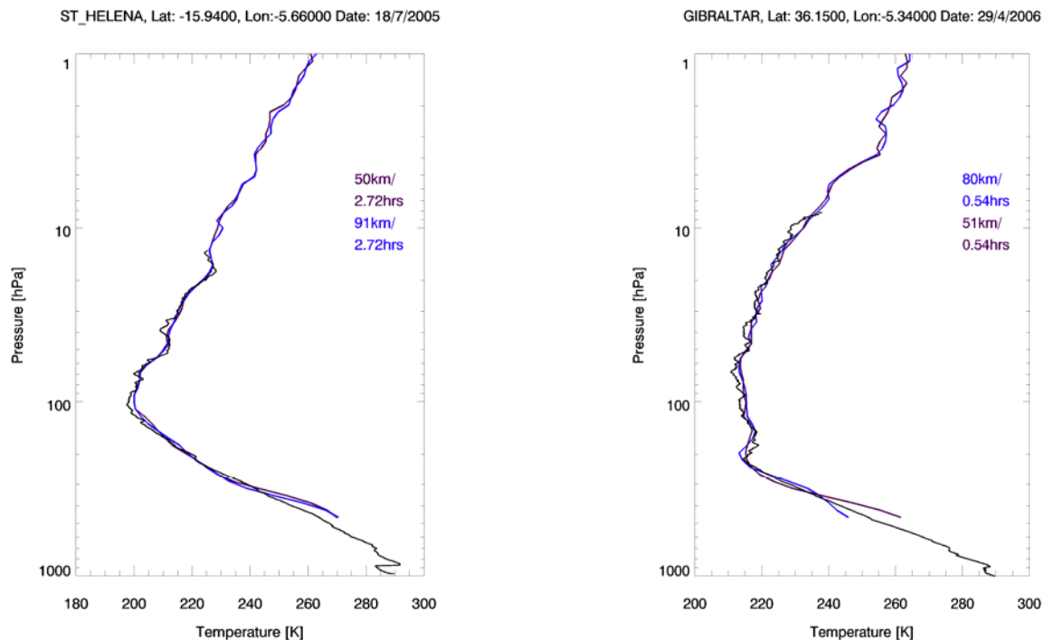
Figure 5.1.1. Temperature comparisons between radiosonde profiles at St. Helena (left) and Gibraltar. Black lines are high resolution radiosondes, blue and magenta are two nearby HIRDLS retrievals. Differences in distances and times are shown.
