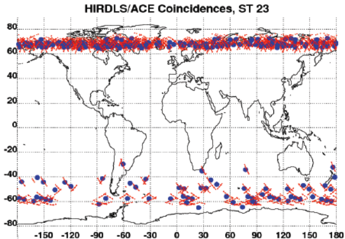
Figure 5.3.7. Latitude-longitude cross sections showing ACE-FTS HNO 3 measurement locations (blue) and HIRDLS HNO 3 measurement locations (red). Coincidences are defined as occurring within 2-hours in time and 500 km. The coincidences shown here are for scan table 23. There were a total of 150 coincidences between 19 May 2006 and 31 October 2006.
