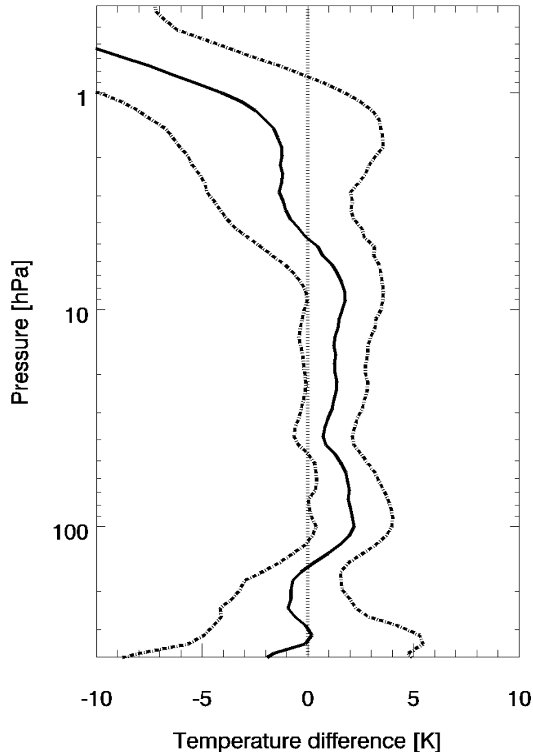
Figure 5.1.3 Results of comparison of HIRDLS temperatures with analyzed ECMWF temperatures interpolated to HIRDLS measurement locations over the full latitude range of HIRDLS observations. HIRDLS minus ECMWF differences \pm 1 standard deviation of the differences.
