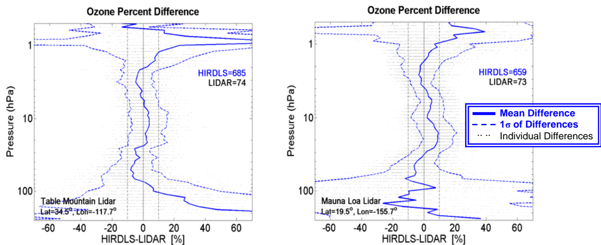
Figure 5.2.2. Shown are the ozone percent differences between 74 TMF lidar profiles and 685 coincident HIRDLS profiles (left), and 73 MLO lidar profiles and 659 coincident HIRDLS profiles (right).
