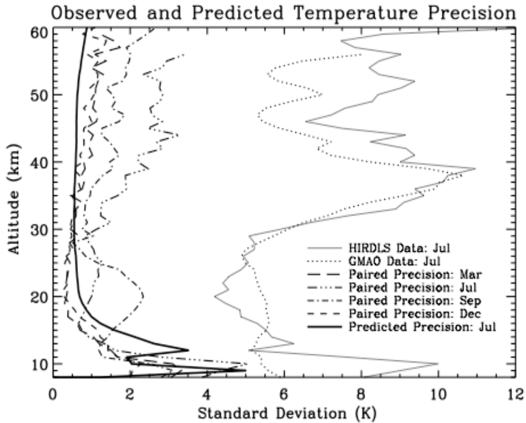
Figure 5.1.4. Empirically determined precision for HIRDLS determined from differences of paired profiles (dashed line) at latitude cross-over points at 63°S for 3 days each in in March, July, September and December, compared to total precision calculated by the retrieval code (solid line). The standard deviations of the GMAO and HIRDLS data for July are also shown. The similarity between the shapes of the summer curve and the predicted values gives us confidence that the predicted values are a reasonable indication the true repeatability of HIRDLS temperatures.
