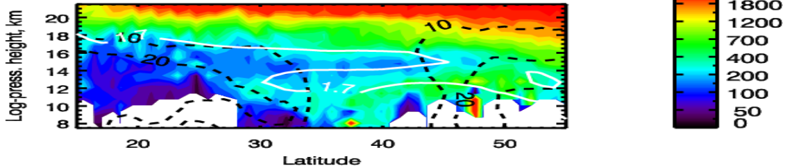
23-01-2006, HIRDLS HNO3, ppbv, Orbit: 141-143 W
