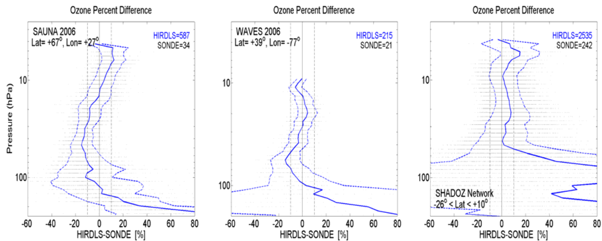
Figure 5.2.1. Shown are the ozone percent differences between ozonesondes and HIRDLS coincident profiles for a high latitude campaign, SAUNA (left), a mid-latitude campaign, WAVES (center) and the low latitude SHADOZ network (right). Mean differences (solid blue), standard deviation (dashed blue) and individual differences (black dots) are indicated. The number of coincident profiles included in the statistical difference is indicated in the upper right corner of each panel.
