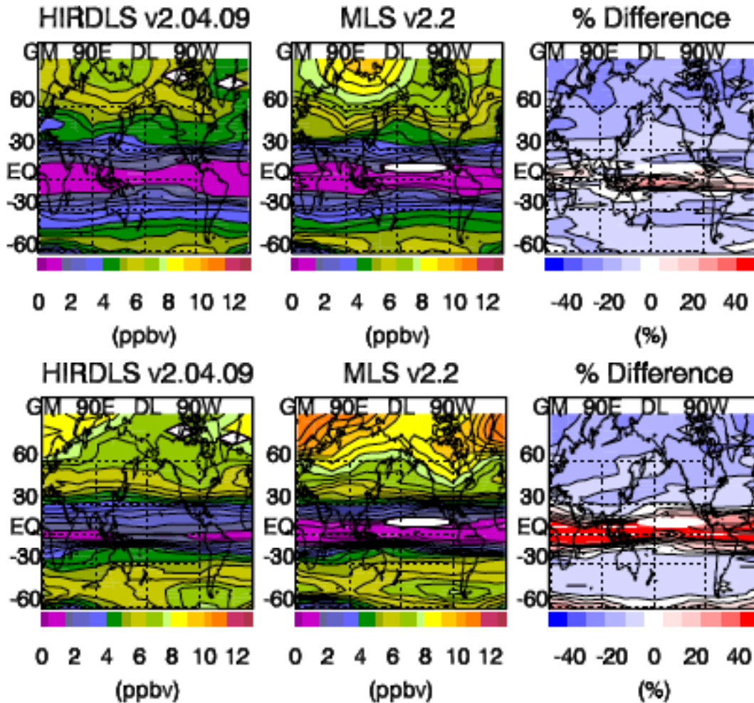
Figure 5.3.5. Longitude-latitude cross sections of HIRDLS and MLS HNO 3 (ppbv) on 28 October 2006. The top and bottom rows are for 51.1 hPa and 31.6 hPa respectively. The percentage difference of (\text{HIRDLS} - \text{MLS}) / \text{MLS} is also shown. The zero percentage difference contour line is the transition from white to blue.
