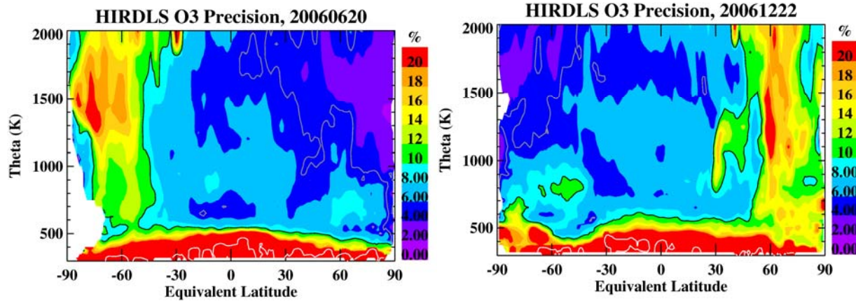
Figure 5.2.6. Shown is the standard deviation of ozone in different equivalent latitude and potential temperature bins, an estimate of HIRDLS ozone precision. Results are given for two days, 2006 June 20 (left) and 2006 December 22 (right), in terms of percentage of ozone mixing ratio.
