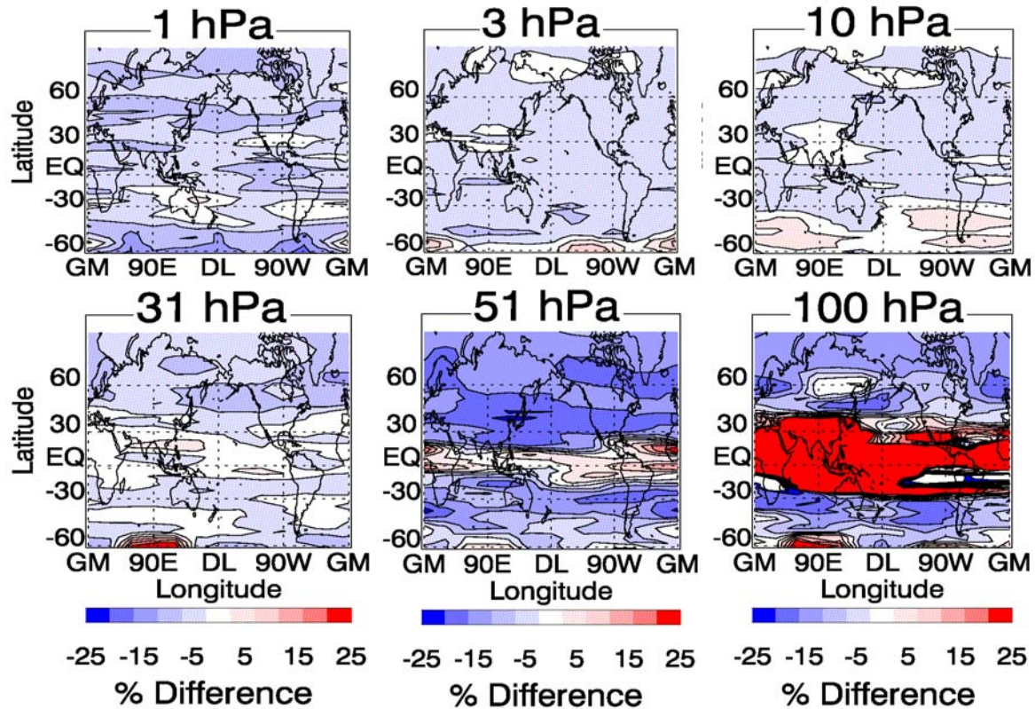
Figure 5.2.5. Mercator representations of the ozone percent difference between HIRDLS and collocated MLS (v2.2) for 2006-July-15, at pressure levels, 1, 3, 10, 31, 51 and 100 hPa, as indicated over each sub-plot. The ozone fields for this day are relatively quiescent.
