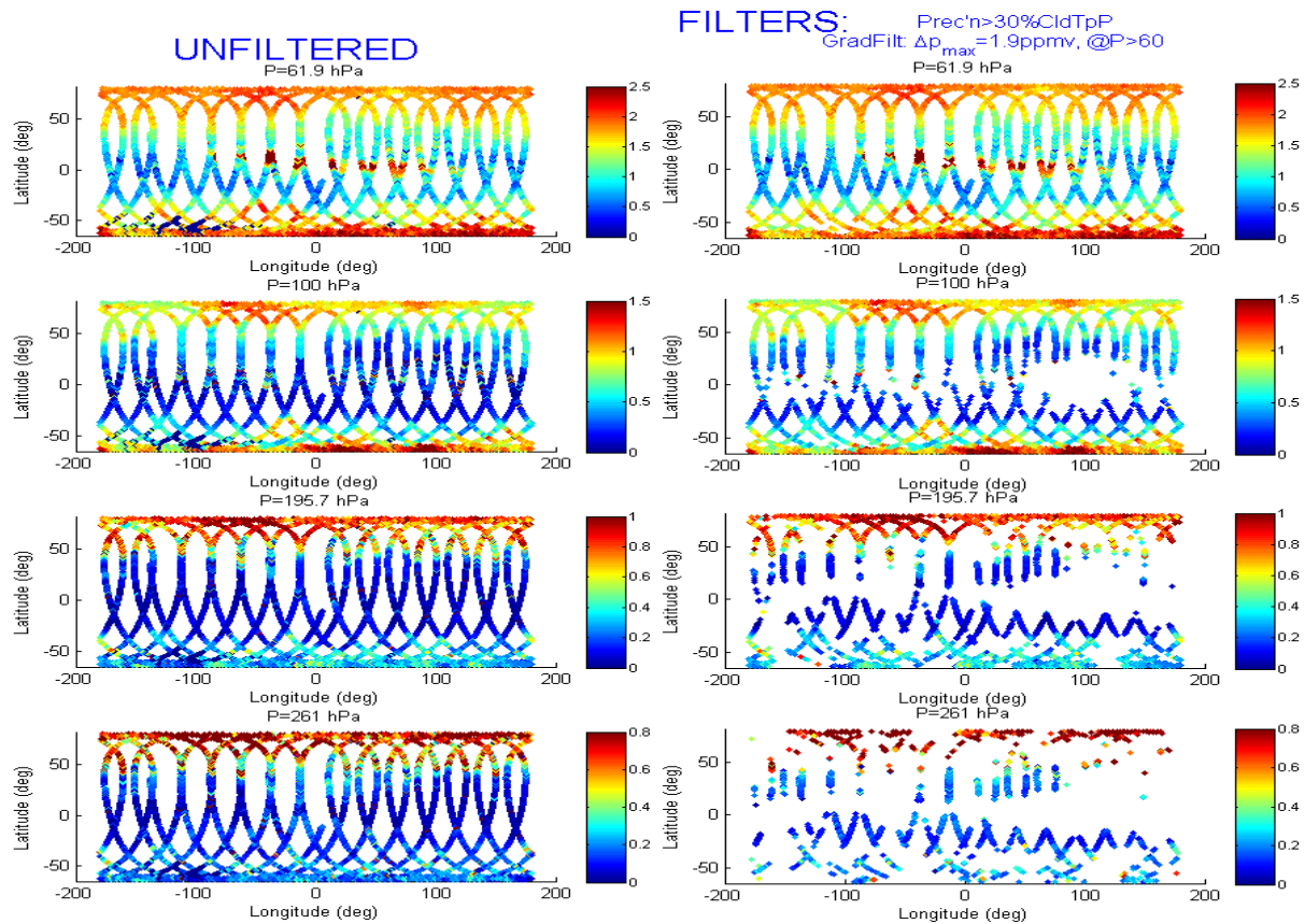
Figure 5.2.8. Shown are HIRDLS v003 ozone on four pressure surfaces (62, 100, 196, 261 hPa) for a 24 hour period on 2006-June-19. At left are the raw unfiltered data and on the right are the filtered data using the three recommended filters.
