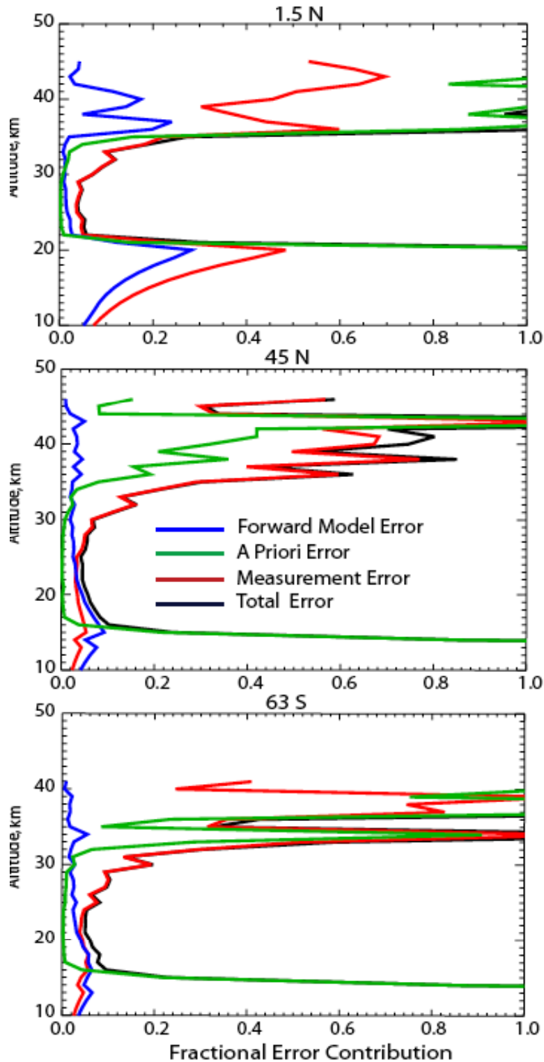
Figure 5.3.2: Shown is the HIRDLs \text{HNO}_3 “theoretical precision” displayed as the fractional error contribution for 21 June 2006. The top, middle, and lower panels are for latitudes 1.5^\circ\text{N} , 45.3^\circ\text{N} and 63^\circ\text{S} respectively (same regions as Figure 5.3.1). The forward model error (blue
