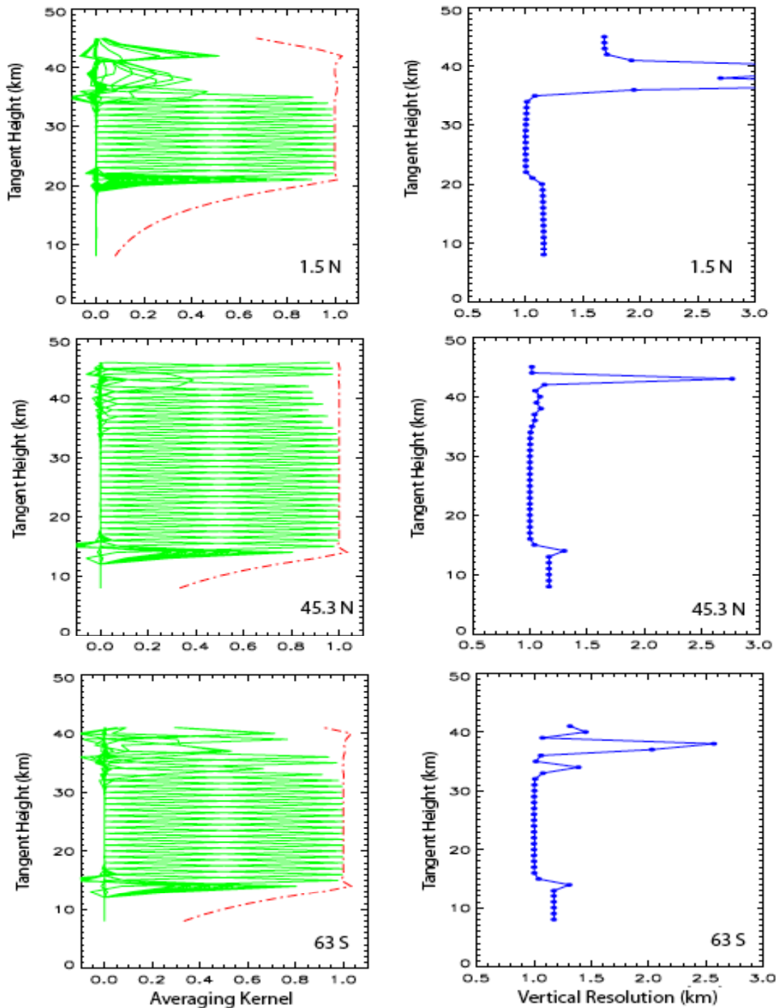
Figure 5.3.1: HIRDLS \text{HNO}_3 averaging kernels and full width half maximum (FWHM) vertical resolution profiles are shown on 21 June 2006 at 1.5^\circ\text{N} , 45.3^\circ\text{N} , and 63^\circ\text{S} . The left column shows the averaging kernels (green lines) and the integrated area under each kernel (red line). Where values of unity indicate that all of the information for that vertical region is coming from the measurements and not the a priori estimate. The right column represents the vertical resolution as derived from the FWHM of each kernel (blue line).
