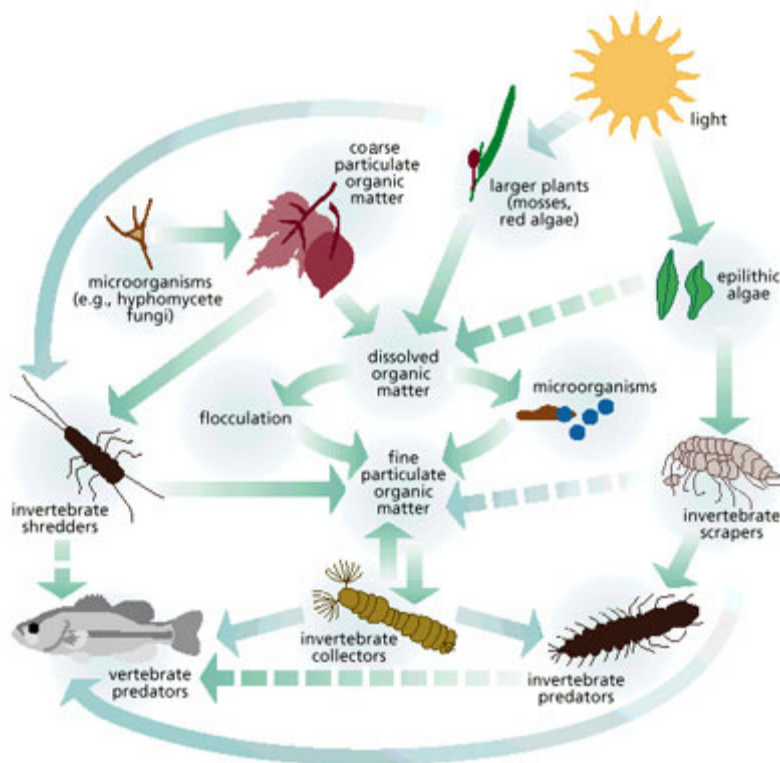
Figure 13. A simplified watershed food web
