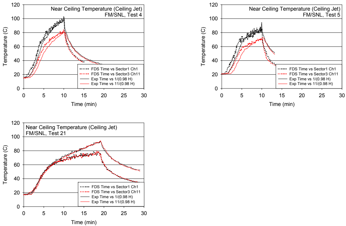
Figure A-20. Near-ceiling gas temperatures, FM/SNL Series, Sectors 1 and 3.
