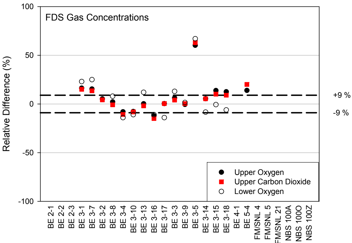
Figure 6-5. Summary of FDS predictions of major gas concentrations.
