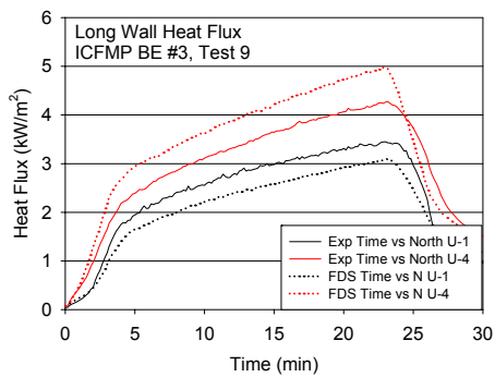
Figure A-67. Long wall heat flux and surface temperature, ICFMP BE #3, closed door tests.
