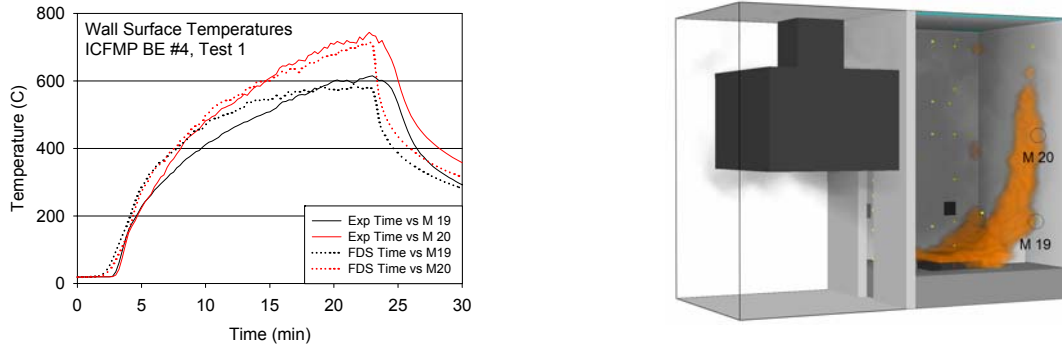
Figure A-81. Back wall surface temperatures, ICFMP BE #4, Test 1. Note that the smoke has been artificially lightened in the picture on the right.
