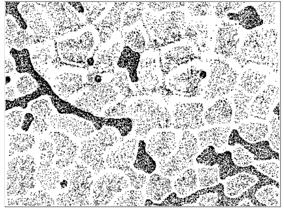
Figure 8. Dark NAPL (Soltrol) and water in a homogenous micromodel after (a) the displacement of water by NAPL and then (b) the displacement of NAPL by water, with NAPL at residual saturation (Wilson et al., 1990).
