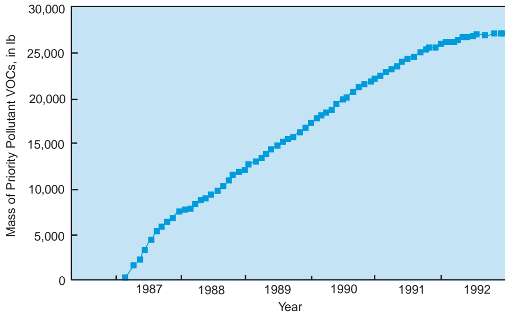
Figure 31. Cumulative mass of VOCs removed from the aquifer at the Chem-Dyne site from 1987 to 1992 (Cohen et al., 1994, after Papadopulos & Associates, 1993).
