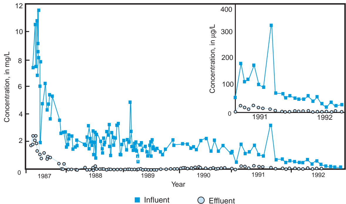
Figure 30. Influent and effluent VOC concentrations (mg/L) at the Chem-Dyne treatment plant from 1987 to 1992 (Cohen et al., 1994, after Papadopoulos & Associates, 1993).
