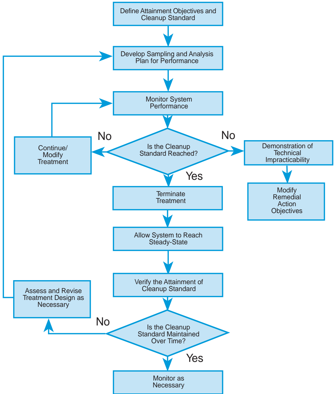
Figure 32. Determining the success and/or timeliness of closure of a pump-and-treat system (Cohen et al., 1994).
