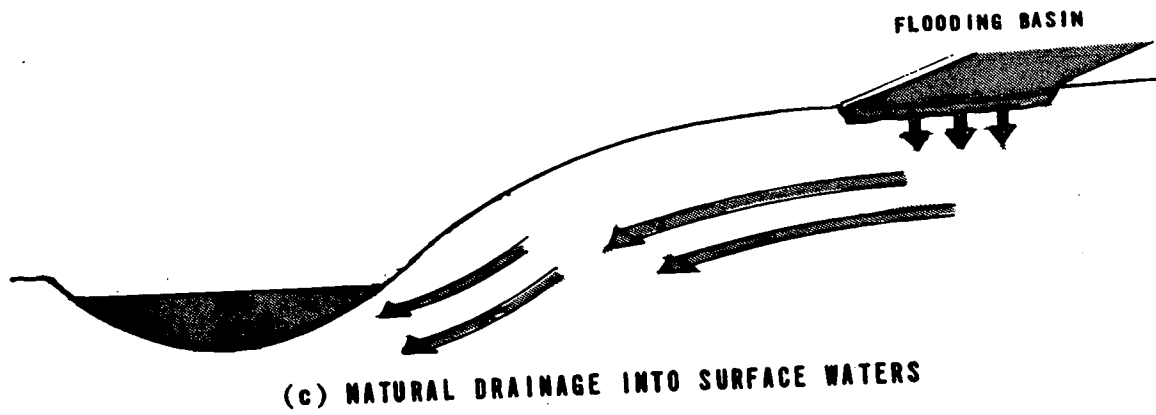
FIGURE 1-2 RAPID INFILTRATION HYDRAULIC PATHWAYS
