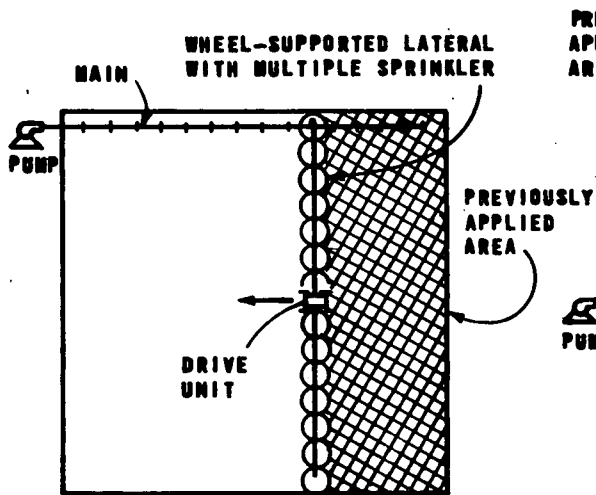
(c) SIDE WHEEL ROLL
