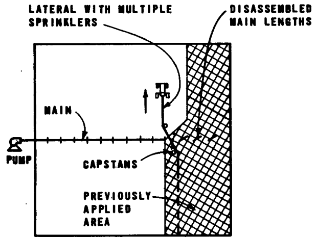
(b) END TOW
