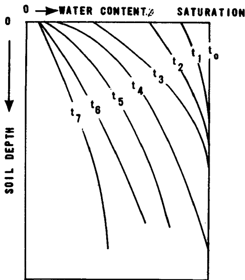
FIGURE 3-5 TYPICAL PATTERN OF THE CHANGING MOISTURE PROFILE DURING DRYING AND DRAINAGE
