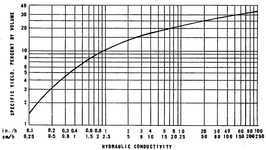
FIGURE 3-4 GENERAL RELATIONSHIP BETWEEN SPECIFIC YIELD AND HYDRAULIC CONDUCTIVITY [9]
