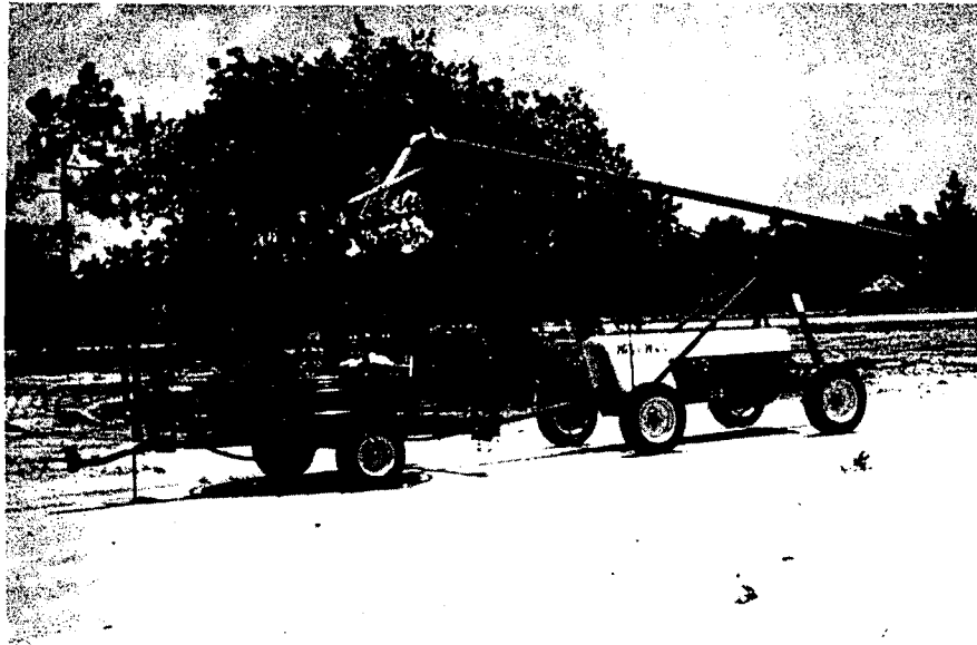
FIGURE E-8 HOSE-DRAG TRAVELING GUN SPRINKLER
