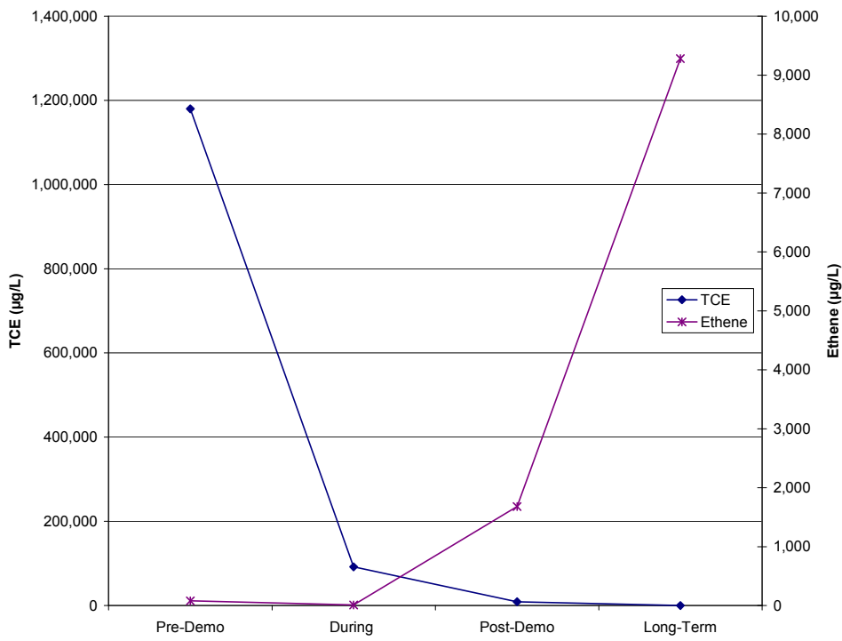
Figure C-2. TCE and Ethene Concentrations in Groundwater in PA-23 after EZVI Treatment
