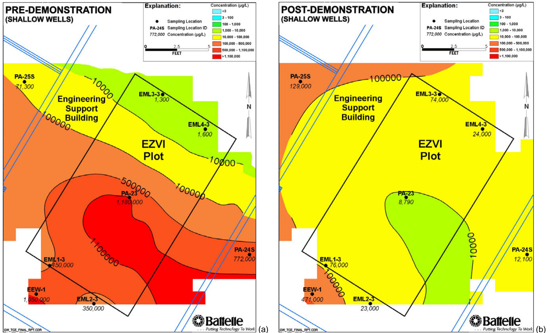
Figure 5-5. Dissolved TCE Concentrations (µg/L) during (a) Pre-Demonstration (March 2002) and (b) Post-Demonstration (November 2002) Sampling of Shallow Wells
