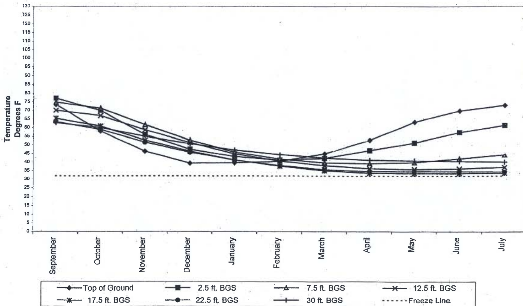
Figure 2-20 Subsurface Temperature Data Over Time for T-5
