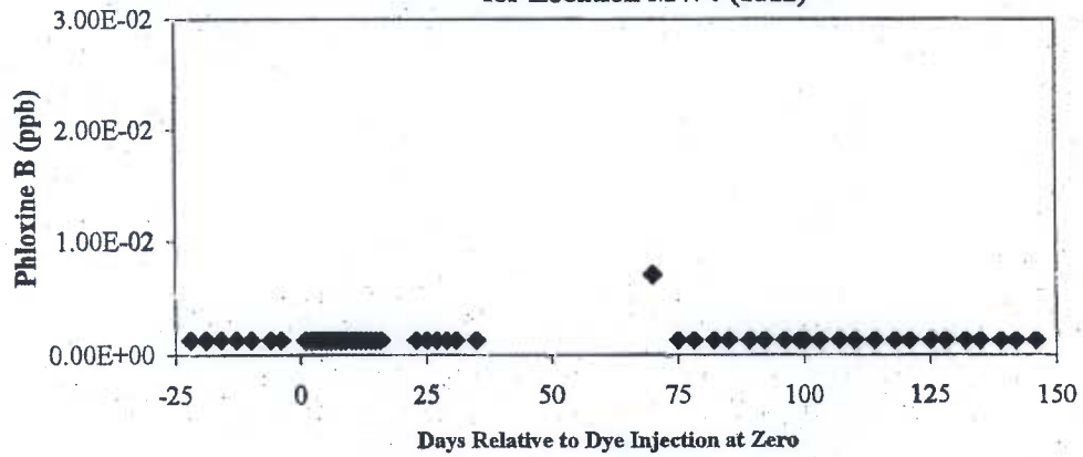
Figure 2-7 Concentrations of Phloxine B Versus Time for Location MW4 (1112)
