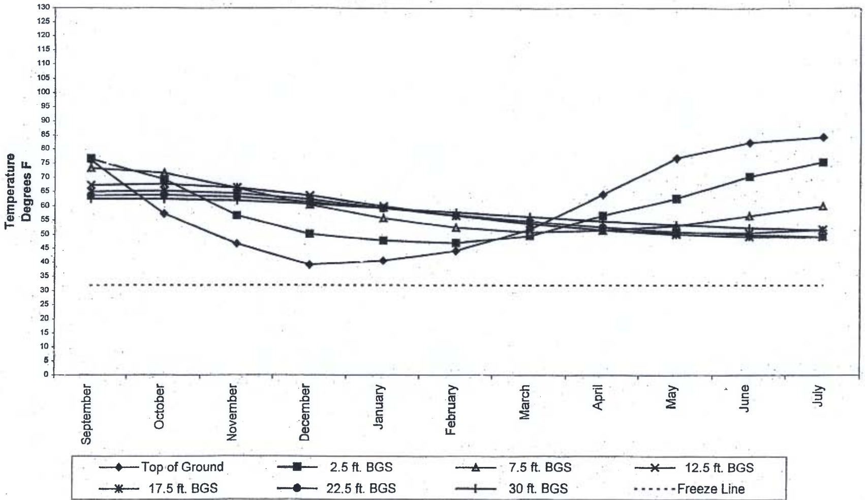
Figure 2-22 Subsurface Temperature Data Over Time for T-7
