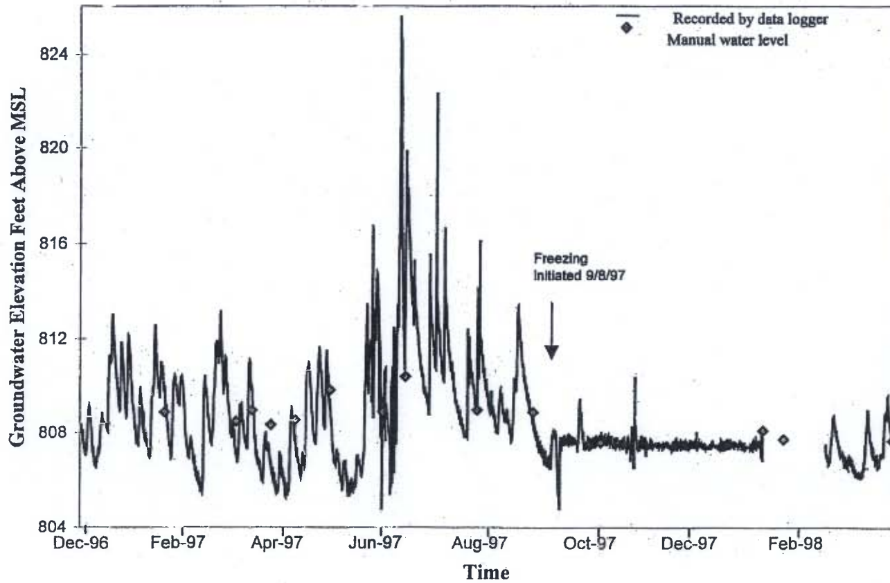
Figure 2-16 Hydrograph for Monitoring Well MW2 (1110)
