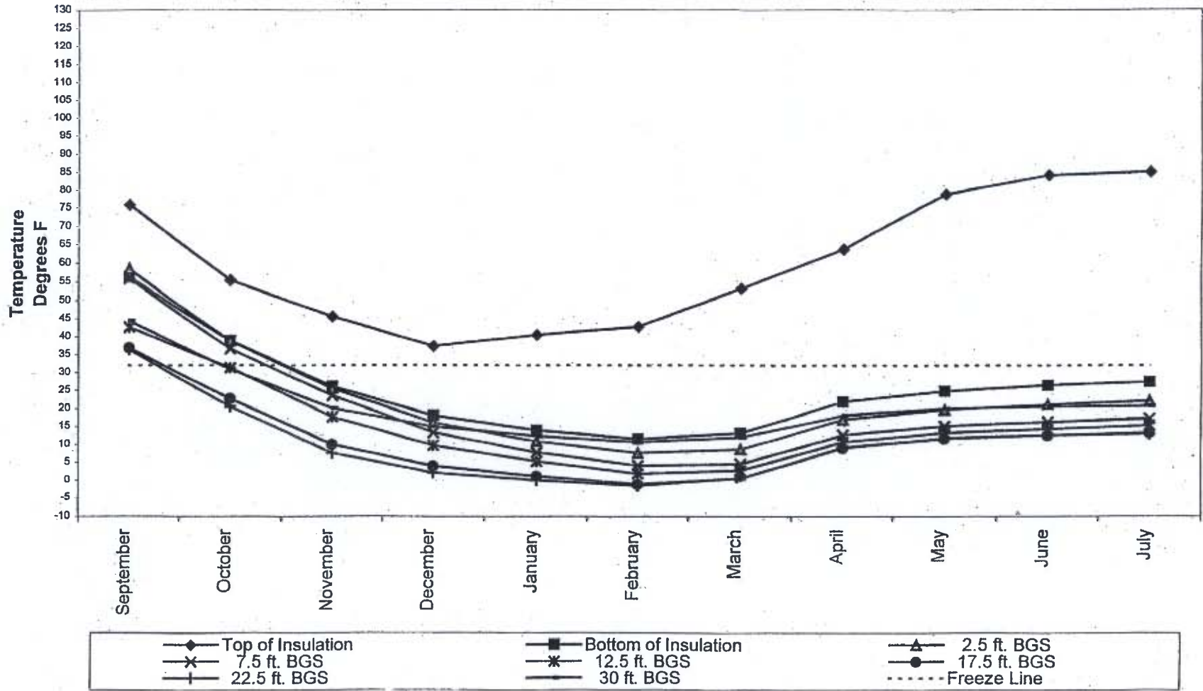
Figure 2-18 Subsurface Temperature Data Over Time for T-3
