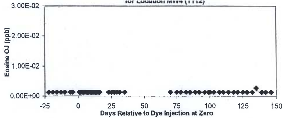
Figure 2-12 Concentrations of Eosine OJ Versus Time for Location MW4 (1112)
