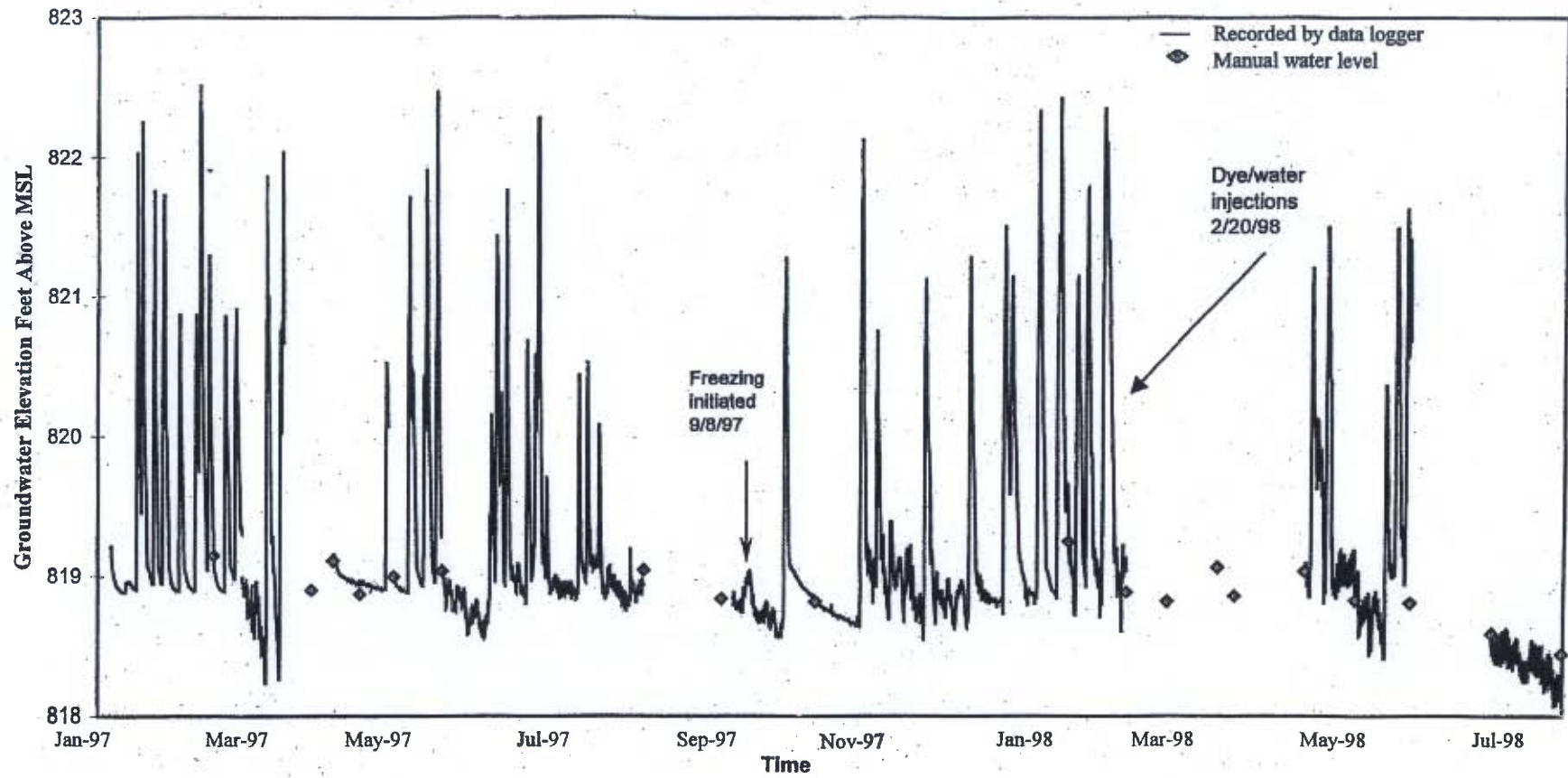
Figure 2-15 Hydrograph for Standpipe STP10
