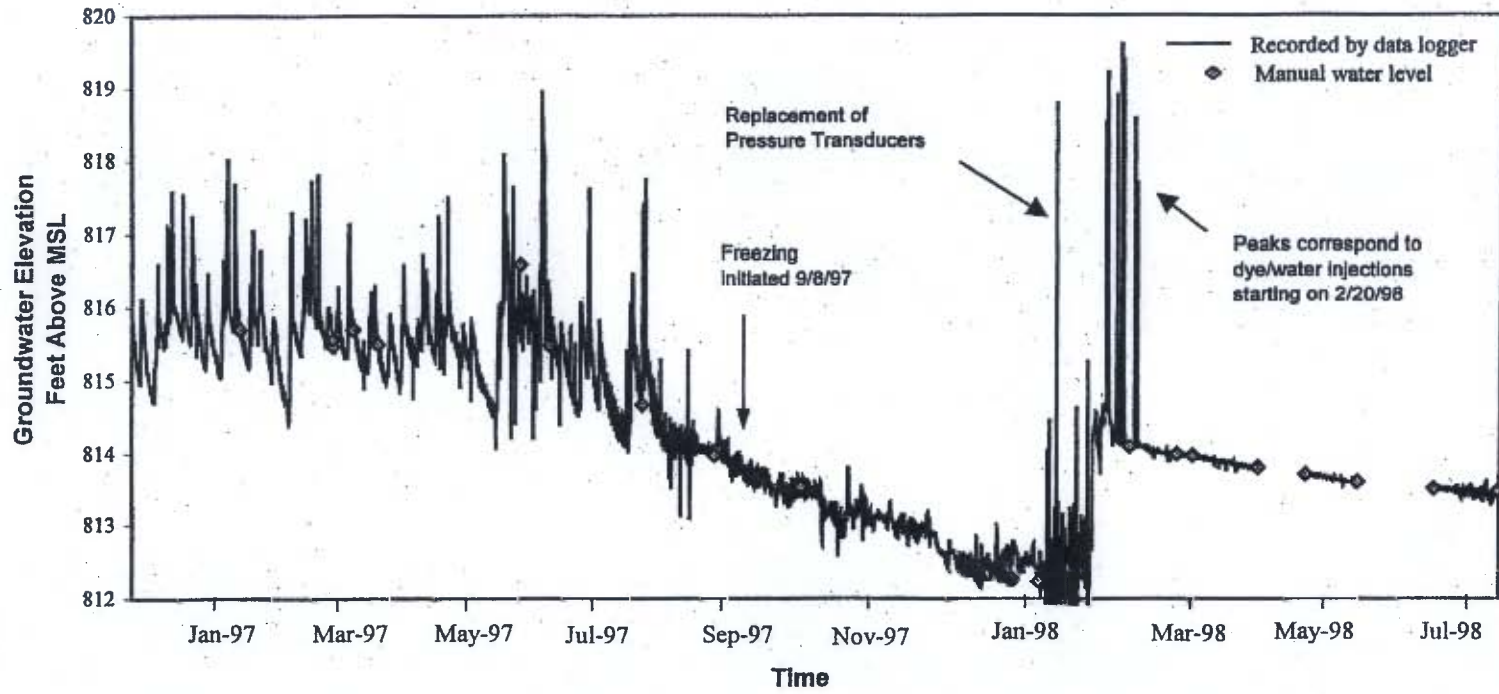
Figure 2-14 Hydrograph for Standpipe I2
