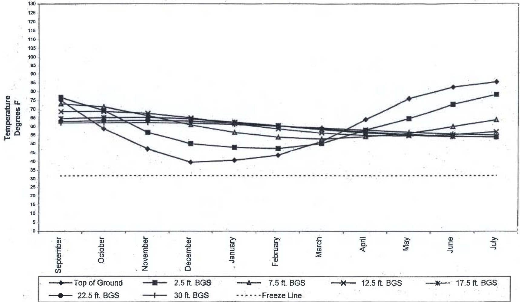
Figure 2-23 Subsurface Temperature Data Over Time for T-8
