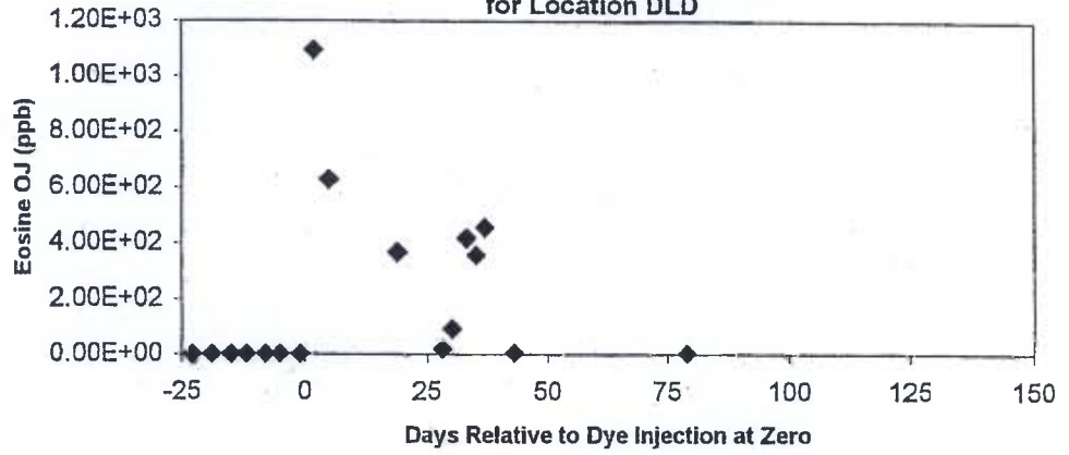
Figure 2-11 Concentrations of Eosine OJ Versus Time for Location DLD
