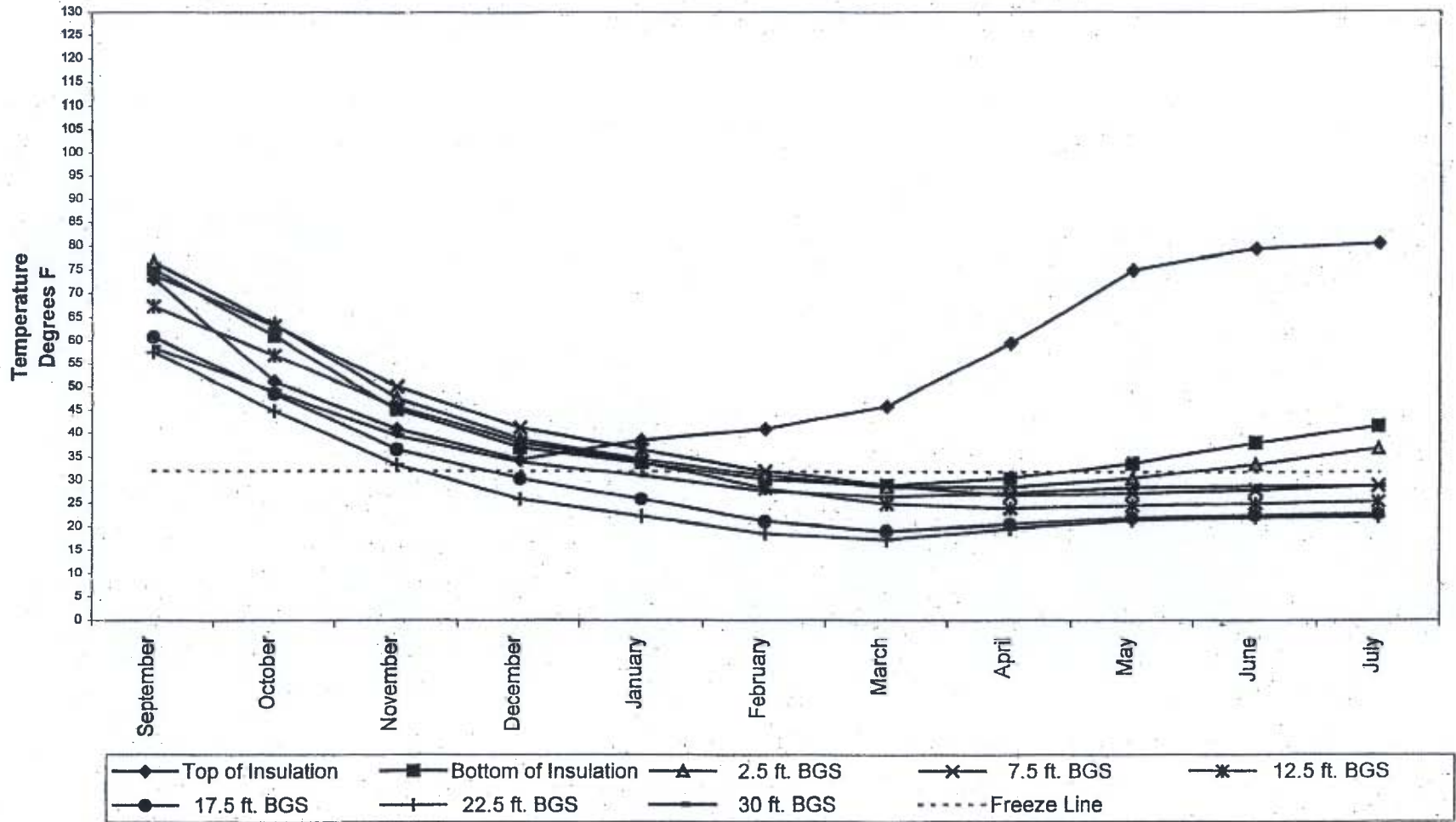
Figure 2-19 Subsurface Temperature Data Over Time for T-4
