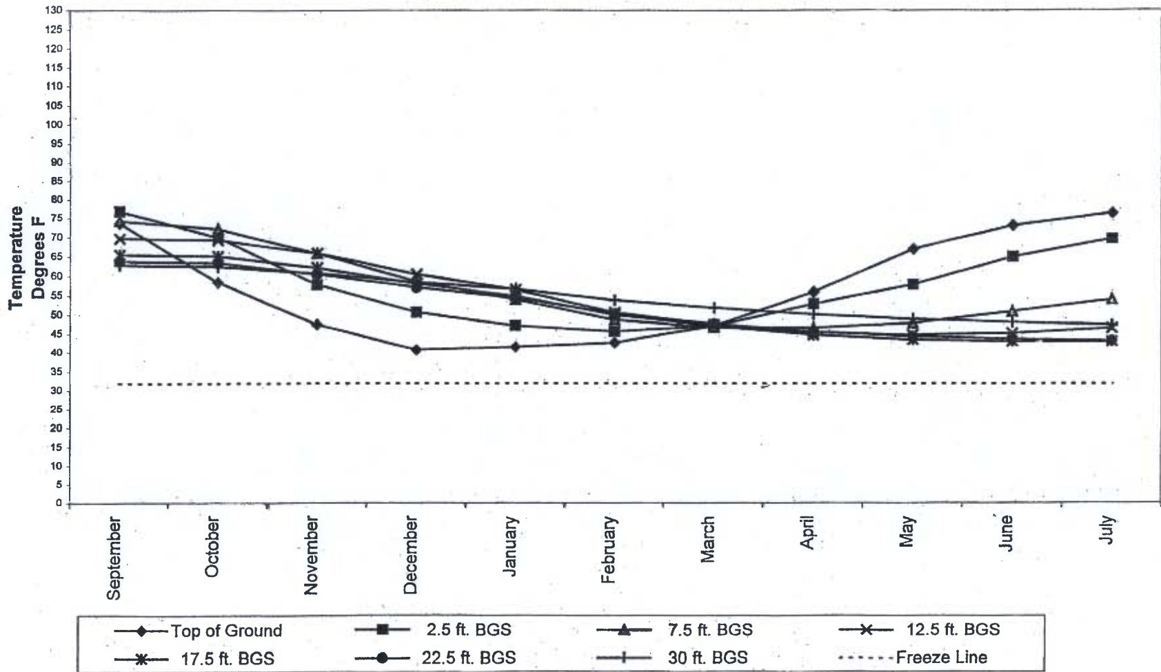
Figure 2-21 Subsurface Temperature Data Over Time for T-6
