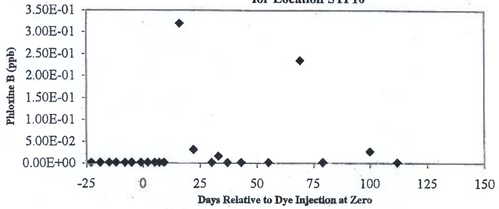
Figure 2-2 Concentrations of Phloxine B Versus Time for Location STP10
