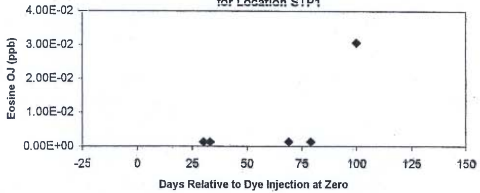
Figure 2-9 Concentrations of Eosine OJ Versus Time for Location STP1
