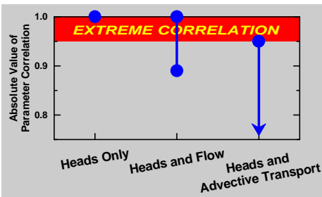
Figure 3. Range of parameter correlation for the Otis Air Force Base model with different types of data. For correlation greater than 0.95, parameters may not be estimated uniquely and predictions may be substantially in error. For the data set with heads only, all values equal 1.
