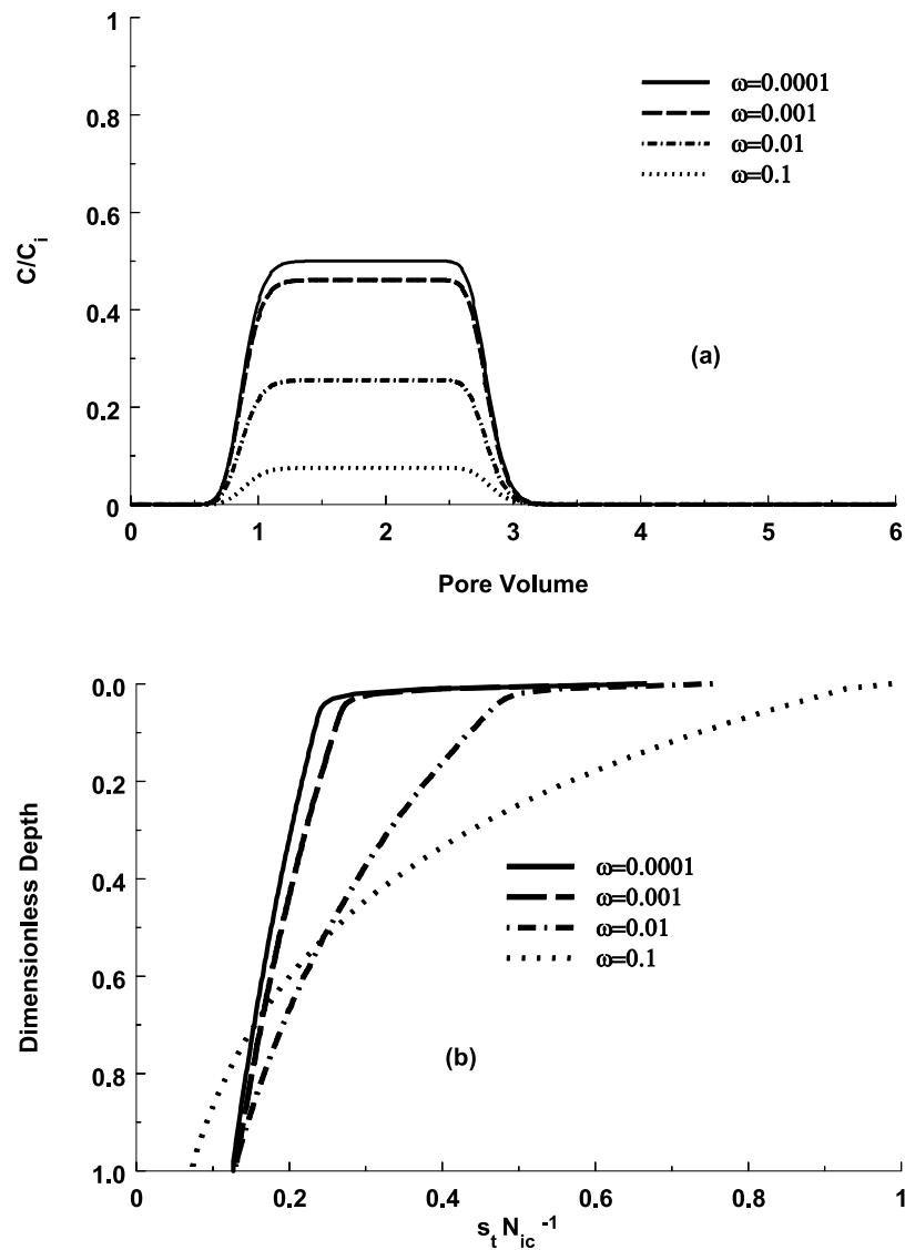
Figure 2. Plots of (a) simulated breakthrough curves and (b) retention profiles when wq_2 was 0.001 \text{ cm min}^{-1} , q_t was 0.0918 \text{ cm min}^{-1} , and \omega was 0.0001 , 0.001 , 0.01 , and 0.1 \text{ min}^{-1} . Other model parameters are provided in the manuscript text.
