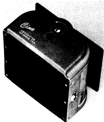
FIGURE 5.—A variation of the device shown in figure 4 was developed for the Gemini program, with a plate attached for storing the magazines. After experimenting with a silver finish, the decision was made to continue with a black finish until the lunar landing.
