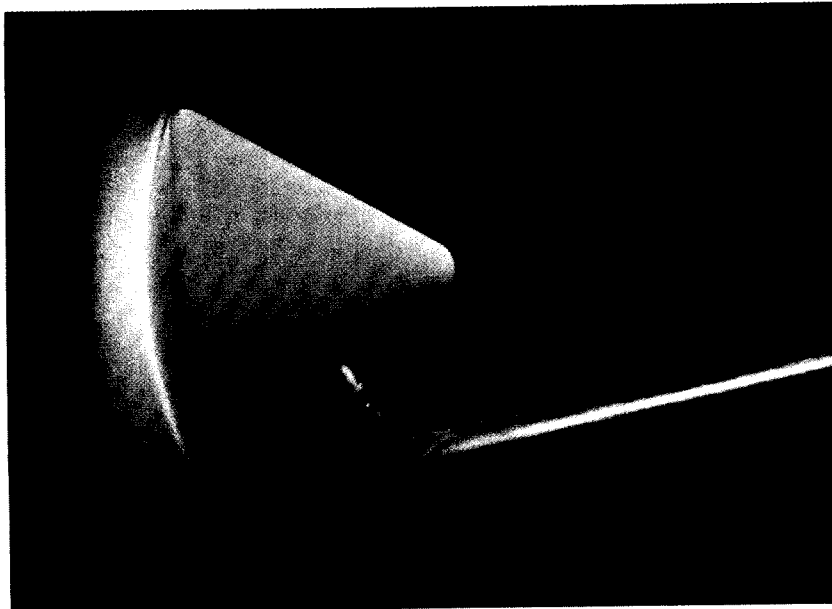
This striking picture of an Apollo model capsule is one of a series used to evaluate heat transfer to the afterbody of the model. It was taken during one of the ablation tests which simulate reentry phenomena in a wind tunnel.
