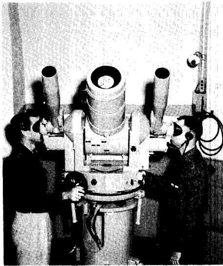
FIGURE 21. —This photograph was taken at the Air Force Eastern Test Range which has responsibility for tracking the vehicles after they leave the launch complexes at Cape Kennedy Air Force Station and Kennedy Space Center. It shows a cinetheodolite which, in addition to tracking the vehicle, records on film complete geometrical information with respect to azimuth elevation and the time each frame was taken.
