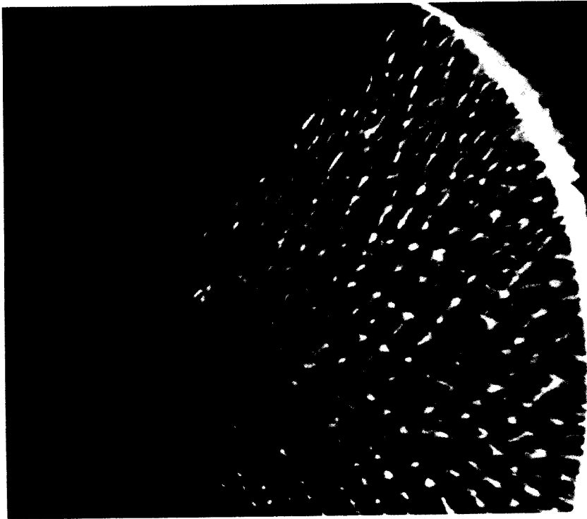
A closeup of patterns formed during ablation on a Lexan plastic model of a cone form. A sequence of pictures of this occurrence shows how the pattern forms as velocity increases and ablation develops.
