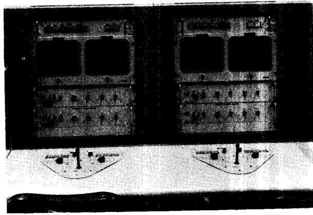
FIGURE 48.—This view of the photographic control center associated with the remote tracking cameras shows the monitors which are used with closed-circuit television boresight instruments for viewing events seen by the camera through remote TV. Through controls in front of and on the desk of the console, the operator can direct the tracking camera to follow any event during the launch cycle.
