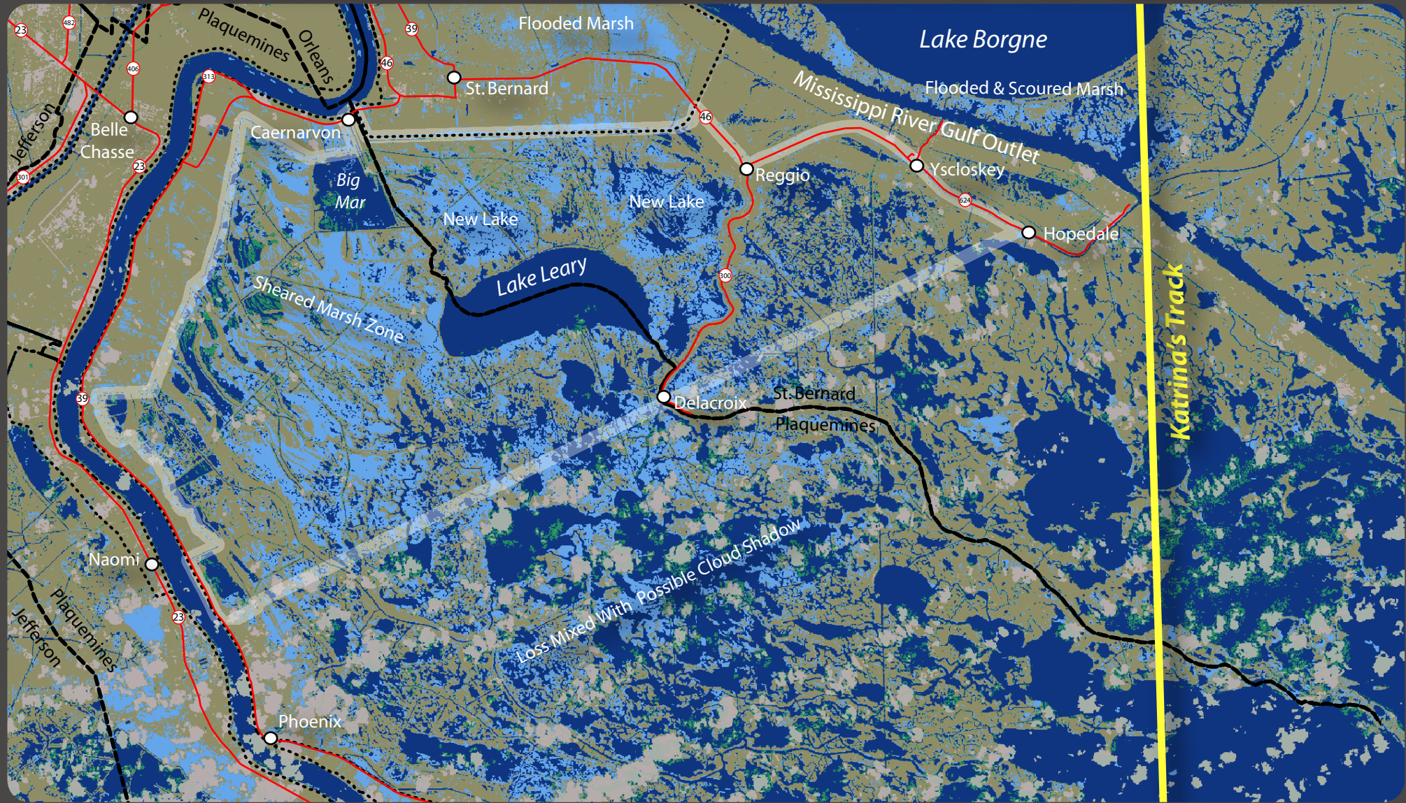
Change Map November 7, 2004 to September 7, 2005 Based on Classified Landsat Thematic Mapper 5 Satellite Land - Water Images
