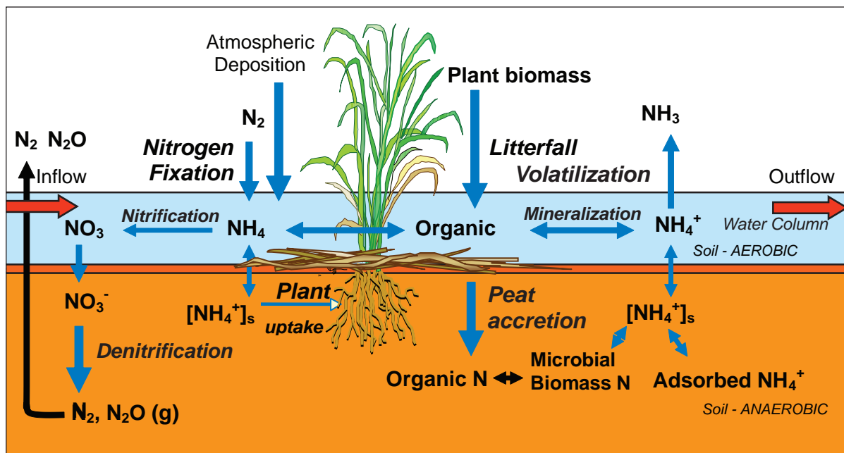
Figure 2.5: Schematic of the nitrogen cycle in wetlands.
