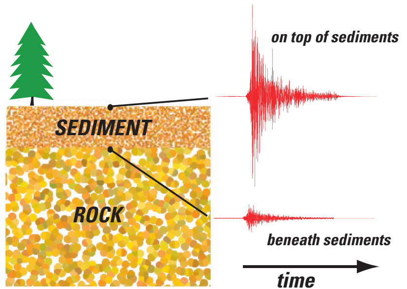
Figure 4. When waves of a small earthquake impinge on the boundary between hard rock and overlying sediments from below (lower seismogram), they become amplified as they travel through the sediments to the surface (upper seismogram). A seismogram records the wave motion over time. The amplifying effects of thick sediments above the New Madrid seismic zone results in motions at the surface that are many times larger than below. (Courtesy of C. Langston, The University of Memphis.)
