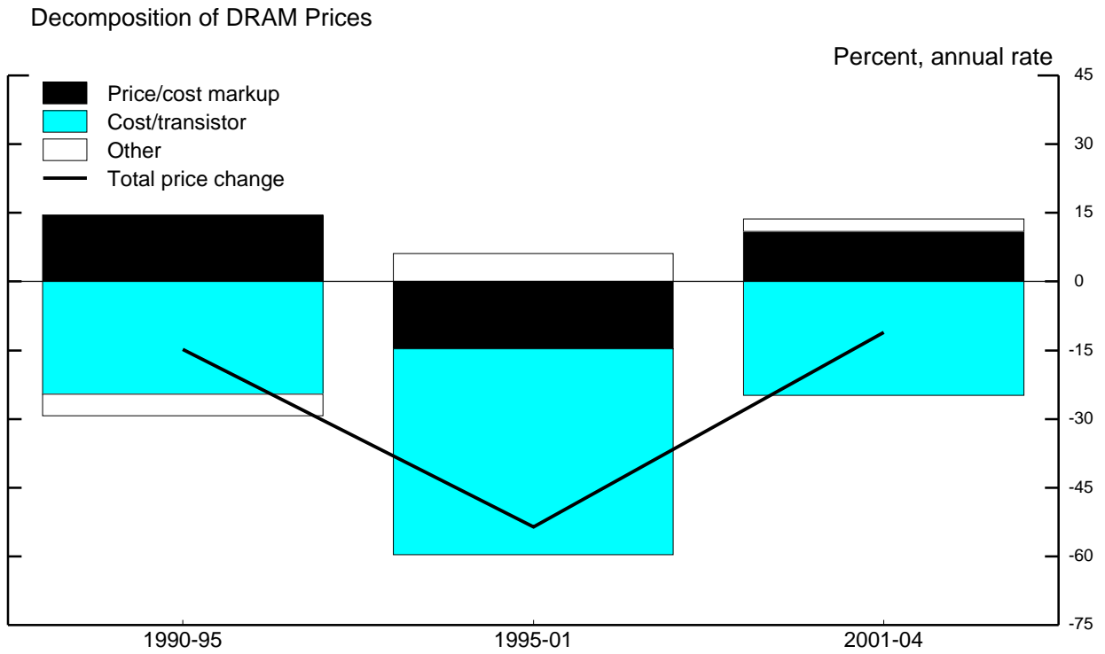
Figure 4 Decomposition of Constant-Quality Semiconductor Price Changes
