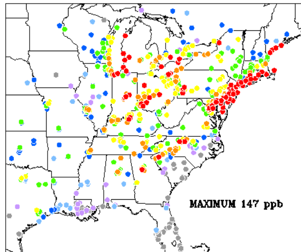
MAXIMUM OBSERVED 8-HR OZONE CONCENTRATIONS (ppb) OVER THE EASTERN UNITED STATES AND ONTARIO July 14, 1995
