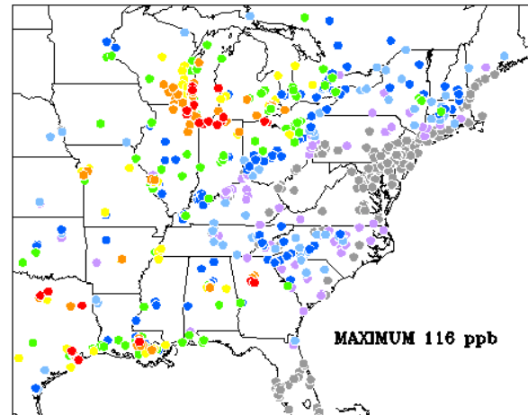
MAXIMUM OBSERVED 8-HR OZONE CONCENTRATIONS (ppb) OVER THE EASTERN UNITED STATES AND ONTARIO June 23, 1995
