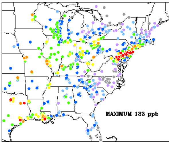
MAXIMUM OBSERVED 8-HR OZONE CONCENTRATIONS (ppb) OVER THE EASTERN UNITED STATES AND ONTARIO June 20, 1995
