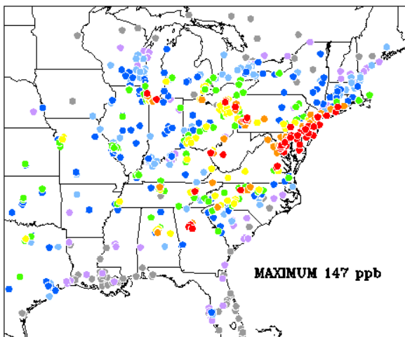
MAXIMUM OBSERVED 8-HR OZONE CONCENTRATIONS (ppb) OVER THE EASTERN UNITED STATES AND ONTARIO July 15, 1995
