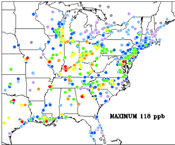
MAXIMUM OBSERVED 8-HR OZONE CONCENTRATIONS (ppb) OVER THE EASTERN UNITED STATES AND ONTARIO July 11, 1995
