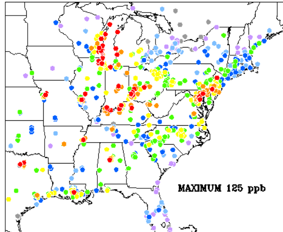
MAXIMUM OBSERVED 8-HR OZONE CONCENTRATIONS (ppb) OVER THE EASTERN UNITED STATES AND ONTARIO July 12, 1995
