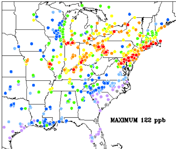
MAXIMUM OBSERVED 8-HR OZONE CONCENTRATIONS (ppb) OVER THE EASTERN UNITED STATES AND ONTARIO June 18, 1995
