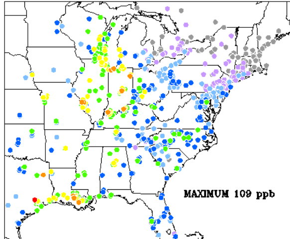
MAXIMUM OBSERVED 8-HR OZONE CONCENTRATIONS (ppb) OVER THE EASTERN UNITED STATES AND ONTARIO June 15, 1995
