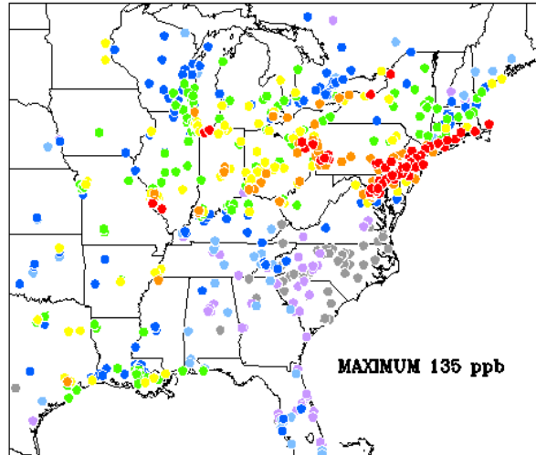
MAXIMUM OBSERVED 8-HR OZONE CONCENTRATIONS (ppb) OVER THE EASTERN UNITED STATES AND ONTARIO June 19, 1995
