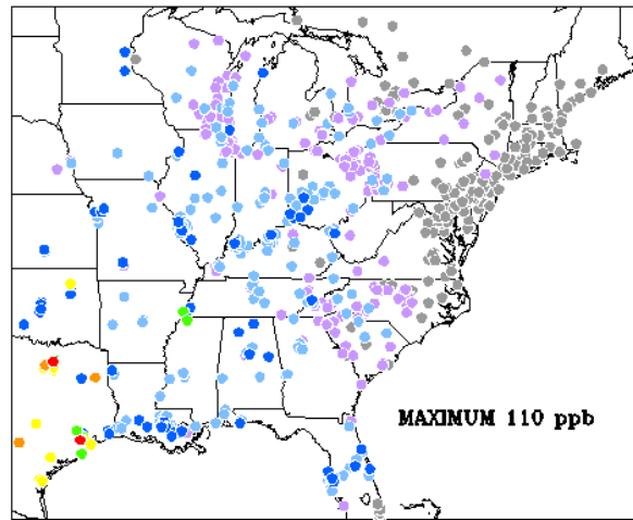
MAXIMUM OBSERVED 8-HR OZONE CONCENTRATIONS (ppb) OVER THE EASTERN UNITED STATES AND ONTARIO June 13, 1995
