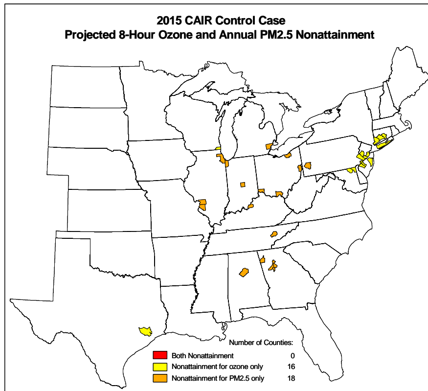
Figure VIII-3. PM2.5 and 8-hour ozone nonattainment counties in the East for the 2015 Base Case (top) and 2015 CAIR control case (bottom).
