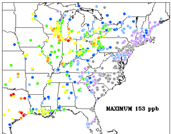
MAXIMUM OBSERVED 8-HR OZONE CONCENTRATIONS (ppb) OVER THE EASTERN UNITED STATES AND ONTARIO June 22, 1995
