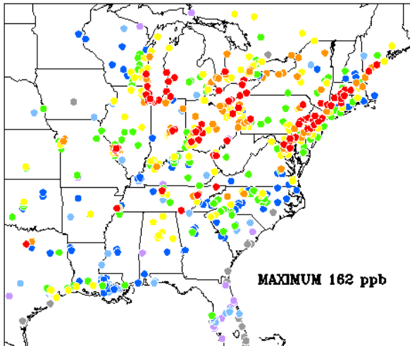
MAXIMUM OBSERVED 8-HR OZONE CONCENTRATIONS (ppb) OVER THE EASTERN UNITED STATES AND ONTARIO July 13, 1995
