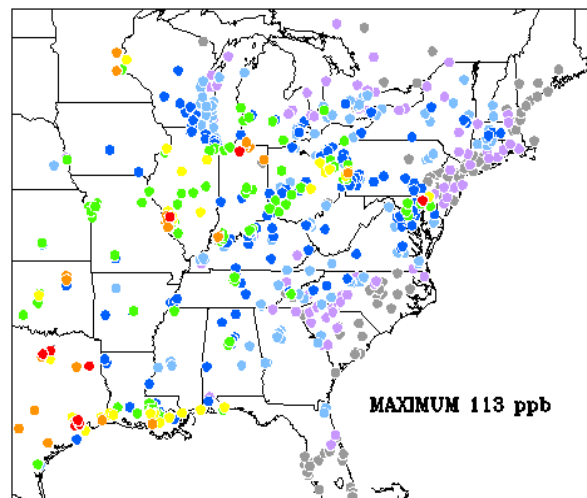
MAXIMUM OBSERVED 8-HR OZONE CONCENTRATIONS (ppb) OVER THE EASTERN UNITED STATES AND ONTARIO June 21, 1995
