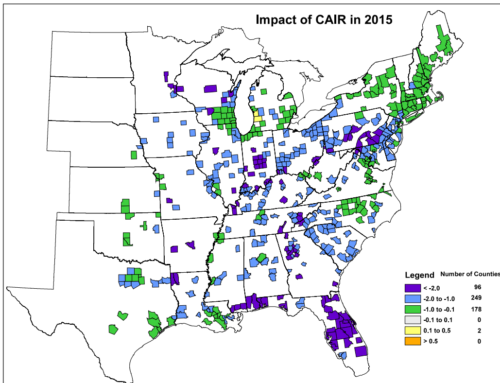
Figure VIII-7. Regionwide reduction in 8-hour ozone concentrations expected from CAIR in 2010 (top) and 2015 (bottom).
