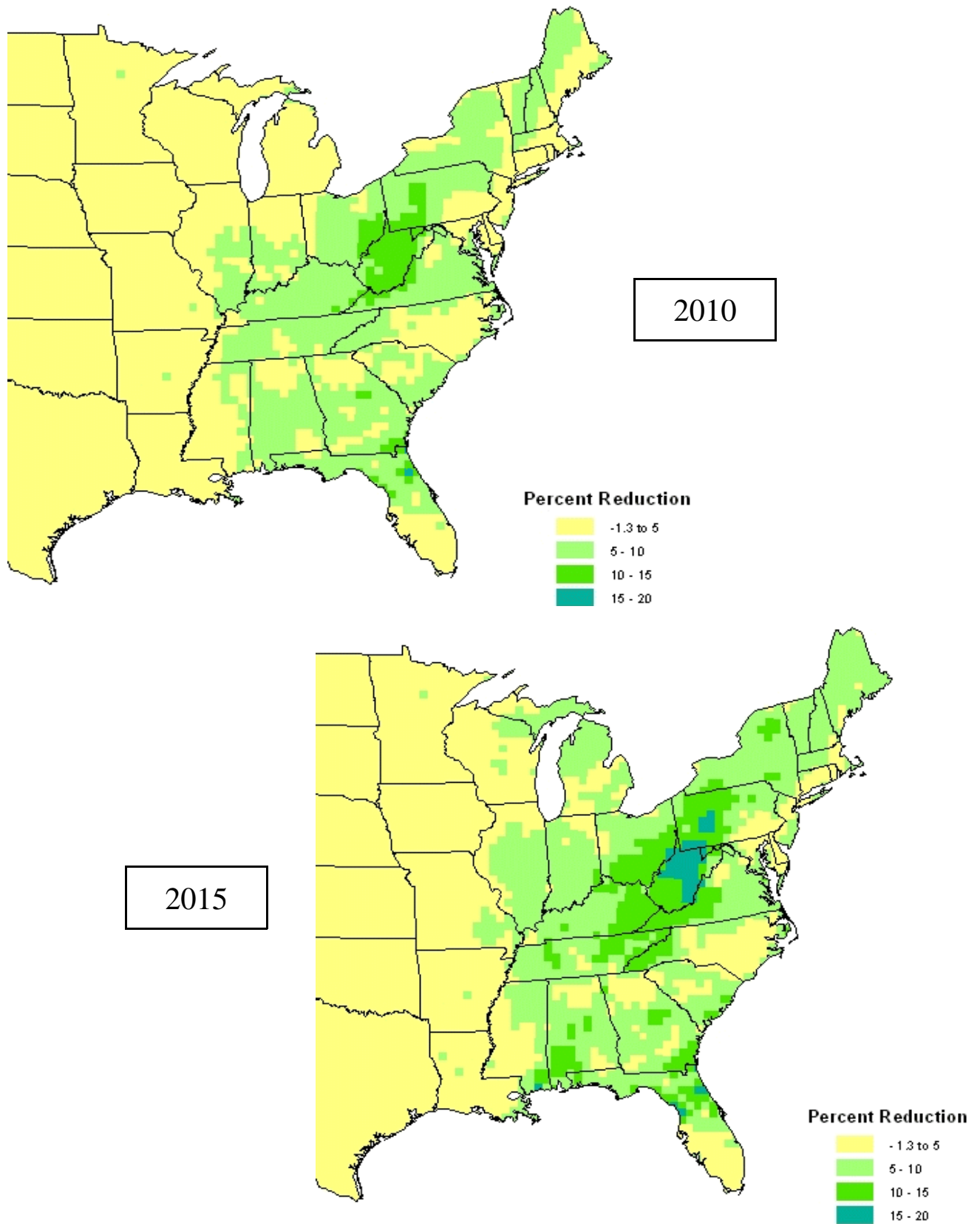
Figure VIII-8. Percent reduction in total nitrogen deposition expected from CAIR in 2010 (top) and 2015 (bottom).
