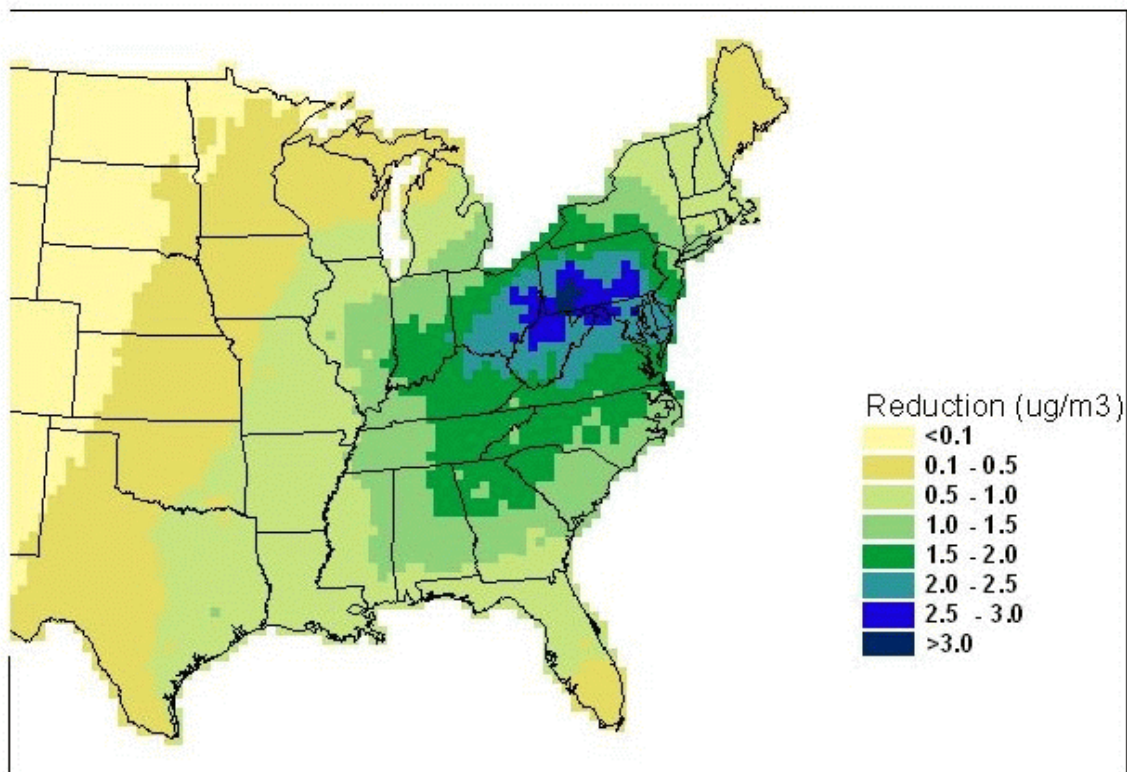
Figure VIII-5. Regionwide reduction in annual average PM 2.5 expected from CAIR in 2010 (top) and 2015 (bottom).
