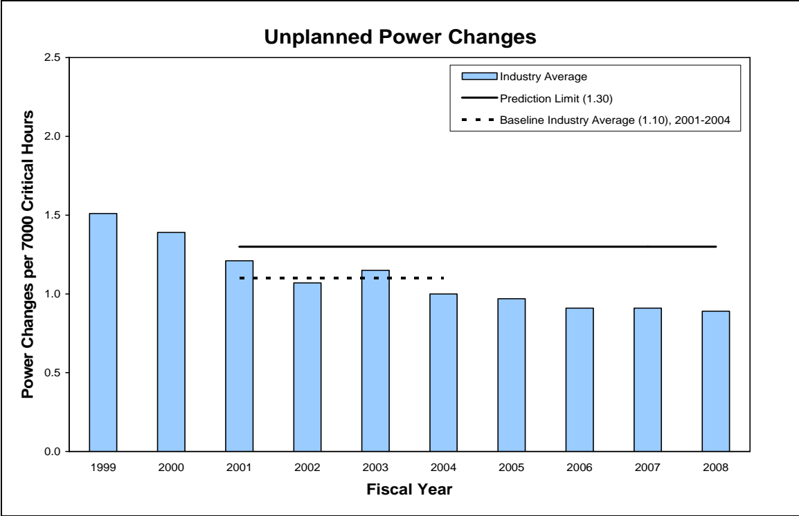
Figure 8. Unplanned Power Changes per 7000 Critical Hours
