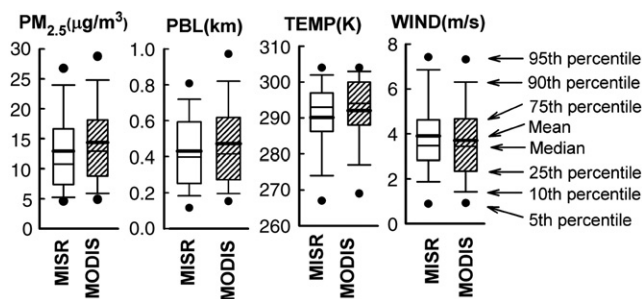
Fig. 3. Boxplots showing the distribution (5th, 10th, 25th, median, 75th, 90th, and 95th percentiles) of PM 2.5 concentrations, mixing height (PBL), surface wind speed (WIND), and surface air temperature (TEMP). The means values are shown as the thick solid line in the plots.
