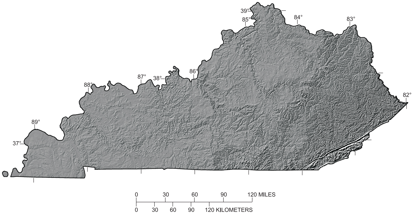
Figure 2. Shaded-relief image of landforms in Kentucky.
