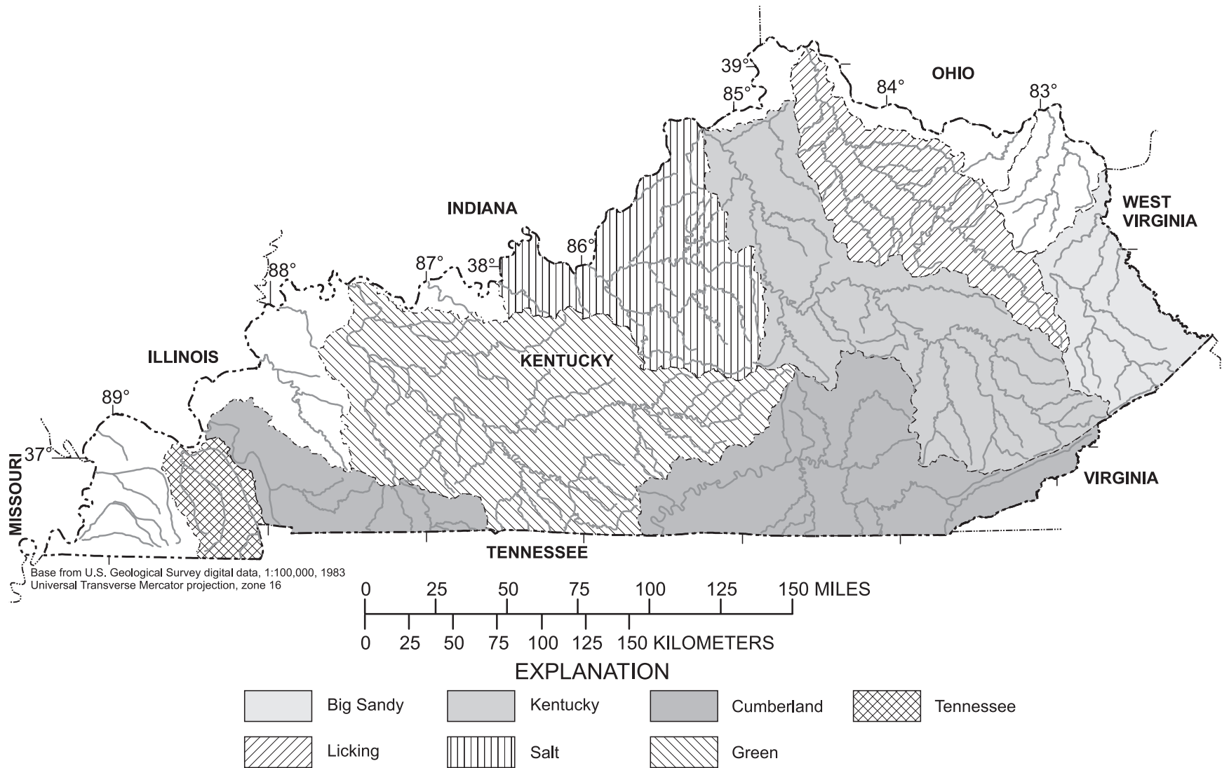
Figure 1. Major drainage basins in Kentucky.
