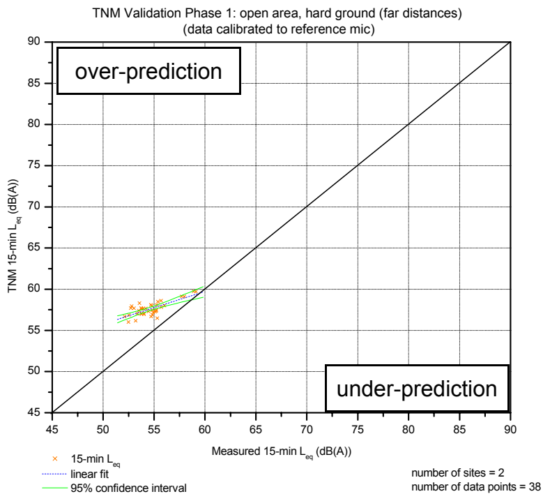
Figure G.5. Direct Comparison of TNM and Measured Data; Open Area, Hard Ground Sites; Separated High and Low Sound Levels; Strong Wind Data Removed.
