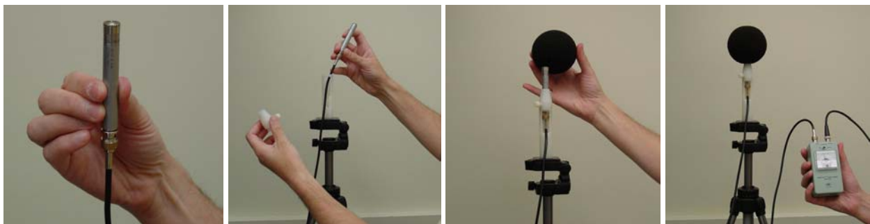
Figure 1. Microphone System.
