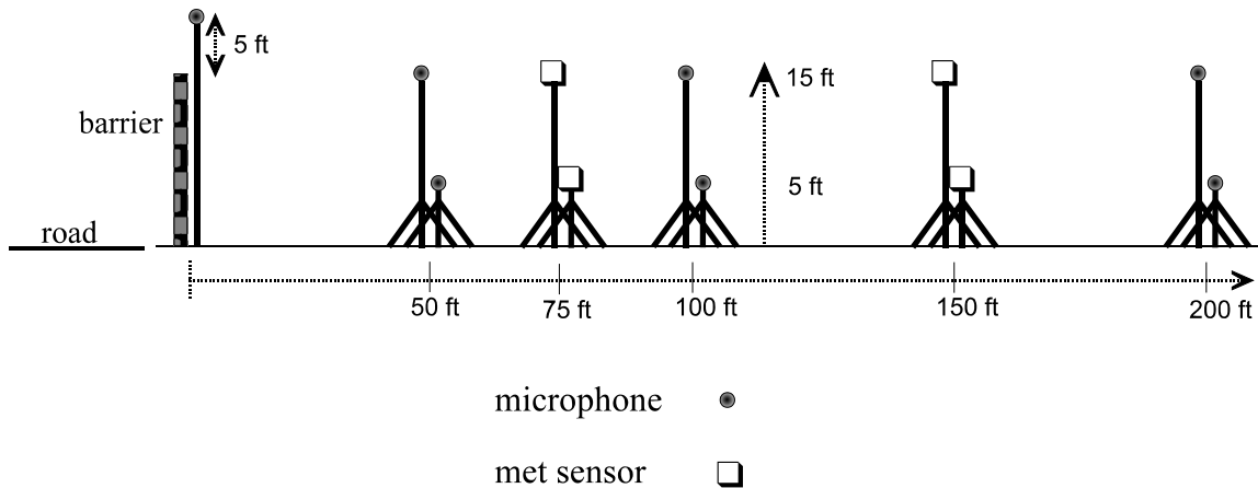
Figure 9. Example Instrumentation Setup for Barrier Site; Profile.
