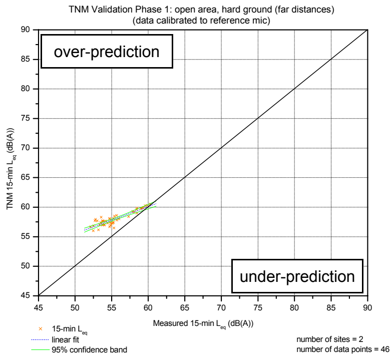
Figure F.5. Direct Comparison of TNM and Measured Data; Open Area, Hard Ground Sites; Separated High and Low Sound Levels; All Wind Data Included.
