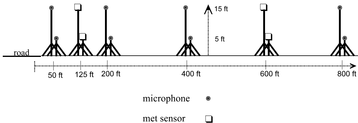
Figure 8. Example Instrumentation Setup for Open Area Site; Profile.
