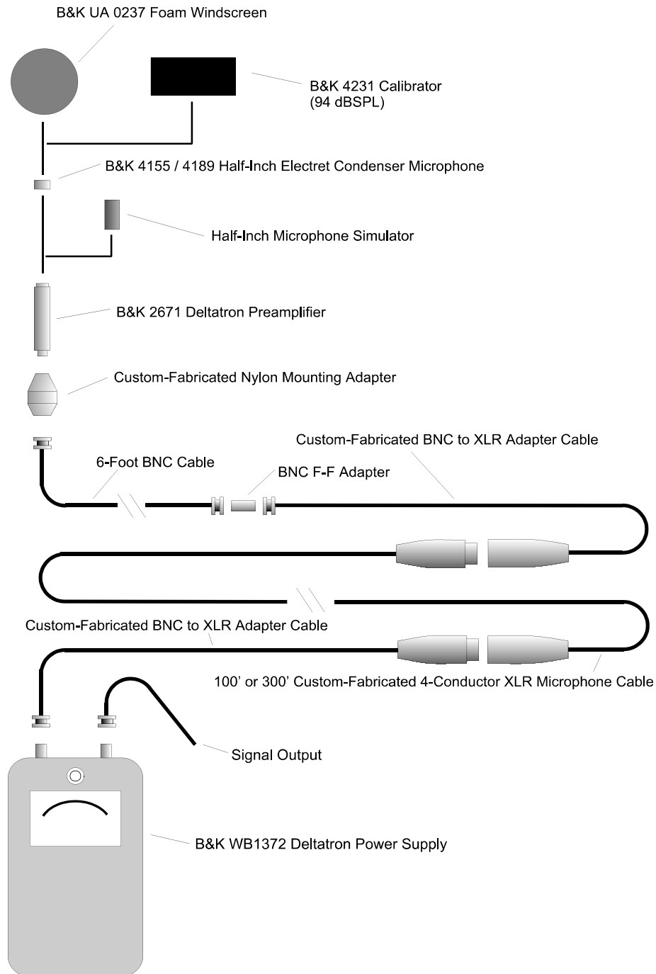
Figure C.3. B&K Deltatron Microphone System
