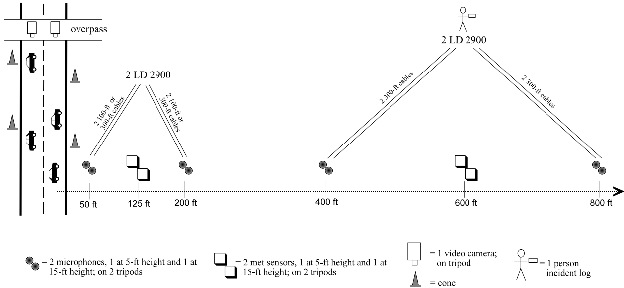
Figure 7. Example Instrumentation Setup for Open Area Site; Plan View.
