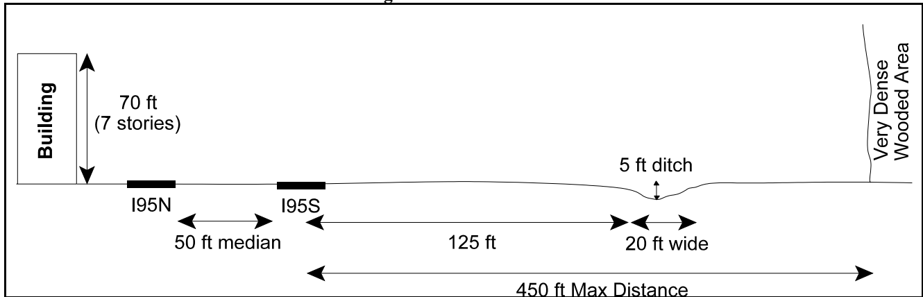
Site Diagram - Cross Sectional View
