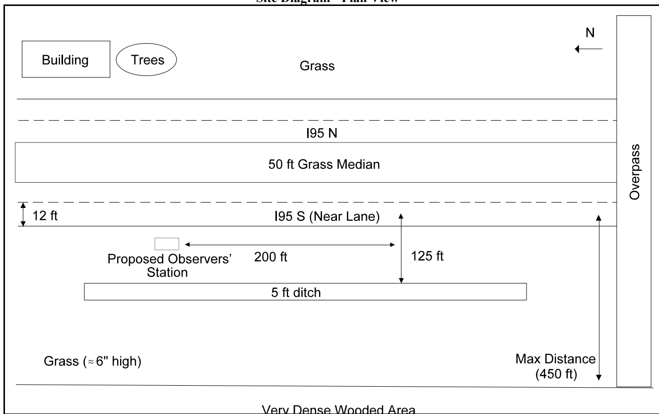
Site Diagram - Plan View *
