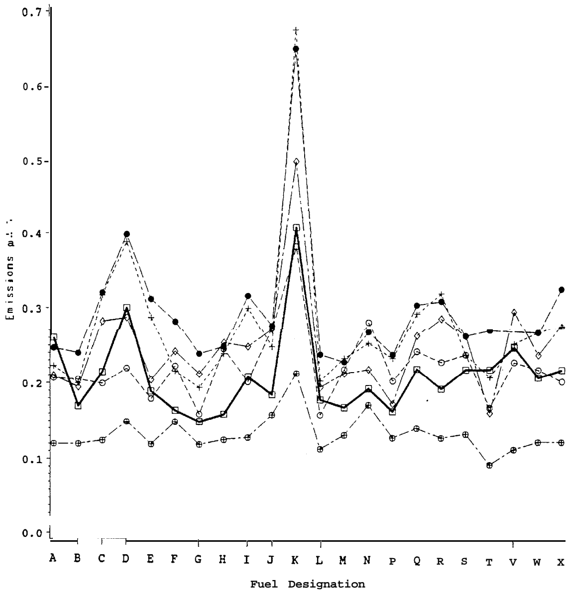
Figure 3 Emissions Test Data - HC
