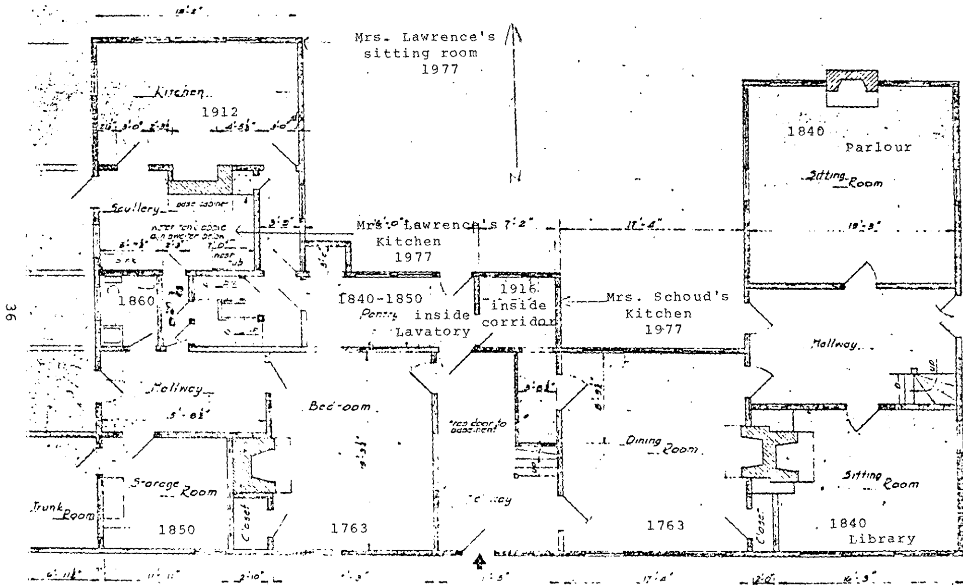
ARCHITECT MADE Sketch of first floor layout scale 1/4" = 1'-0"
