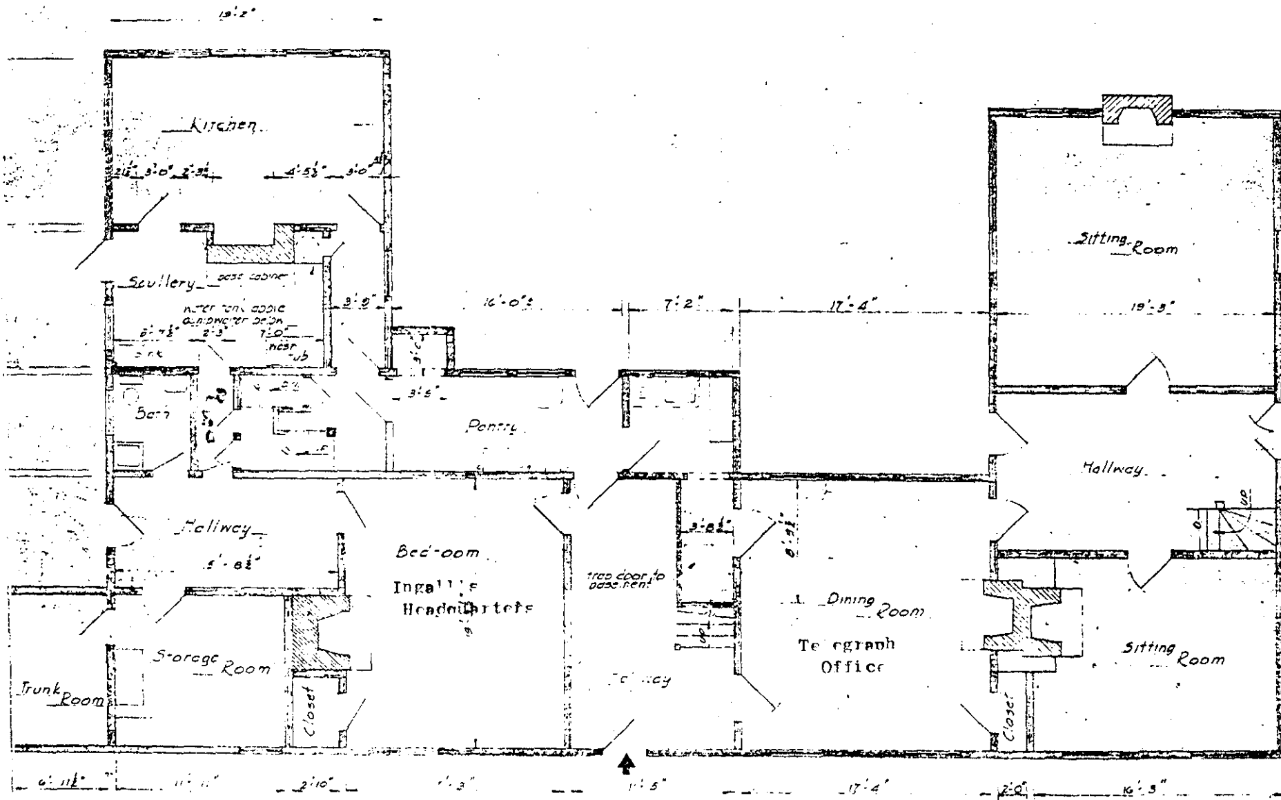
APROMATTOX MANOR Sketch of first floor Layout scale 1/2" = 1'-0"
