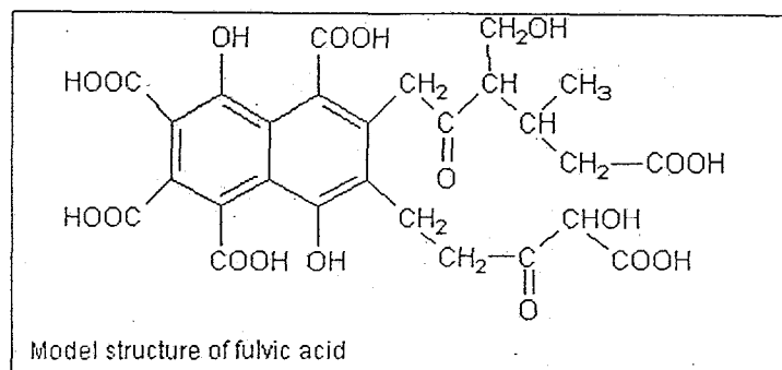
Figure 3: Model structure of fulvic acid [6].
