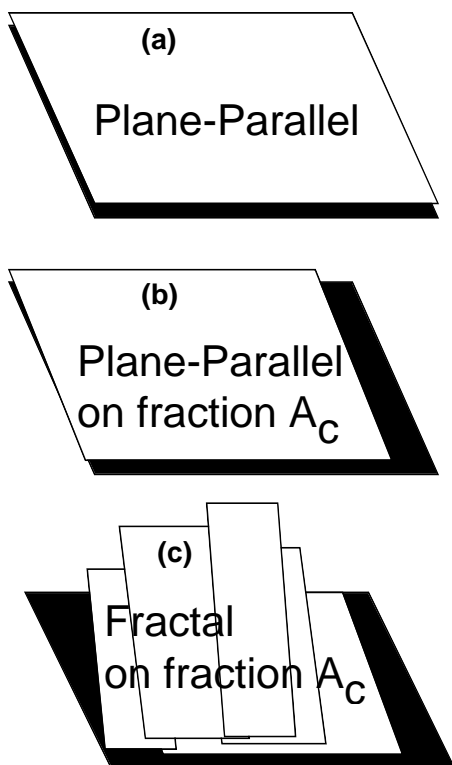
Fig. 1. Schematic showing three approaches to distributing the cloud liquid water in a GCM gridbox. In the top figure, the cloud has plane-parallel geometry, with cloud parameters such as vertical optical thickness, \tau_v , uniform over the whole gridbox. In the middle figure, the parameters are uniform over a fraction A_c of the gridbox, with the same values as above, except that cloud vertical optical thickness increases to \tau_v/A_c , thus preserving the total liquid, while the cloud thickness is zero on the remaining fraction 1 - A_c . In the bottom figure one has a fractal distribution of cloud parameters over the fraction A_c , with the same mean values as in the middle, and an identical clear fraction 1 - A_c .
