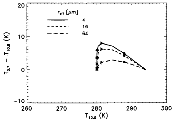
Figure 3. Dependence of water droplet cloud brightness temperature differences on effective radius of cloud particle distribution. For a cloud layer mean temperature of 280 K, results are shown for BTD^{34} ( T(3.7 \mu\text{m}) - T(10.8 \mu\text{m}) ) versus T(10.8 \mu\text{m}) . On the theoretical curves, 10.8- \mu\text{m} optical depths of 0.5, 2, 4, and 6 are represented by a circle, triangle, square, and asterisk, respectively.
