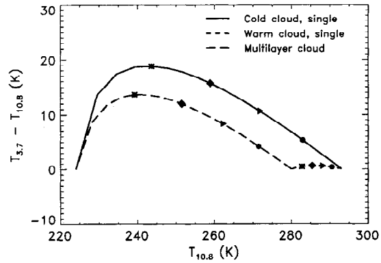
Figure 2. Dependence of BTD^{34} ( T(3.7 \mu m) - T(10.8 \mu m) ) on effective cloud amount \epsilon A_c as a function of the 10.8- \mu m brightness temperature due to the nonlinearity of the Planck radiance with temperature. Calculations are performed for no atmosphere and the cloud emittances are assumed to be the same at 3.7 and 10.8 \mu m . Curves are shown for a single-layered warm cloud (280 K), a single-layered cold cloud (224 K), and for overlapping cloud layers. On the theoretical curves, effective emittance ( \epsilon A_c ) values of 0.2, 0.4, 0.6, and 0.8 are represented by a circle, triangle, square, and asterisk, respectively.
