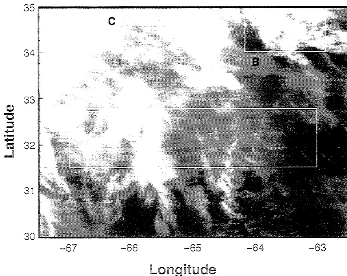
Figure 9. Multilevel cloud scene derived from AVHRR 1.1-km multispectral radiometric data on April 16, 1989, at 0606 UTC.
