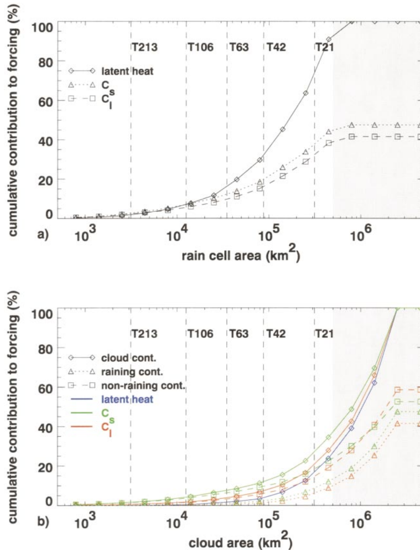
FIG. 6. (a) Cumulative contribution of rain cells to total latent heating (solid), C_l (dashed line) and C_s (dotted) as a function of rain cell area. (b) Same for clouds. Blue is latent heating, green is C_s , and red is C_l . Solid lines are the contributions from the entire cloud, dotted lines are the contributions from the precipitating portions of cloud, and dashed lines are the contributions from nonprecipitating portions of cloud.
