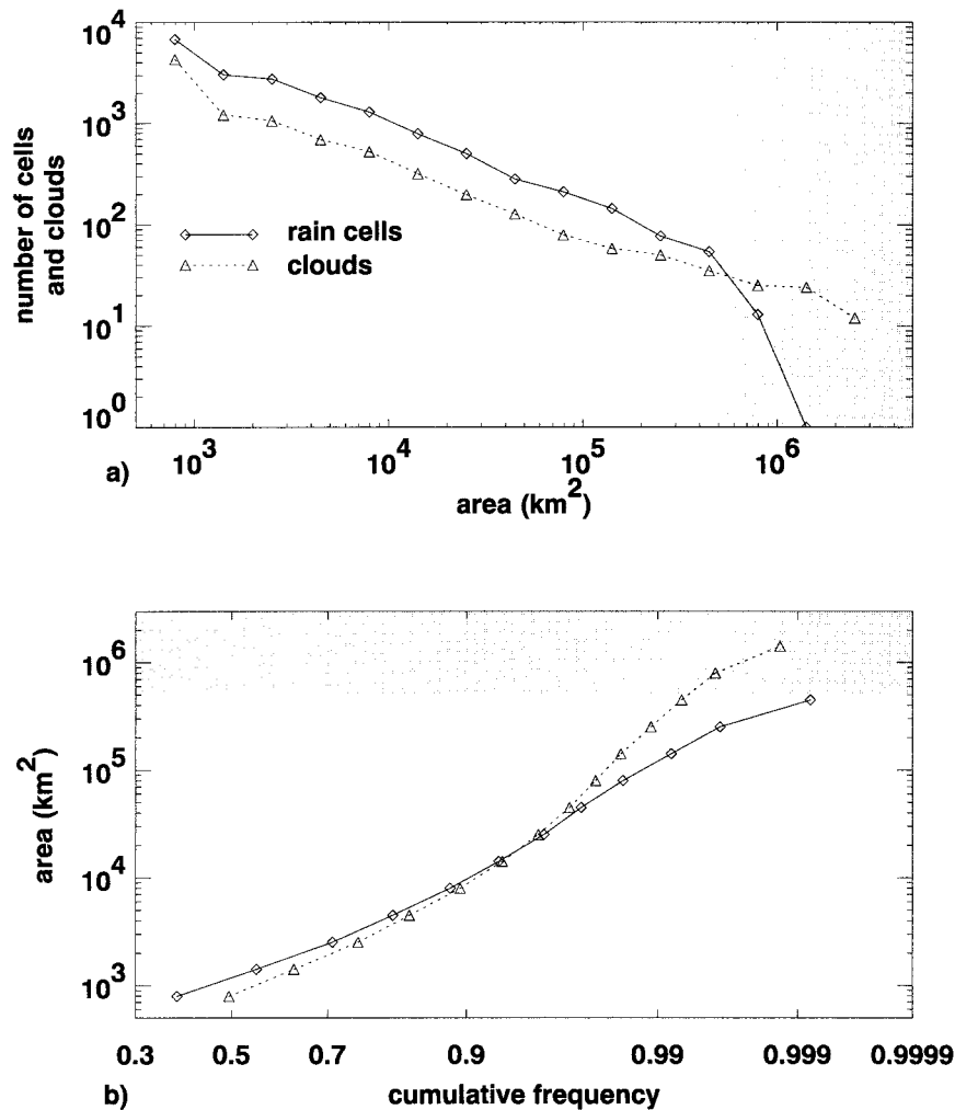
FIG. 2. (a) Number of rain cells (solid line) and clouds (dotted) as a function of area. (b) Cumulative frequency of occurrence of rain cells and clouds as a function of area. Cumulative frequency (abscissa) is shown on a normal probability scale.
