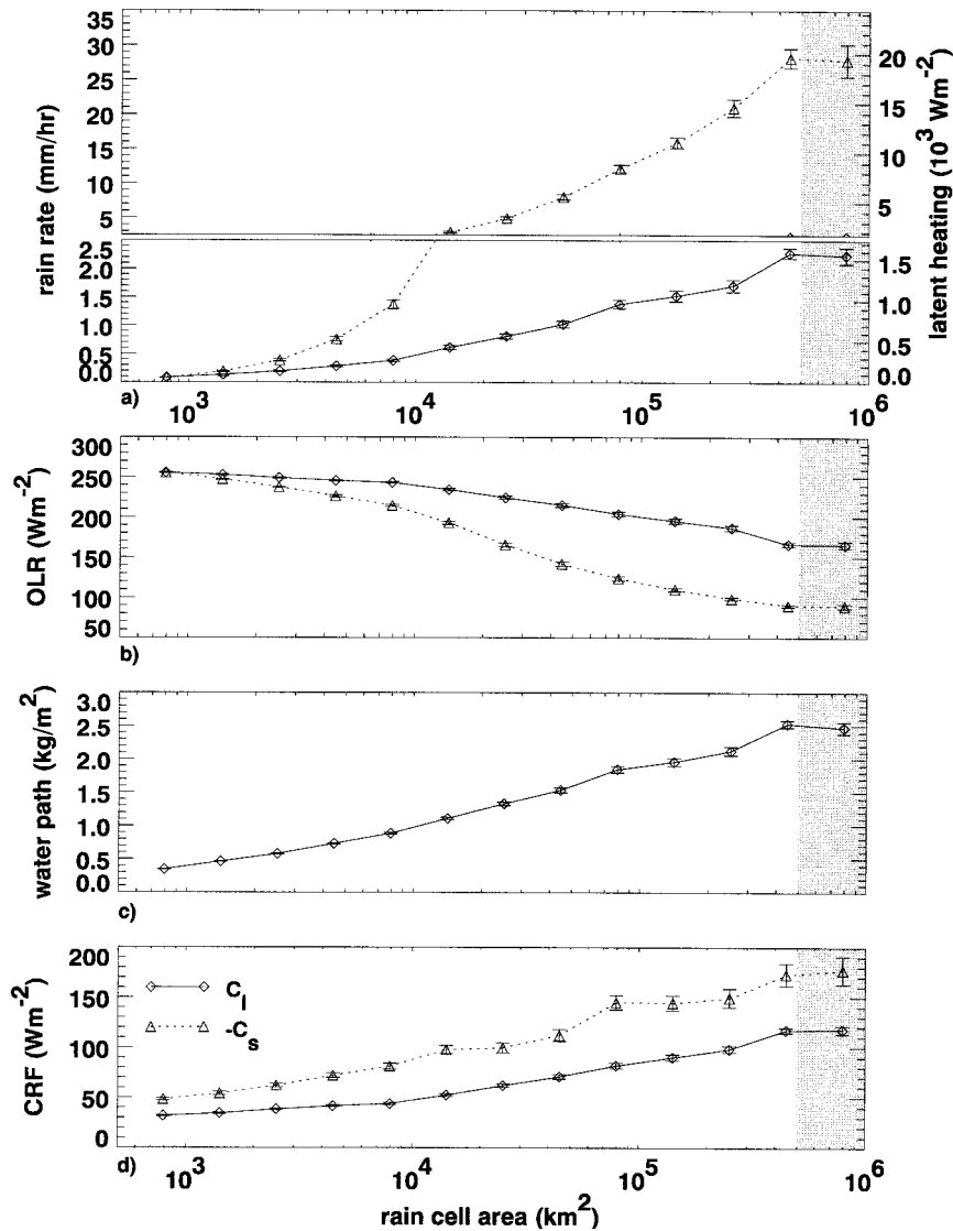
FIG. 4. Rain-cell-averaged properties as a function of rain cell area. (a) Rain rate (solid line) and 0.25^\circ peak rain rate (dotted). Right-side axis scaled to show vertically integrated latent heating. (b) OLR (solid) and 0.25^\circ minimum OLR (dotted); (c) Ice + liquid water path; (d) C_l (solid) and -C_s (dotted). Error bars indicate one standard deviation of the mean.
