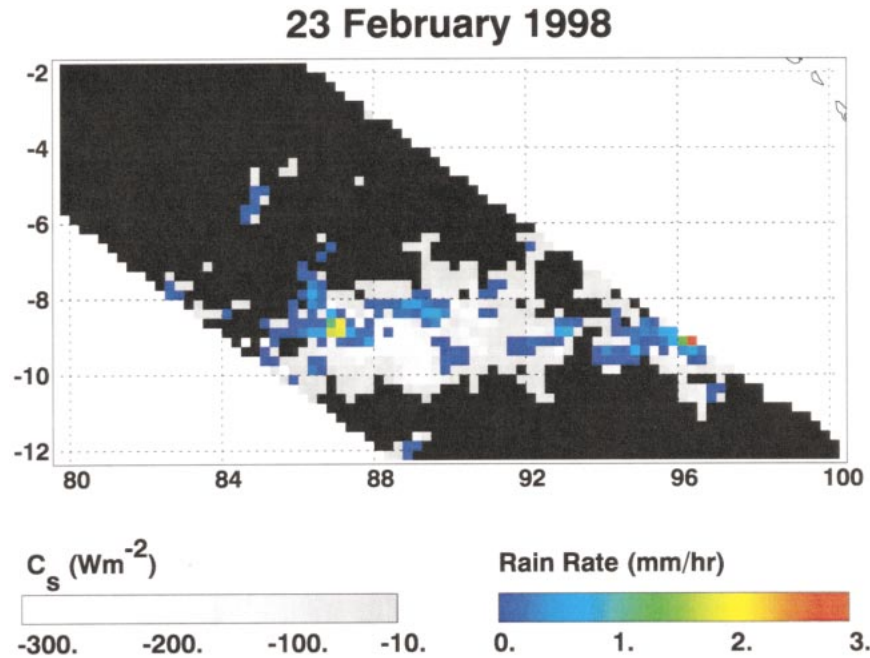
FIG. 1. Clouds and rain cells detected by TRMM over the tropical Indian Ocean on 23 Feb 1998. Grid boxes where C_s is less than -10 W m^{-2} are shown in gray. Contiguous regions of such grid boxes are clustered into individual clouds. One large cloud is shown in the center of the swath with several smaller clouds surrounding it. Overlaid in color is surface rain rate. Contiguous regions of nonzero rain rate are clustered into rain cells. Rain cells always exist within a cloud. Several rain cells of varying size exist within the large cloud shown. Some of the surrounding clouds contain rain cells and others do not.
