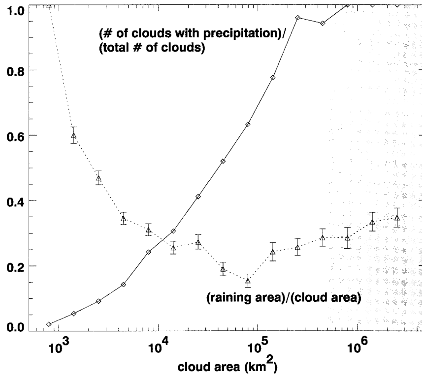
FIG. 3. Fraction of clouds that contain a rain cell (solid line). Also, the average fraction of cloud area taken up by rain cells (dotted), for clouds that contain at least one rain cell only. Both shown as a function of cloud area. Error bars indicate one standard deviation of the mean.
