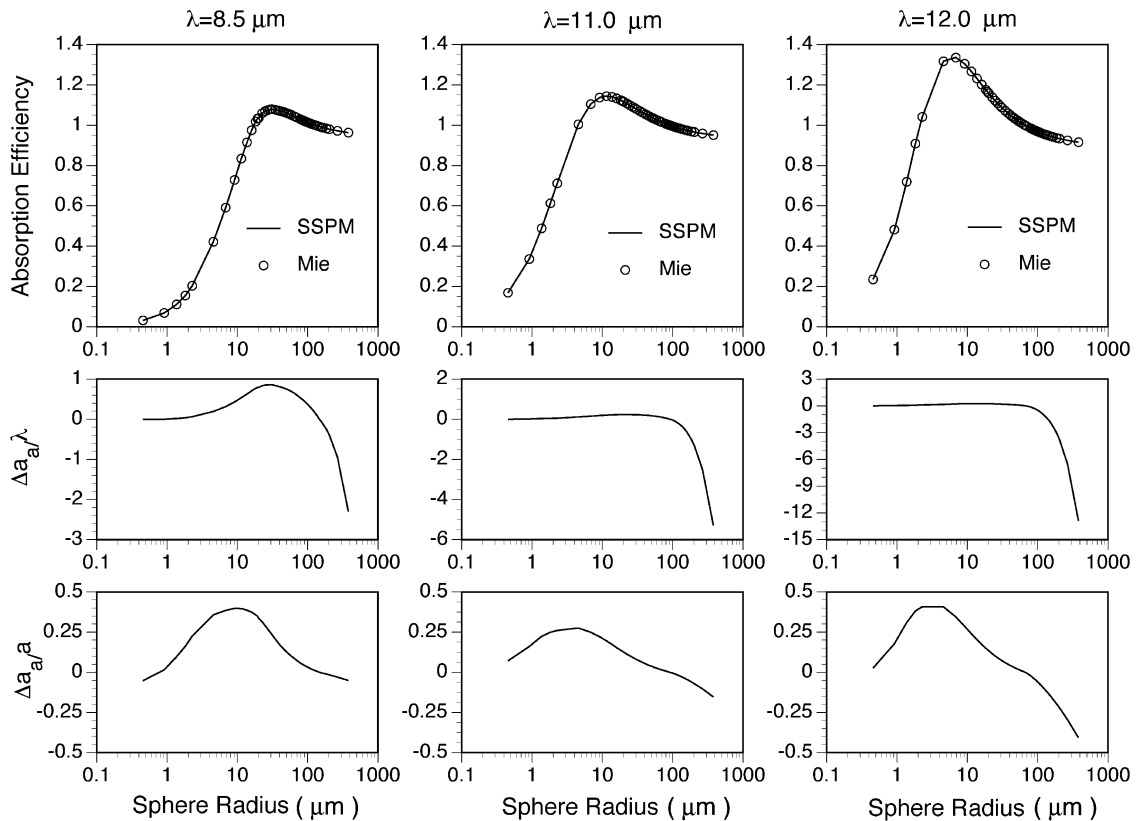
Fig. 8. The same as Fig. 7 except for absorption efficiency. A pronounced tunneling effect is evident at the 12.0 \mu\text{m} wavelength, as the absorption efficiency is substantially larger than unity at particle radii near 10 \mu\text{m} .
