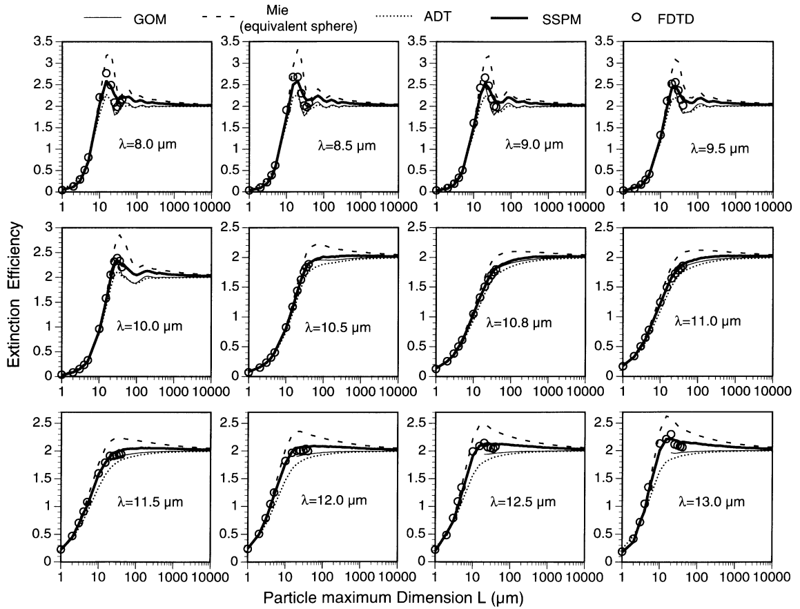
Fig. 11. The same as Fig. 10 except for extinction efficiency.
