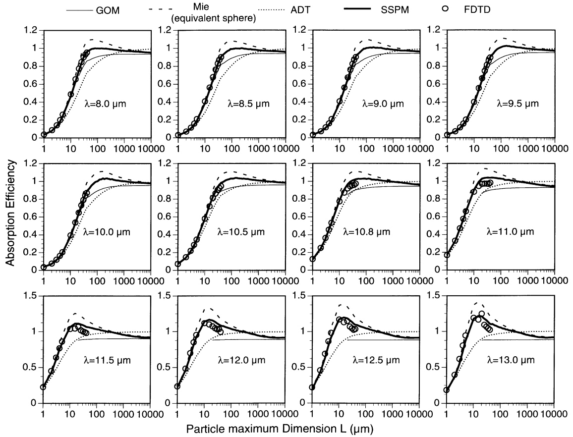
Fig. 10. The absorption efficiency of hexagonal ice crystals computed from various methods. The particle sizes are defined by their maximum dimensions with an implicit inclusion of aspect ratio defined in Eq. (1). The expansion parameter \Delta a_e and \Delta a_a required for SSPM calculation in the hexagonal case are approximated by their counterparts in a spherical case, that is, the number of layers of stretched potential and their thickness in hexagonal case is the same as in the spherical case.
