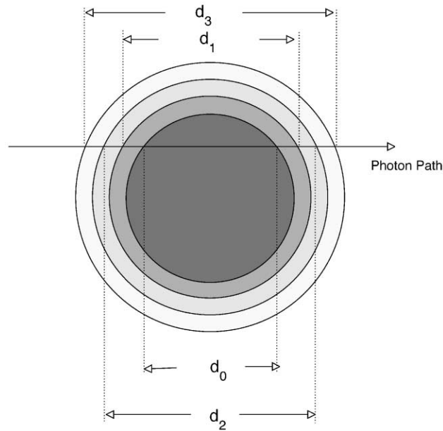
Fig. 6. Conceptual diagram illustrating the computational scheme for a multi-layered particle in the frame of an eikonal-type approximate method. Rectilinear projectiles are assumed for the photon paths in conjunction with the computation of phase delay and wave attenuation.
