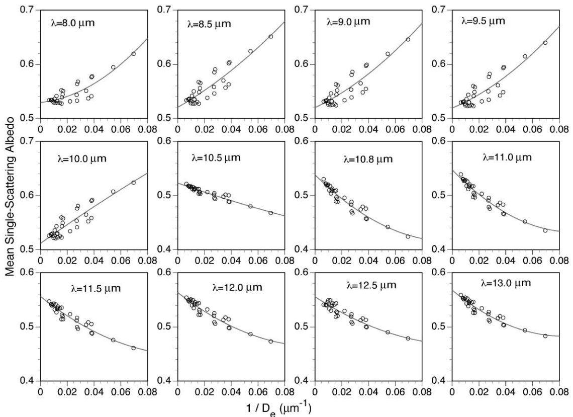
Fig. 16. The same as Fig. 15 except for mean single-scattering albedo. An increasing trend is evident for the variation of the single-scattering albedo versus 1/D_e at wavelengths 8.0, 8.5, 9.0, 9.5 and 10.0 \mu\text{m} . A decreasing trend is noted for the other wavelengths.
