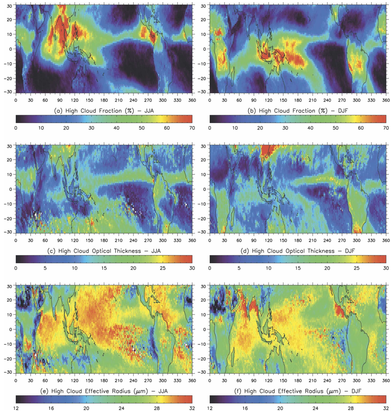
FIG. 8. The seasonal distributions of high cloud: (a), (b) fraction; (c), (d) optical thickness; and (e), (f) effective radius for the Northern Hemisphere (left) summer and (right) winter seasons derived from the 3-yr Terra and Aqua data over the Tropics (30°S–30°N).
