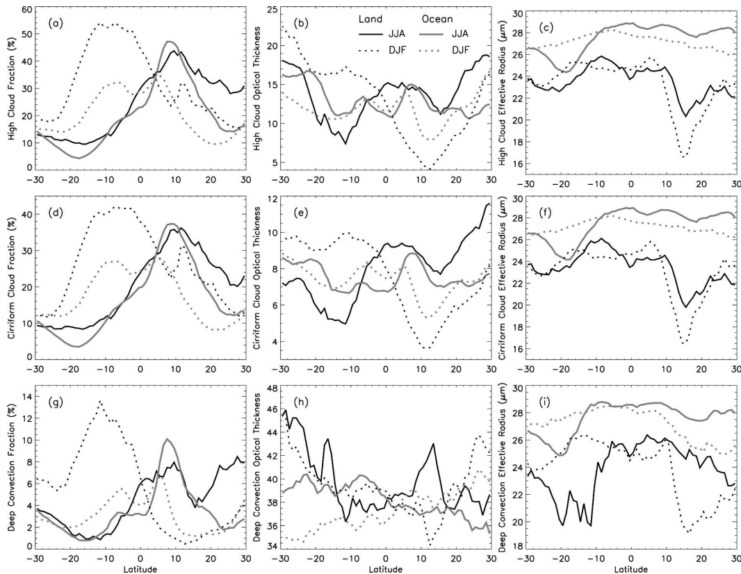
FIG. 10. The zonal mean cloud properties: (a), (d), and (g) cloud fraction; (b), (e), and (h) optical thickness; and (c), (f), and (i) effective radius for tropical (top) high cloud, (middle) cirriform, and (bottom) deep convective clouds over land and ocean along latitudes in summer (JJA) and winter (DJF).
