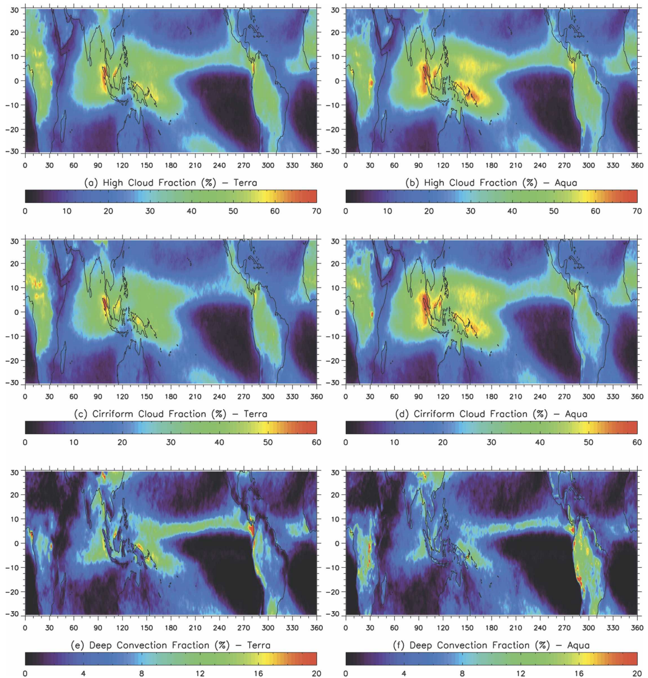
FIG. 5. Geographical distributions of the 3-yr mean fractions of: (a), (b) high cloud; (c), (d) cirriform cloud; and (e), (f) deep convective cloud from (left) Terra and (right) Aqua over the Tropics (30°S–30°N).
