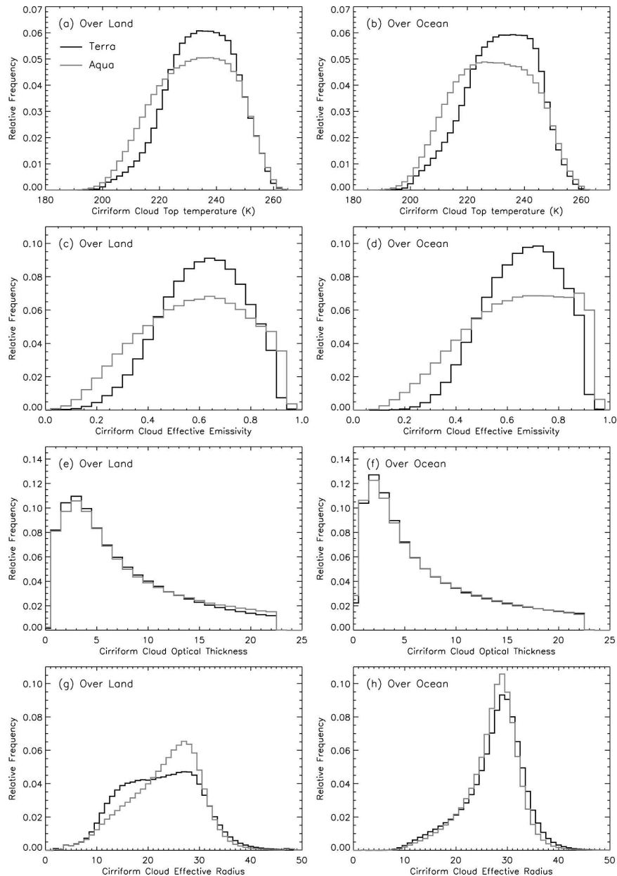
FIG. 2. Same as in Fig. 1, but for cirriform clouds.
