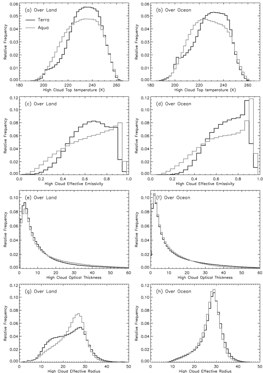
FIG. 1. Frequency distributions of: (a),(b) cloud-top temperature; (c),(d) effective emissivity; (e),(f) optical thickness; and (g),(h) effective radius for high clouds over (left) land and (right) ocean in the Tropics ( 30^{\circ}\text{S} – 30^{\circ}\text{N} ) from Terra (descending orbit with an equatorial crossing at 1030 LST) and Aqua (ascending orbit with an equatorial crossing at 1330 LST).
