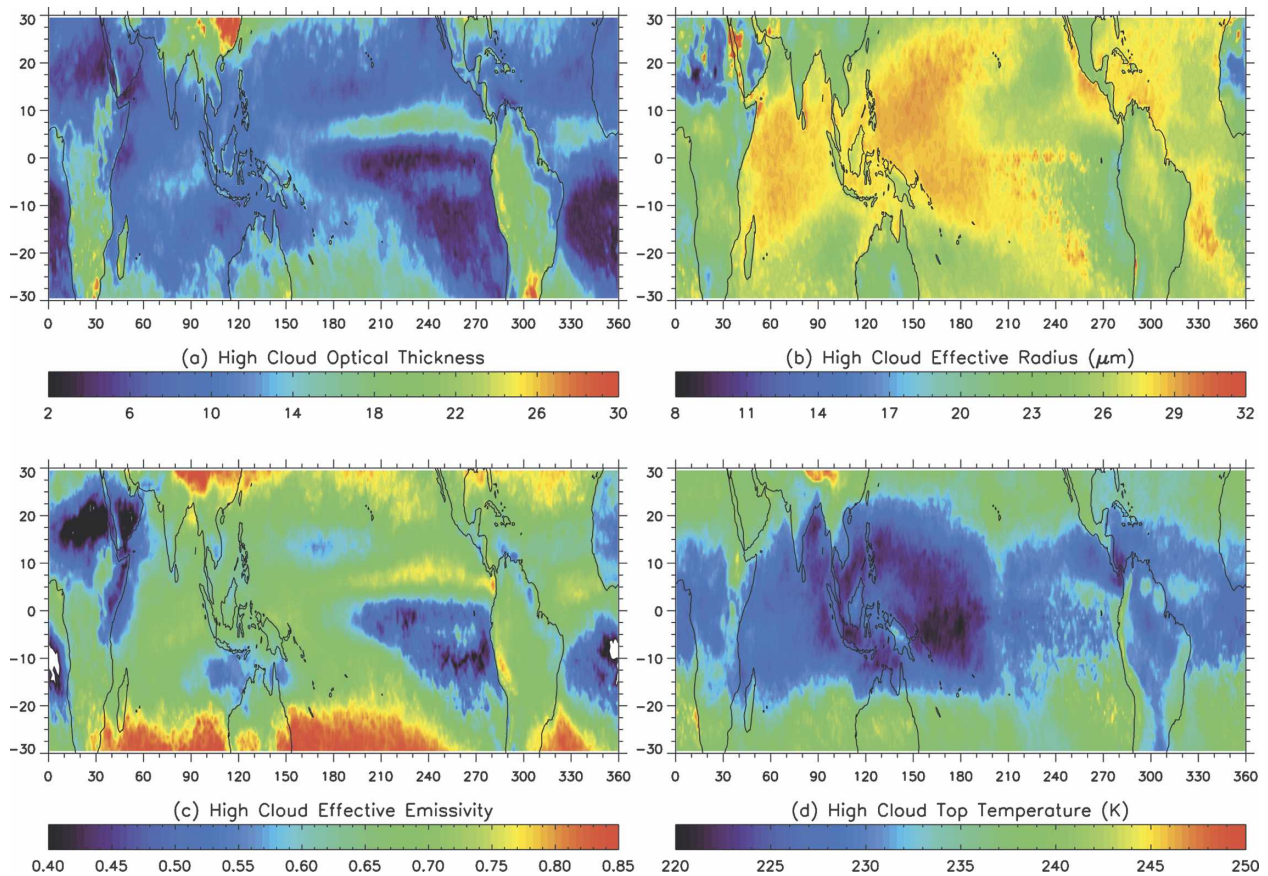
FIG. 7. Same as in Fig. 6, but for Aqua .
