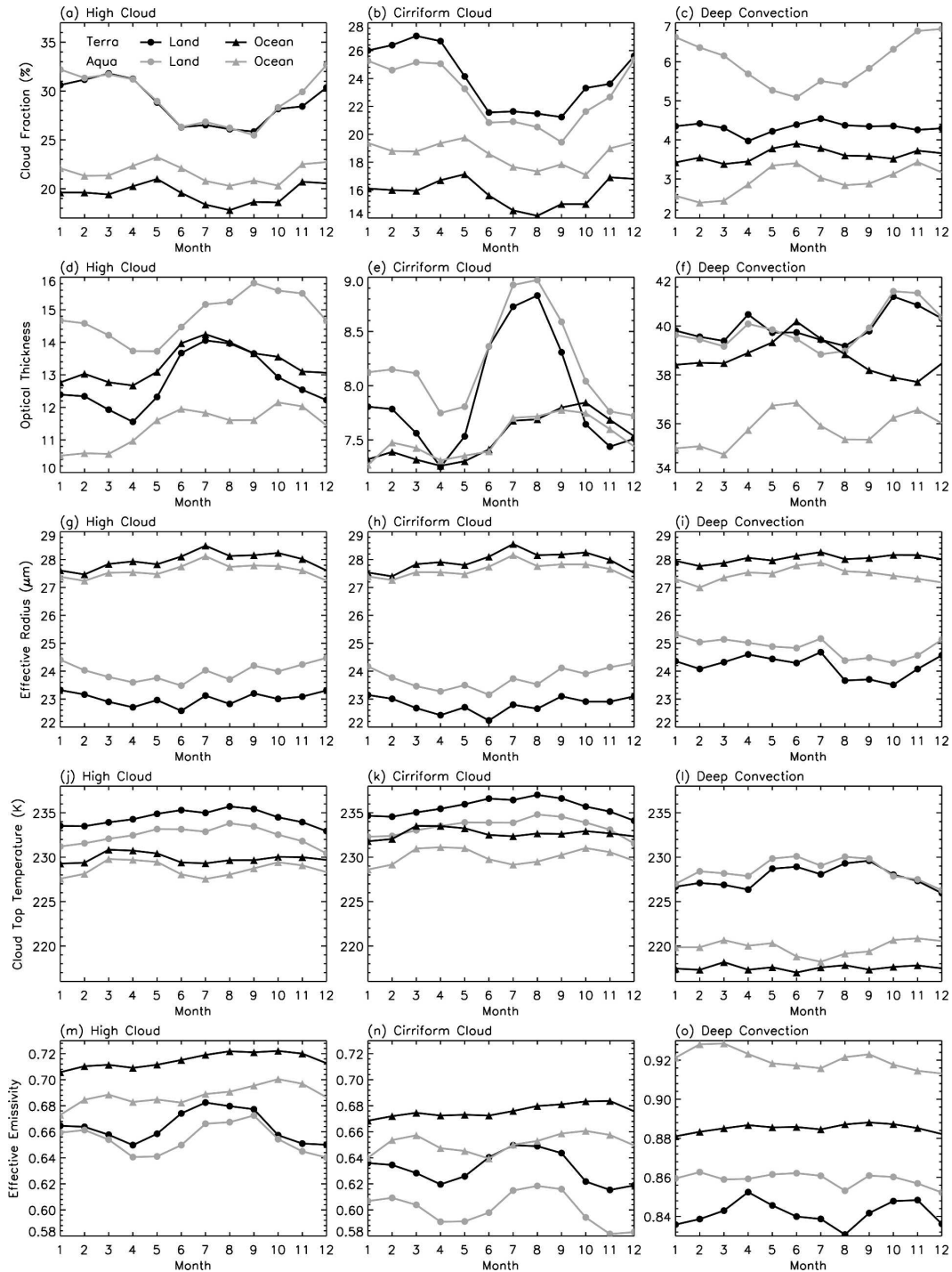
FIG. 9. Monthly means of (a)–(c) cloud fraction, (d)–(f) optical thickness, (g)–(i) effective radius, (j)–(l) cloud-top temperature, and (m)–(o) effective emissivity for (left) high cloud, (middle) cirriform, and (right) deep convective clouds from Terra and Aqua over the tropical land and ocean (30°S–30°N).
