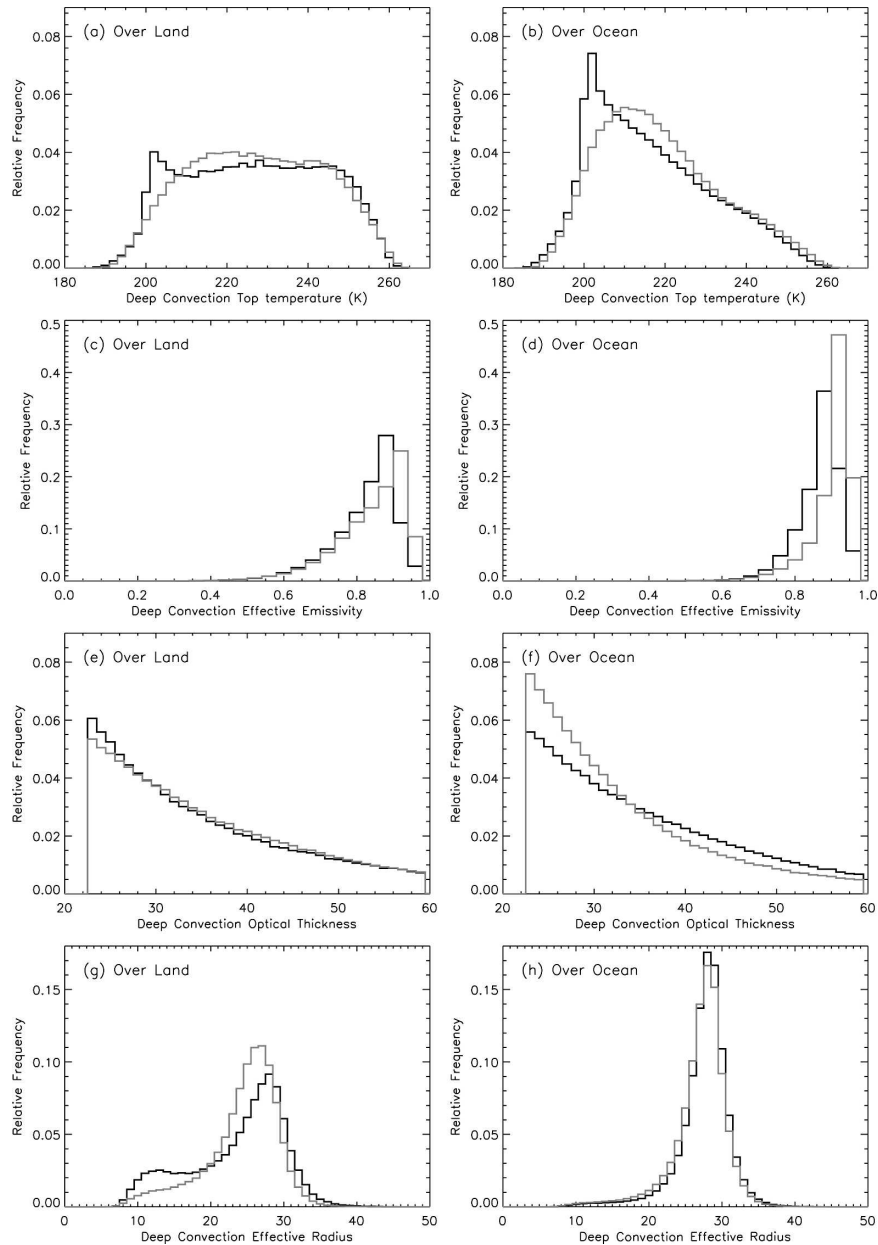
FIG. 3. Same as in Fig. 1, but for deep convective clouds.
