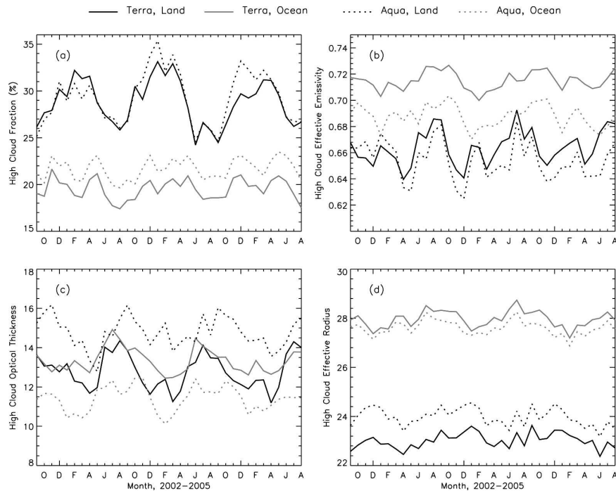
FIG. 4. Monthly means of (a) high cloud fraction, (b) effective emissivity, (c) optical thickness, and (d) effective radius averaged over the Tropics ( 30^{\circ}\text{S} – 30^{\circ}\text{N} ) from Terra and Aqua .
