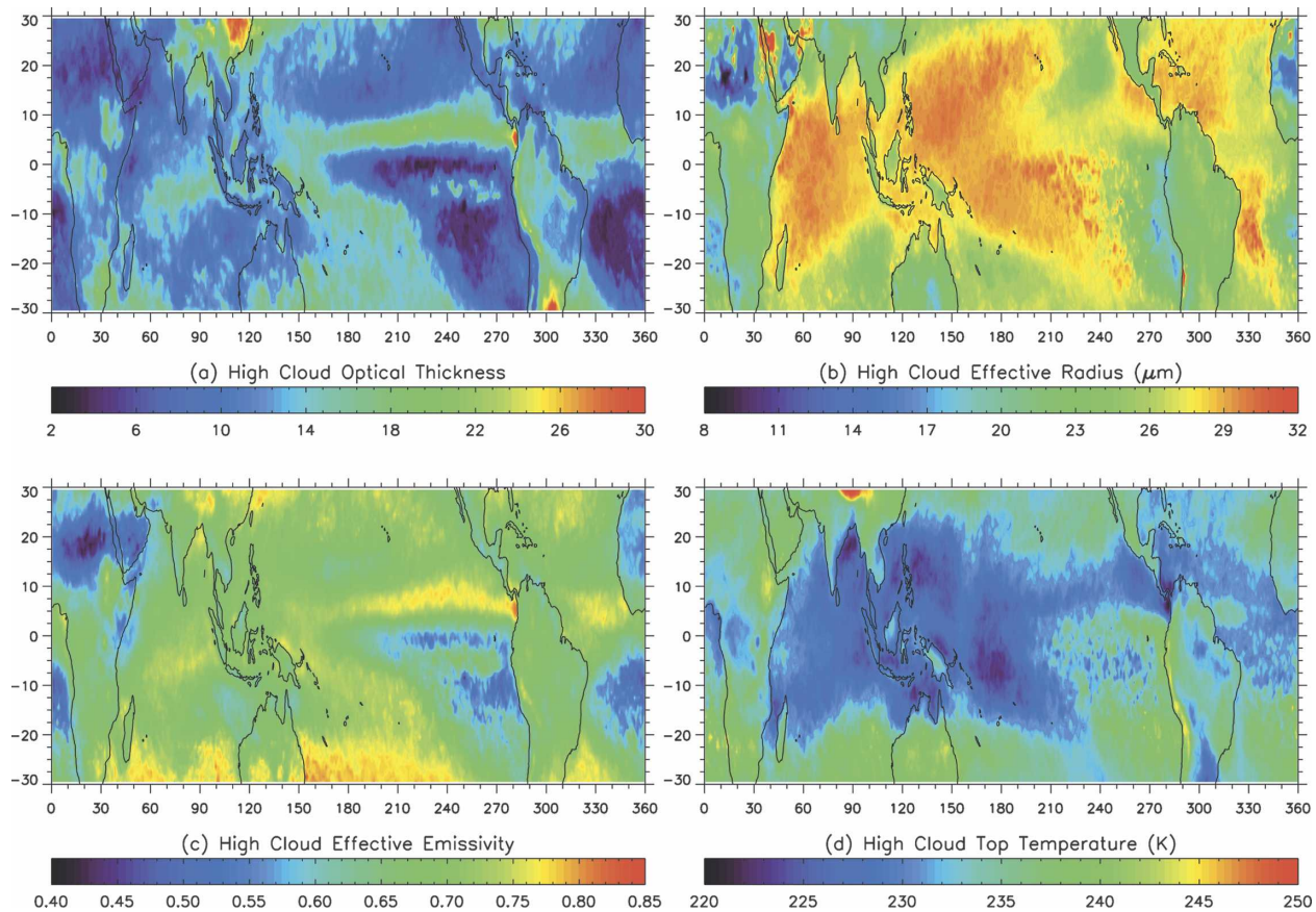
FIG. 6. The geographical distributions of 3-yr means of high cloud (a) optical thickness, (b) effective radius, (c) effective emissivity, and (d) cloud-top temperature from Terra over the Tropics (30°S–30°N).
