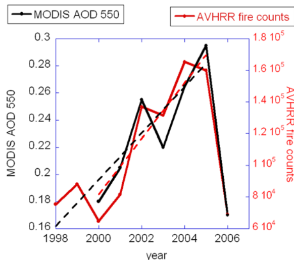
Figure 4. Mean MODIS aerosol optical depth at 550 nm (left axis, black) and total AVHRR fire counts (right axis, red) for the entire domain and biomass burning season of August through November plotted as a function of year. Also plotted are the linear trend lines through the time series with 2006 omitted (dashed lines). The subsetted time series with 2006 omitted results in significant trend correlations of R = 0.90 for both variables, while the full time series including 2006 results in insignificant trend correlations of R = 0.27 for the AOD and R = 0.50 for the fire counts.
