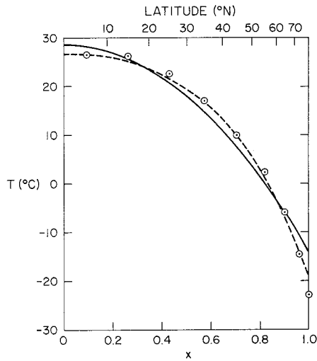
Fig. 5. Mean annual northern hemisphere zonally averaged temperature (degrees Celsius) versus sine of latitude for the two-mode approximation to the diffusive model (solid curve), the observations (circled dots), and a fit including P_4(x) (dashed curve) [from North, 1975b] (cf. (32)).
