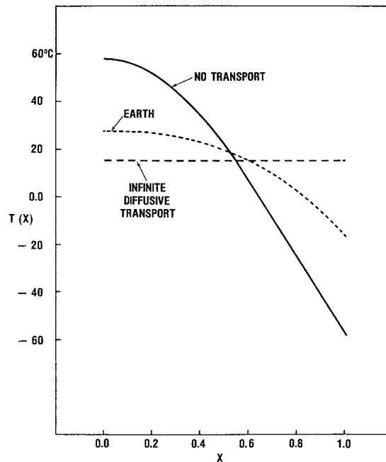
Fig. 4. Temperature (degrees Celsius) versus sine of latitude for the cases of no transport, infinite transport, and earth (schematic).
