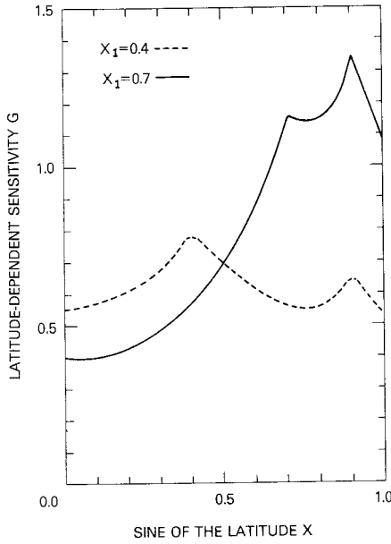
Fig. 20. Latitude-dependent sensitivity (i.e., stationary response function) G(x, x_1) computed with diffusive transport, Budyko's infrared rule, and an isothermal ice cap edge at x_0 = 0.9 . The two cases shown are for perturbations at 23.5^\circ latitude ( x_1 = 0.4 ) and at 45^\circ latitude ( x_1 = 0.7 ). In both cases, additional heat is absorbed in the ice edge region, and the effect increases with the global temperature sensitivity (here \beta_0 = 1.6^\circ\text{C} per 1% change in solar constant) as well as with the proximity of the perturbation to the ice edge.
