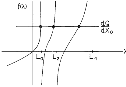
Fig. 18. Schematic graph of the right-hand side of (105) (denoted by f(\lambda) in the figure) versus the stability parameter \lambda . Intersections with the (flat) dQ/dx_0 graph indicate discrete eigenvalues \lambda^0 of the system. Note that if dQ/dx_0 is negative, the lowest eigenvalue must be negative, implying instability.
