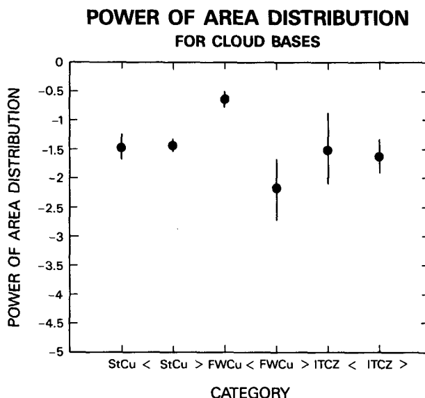
FIG. 4(a). Summary of cloud base area distributions. The slopes (referred to as 2B in the text), were determined as in Fig. 3 and averaged over all available scenes of a given cloud type, for the three cloud types described in the text. A value of the slope is obtained for smaller (<) and larger (>) areas for each cloud type. The vertical lines extend one standard deviation above and below the mean. Note that small and large clouds have significantly different slopes for both fair weather cumulus and ITCZ. Only stratocumulus are consistent with scale invariance.
