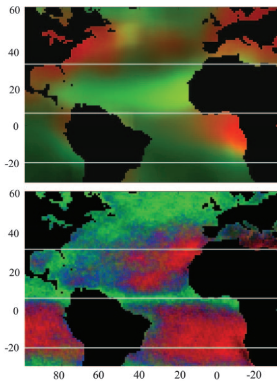
Fig. 1. Spatial distribution of aerosol and clouds over the Atlantic Ocean from Moderate Resolution Imaging Spectroradiometer (MODIS) data for June–August 2002. (Upper) Spatial distribution of the aerosol column concentration (expressed as the optical thickness) and type (given by the fraction of the aerosol in the sub- \mu\text{m} mode) over the Atlantic Ocean for the June–August period. The optical thickness is represented by the brightness of the image. The aerosol type is represented by the color: red, dominance by sub- \mu\text{m} particles, smoke from central Africa and pollution from Europe and North America, and green, dominance by dust from Africa or sea salt in regions with high winds. (Lower) Spatial distribution of shallow (red), deep convective (green), and mixed (blue) cloud cover on a 1^\circ \times 1^\circ longitude \times latitude grid. Black indicates continental regions. The data are averaged for June–August 2002.
