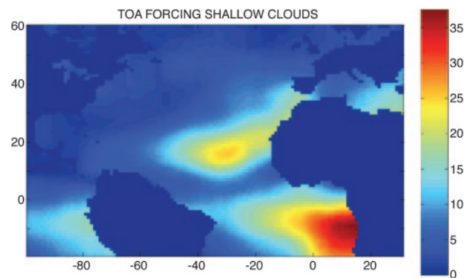
Fig. 3. The aerosol reflected solar flux at the top of the atmosphere due to combined effect on cloud cover and microphysics and on reflection of solar radiation. The radiative effect is calculated as the difference of MODIS observations from the conditions for baseline aerosol with optical thickness of 0.06. The results are weighted by the frequency of detection of shallow clouds in the 1^\circ latitude \times longitude daily grid boxes. The color bar shows the values in \text{W/m}^2 .
