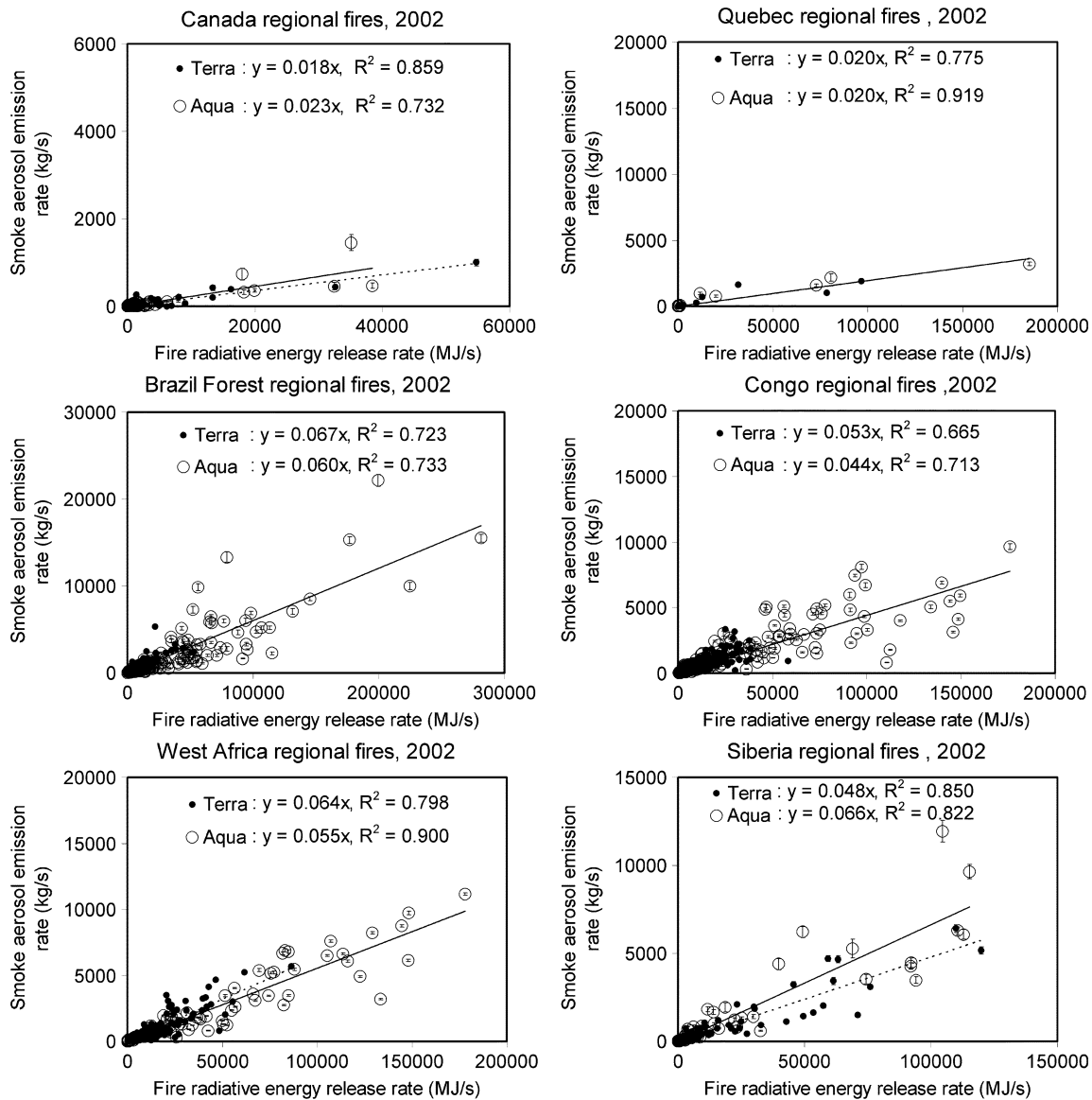
Fig. 2. Regional correlations between rates of emission of smoke aerosols R_{sa} (kilograms per second) and the rates of release of fire radiative energy R_{fire} (megajoules per second or megawatts) from fires detected by MODIS on (dots and dotted lines) Terra and (circles and solid lines) Aqua throughout the designated regions in 2002. Each data point represents one MODIS daytime overpass over the region. Vertical error bars represent the standard errors of R_{sa} .
