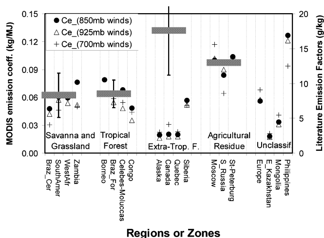
Fig. 7. FRE coefficients of emission ( C_e ) of smoke aerosol (scale on left vertical axis), derived with wind speeds at 850 mb (approximately 1.5-km altitude), are shown for various regions or zones alongside those derived with winds at 925 mb ( \sim 0.75 km) and 700 mb ( \sim 3 km). The different regions have been grouped according to the ecosystem categories of Andreae and Merlet [6], based on the dominant ecosystem type as visually determined from the land-cover map in Fig. 6. It was not obvious to determine the dominant ecosystem types for the last group designated as unclassified (Europe, E_Kazakhstan, Mongolia, and Philippines). Thick horizontal bars (scale on right vertical axis) represent the average literature values of traditionally derived emission factors (with associated error bars) for each of the ecosystem types [6].
