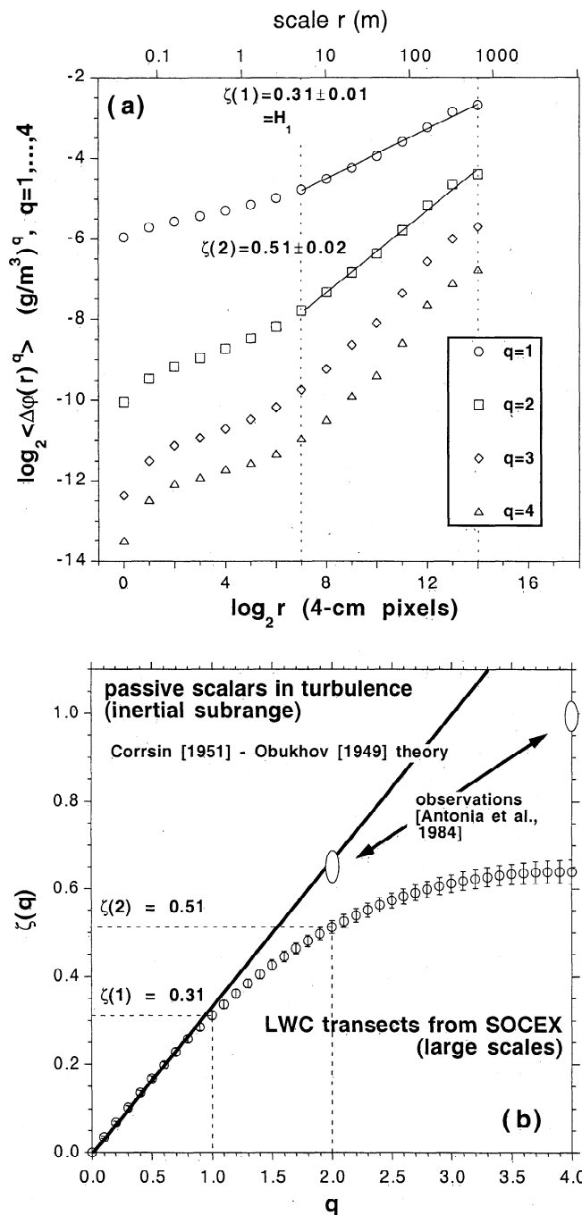
Figure 4. Ensemble-averaged structure functions. (a) Structure functions \langle \Delta\varphi(r)^q \rangle ( q = 1, \dots, 4 ) versus scale r on a log-log plot for the (37 segment) ensemble average; the range of scales used for the regressions is highlighted. Judging by the spectral data for segment 5 in Figure 1, we see that the actual scaling range goes far beyond the maximum scale sampled here, namely, L_6^*/2 \approx 0.6 km; a conservative estimate is 5–10 km. (b) Large-scale exponent function \zeta(q) obtained from 5 m to 0.6 km; two important exponents are emphasized at q = 1, 2 . The standard model for passive scalars in turbulence is indicated, \zeta(q) = q/3 , along with selected empirical results collected by Antonia et al. [1984].
